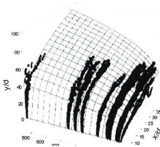
Figure 10. The Penn State correlation for penetration of trans- and super-critical fuel ( n -heptane and JP-8) jets in a low-speed cross-flow is represented by the surface in this 3-D plot. ( y/d=2.94J^{0.35}(x/d)^{0.33} ) Data points correspond to measured jet penetration profiles from several images.
