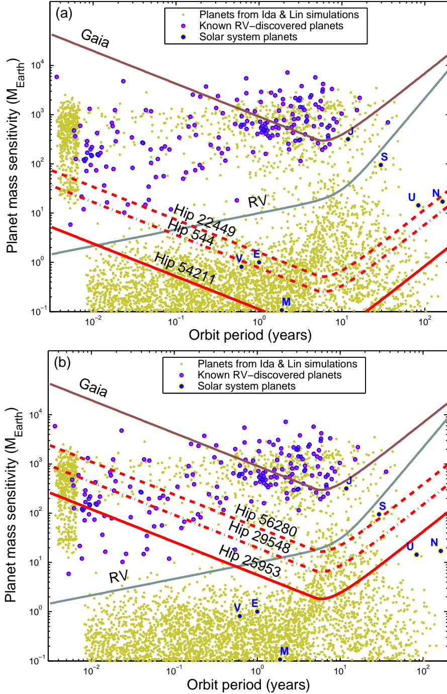
FIG. 1.— (a) Detailed view of the discovery space for rocky Earth-like ( \sim 1 - 10M_{\oplus} ) planets in the habitable zone ( \sim 0.7\text{-}1.5 AU for a G star), for the ‘Earth Analog Survey’ of 129 stars described in § 2. The small dots represent a theoretical planet distribution (Ida & Lin 2005) for planets of 0.1 - 3000M_{\oplus} . In this distribution gas giants have an envelope mass at least 10 times the mass of the central core; terrestrial planets initially formed within the ice line (2.7 AU for a solar luminosity star); icy planets formed outside the ice line; and hot Jupiters have periods \leq 0.1 AU. Exoplanets discovered as of early 2007 and with semimajor axes > 0.03 AU are shown as filled circles. Planets in our Solar System are labeled with single letters. Labeled curves represent the estimated sensitivity limits of indirect detection methods: for radial velocity method (RV at 1 \text{ m s}^{-1} ), and astrometry with SIM and Gaia. The SIM sensitivity in this space is a broad band, defined by the three lowest curves (labeled with specific Hipparcos star numbers). The lowest curve shows the ‘best’ star (as computed from star mass and distance); the middle curve represents the median star; and the upper curve shows the least favorable star in the sample. Also shown is the effective sensitivity of Gaia for stars at 50 pc, a typical distance for Gaia targets. (b) Detailed view of the discovery space for the SIM ‘Broad Survey’ of 2100 stars, in which a much larger sample of stars is surveyed with less sensitivity than in the ‘Earth Analog Survey’. Symbols and curves have the same meaning as in (a).
