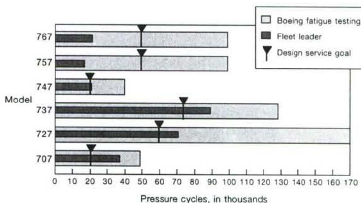
Figure 8. Boeing Full-Scale Fatigue Test
