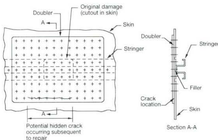
Figure 13. Typical Fuselage External Skin Repair
