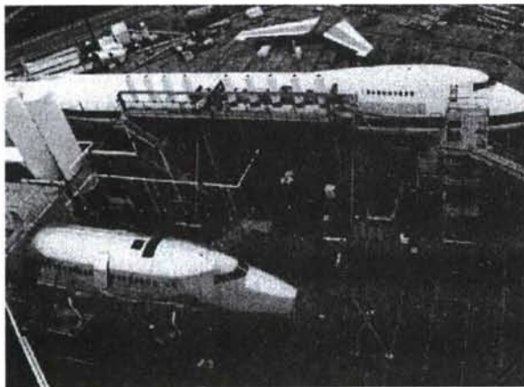
Figure 4. Cyclic Pressure Testing of 747 Fuselage Structures
