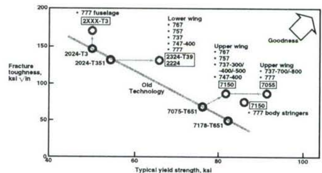
Figure 11. Boeing Structural Aluminum Alloy Improvements
