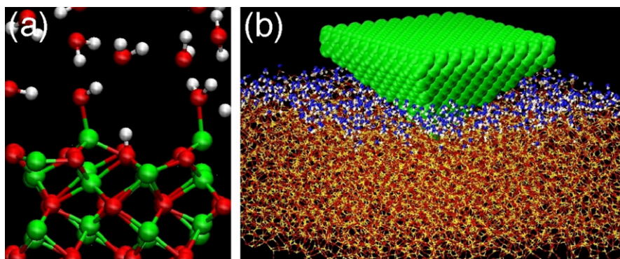
Fig. 9. (a) Close-up of EDC–DFT MD simulation of an \alpha - \text{Al}_2\text{O}_3 (0001) surface immersed in water. White, red, and green spheres represent hydrogen, oxygen, and aluminum atoms, respectively. (b) Indentation of amorphous silica covered with adsorbed water layer. White and yellow spheres are hydrogen and silicon atoms, whereas blue and red spheres are oxygen atoms originated from water and silica substrate, respectively. The indenter is shown in green.
