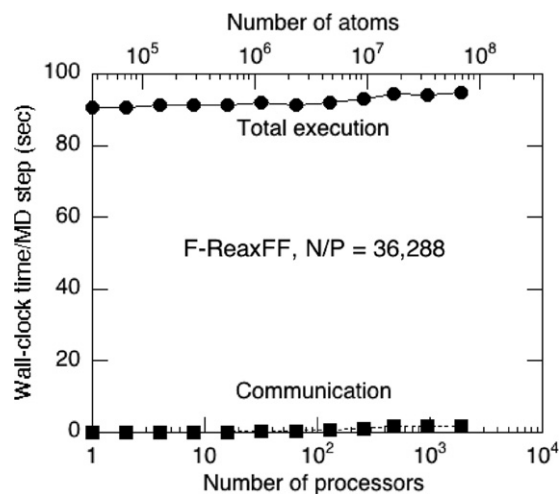
Fig. 5. Total execution (circles) and communication (squares) times per MD time step as a function of the number of processors for the F-ReaxFF MD algorithm with scaled workloads—36,288 P atom RDX systems on P processors ( P = 1, \dots, 1920 ) of Columbia.
