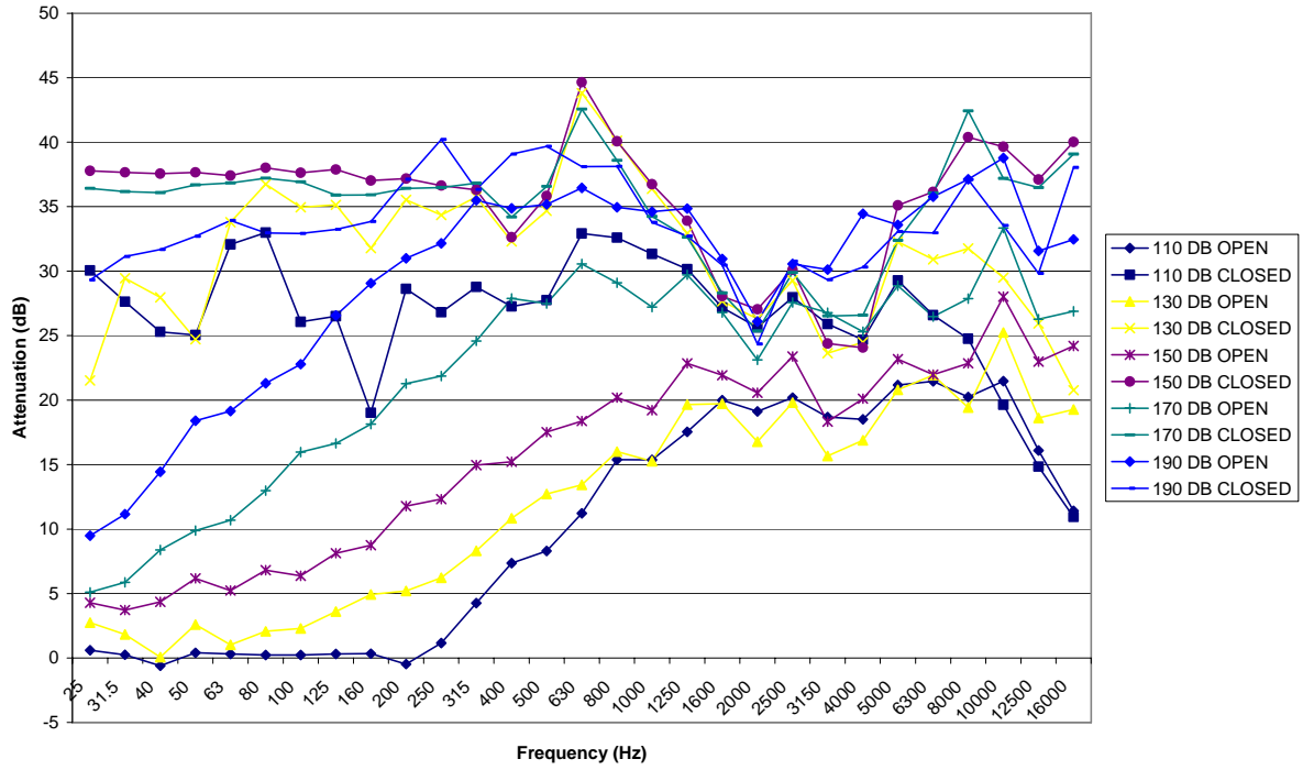
Figure 8: Attenuation measured with the AEARO prototype plugs, in the open and closed configurations.
