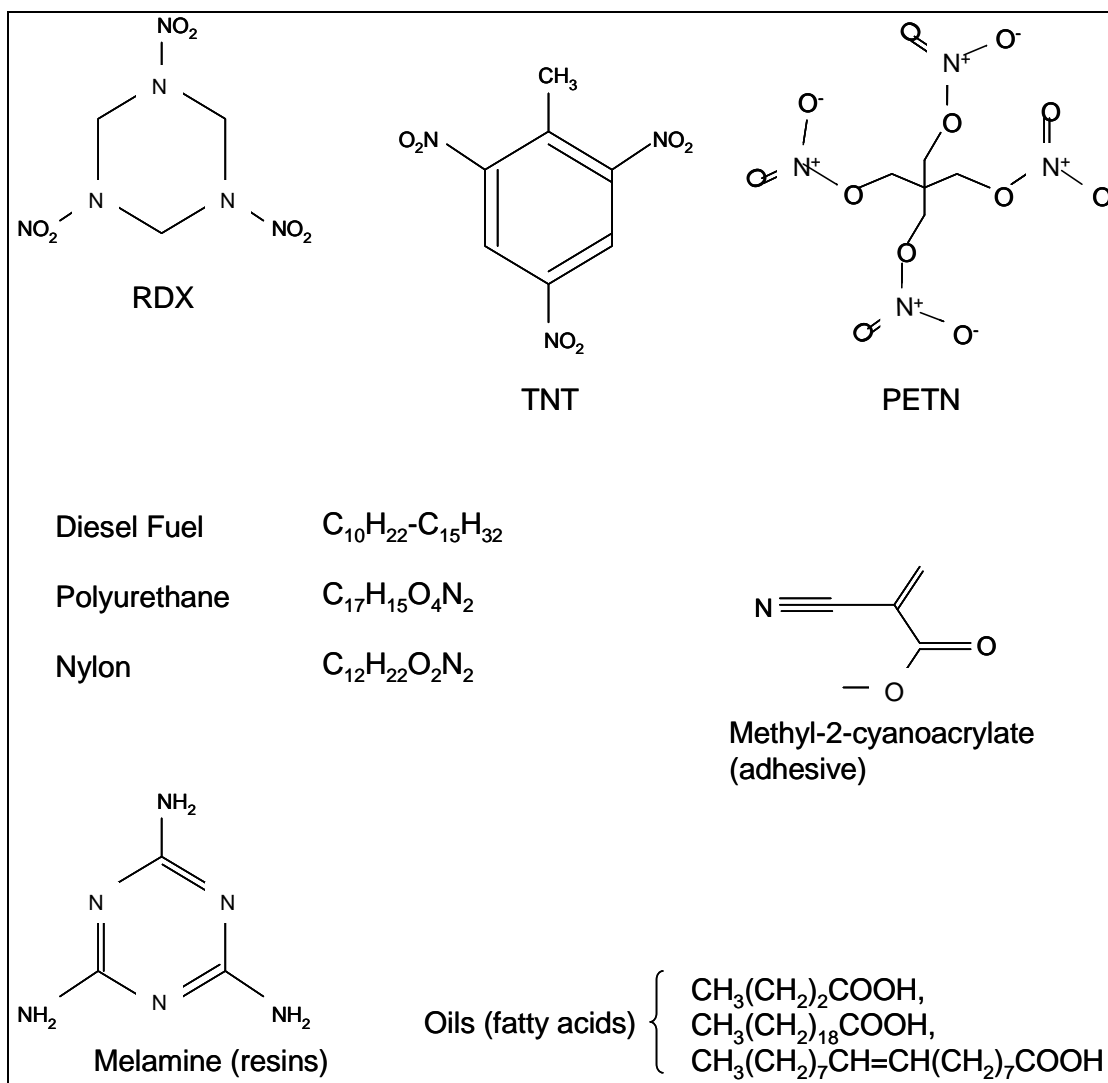
Figure 1. Structures or formulas of several explosives and non-energetic organic compounds.
