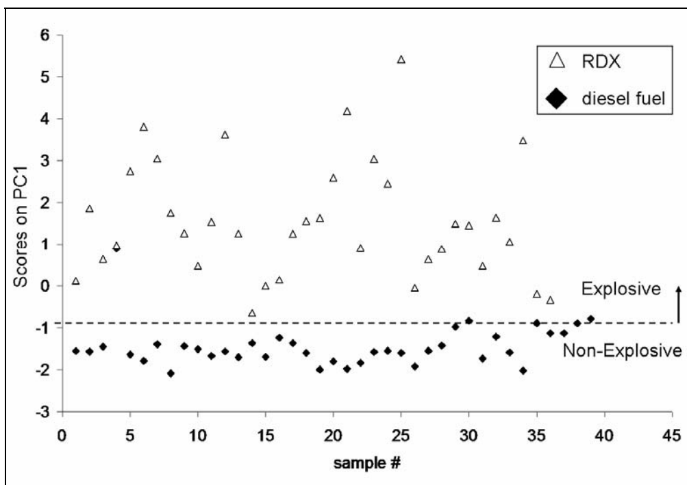
Figure 20. First principal component from atomic emission ratios O/C, O/H, N/C, N/H, and O/N from each single pulse LIBS spectrum of RDX and diesel fuel residue. (The dotted line represents the threshold that is moved along the y axis in order to create the ROC curve in figure 21.)
