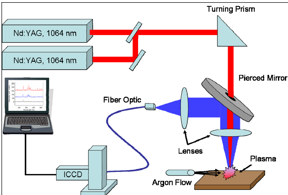
Figure 4. Laboratory double pulse LIBS experimental setup. (A 100-mm focal length convex lens is used to focus the Nd:YAG laser pulses on the sample surface. A 30-mm biconvex quartz lens focuses the plasma emission into the 600- \mu m fiber optic, which is sent to the spectrometer. An argon flow is positioned to eliminate the air above the sample surface.)
