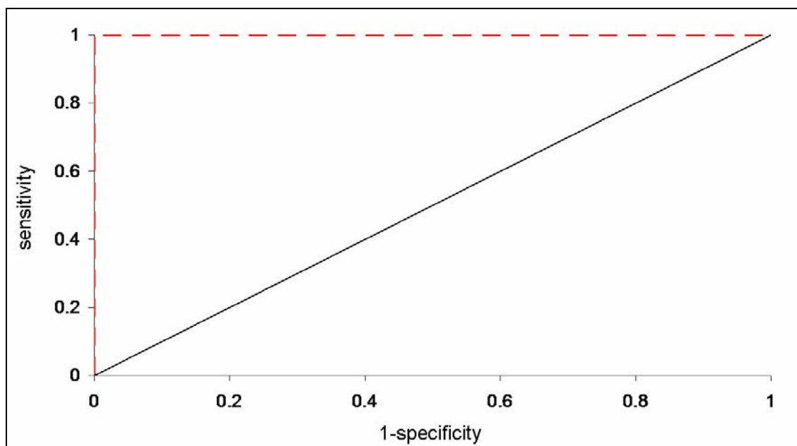
Figure 17. Examples of an ideal ROC curve (dashed line) and a ROC curve based on a random predictor (solid line).
