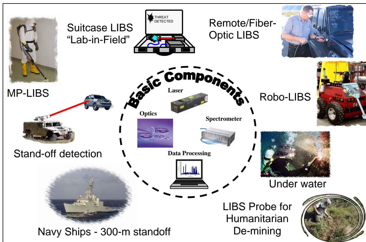
Figure 3. LIBS sensor suite and applications. (The basic LIBS components are compactible and ruggedizable and have been configured by different groups for a variety of applications.)
