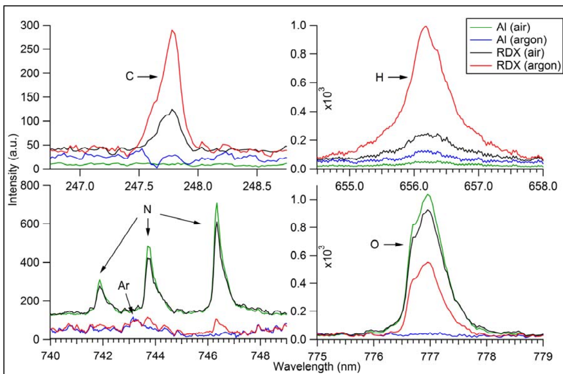
Figure 10. Single-shot spectra of Al and RDX residue on Al in air and under argon acquired with the MP-LIBS system. (Approximately 400 ng/mm 2 of RDX were applied to the Al foil substrate, and 10 spectra of each sample under each condition were acquired. The C [247 nm] and H [656 nm] signals from the RDX are enhanced under argon, while the O [777 nm] and N [742 to 747 nm] signals under argon are representative of the sample composition rather than atmospheric contributions.)
