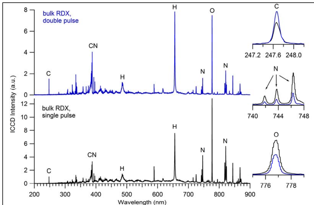
Figure 13. LIBS spectra of bulk RDX with a double laser pulse with \Delta t=2 \mu s (top) and a single laser pulse with equivalent pulse energy (bottom). (The carbon [inset right top] and hydrogen lines increase with double pulsing, while the nitrogen [inset right middle] and oxygen [inset right bottom] lines decrease because of the reduction in air entrained in the plasma.)
