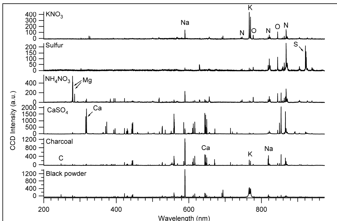
Figure 8. Single-shot LIBS spectra of black powder and its typical components: charcoal, calcium sulfate, ammonium nitrate, sulfur and potassium nitrate. (Strong lines of C, Mg, Na, N, K, O and S are labeled.)
