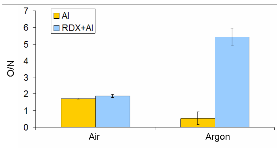
Figure 11. Relative oxygen to nitrogen peak intensities for Al and RDX residue on Al in air and in an argon flow (error bars represent \pm\sigma for the 10 spectra acquired with the MP-LIBS system). (The RDX residue can only be discriminated from the Al substrate [with the O/N ratio] under argon.)
