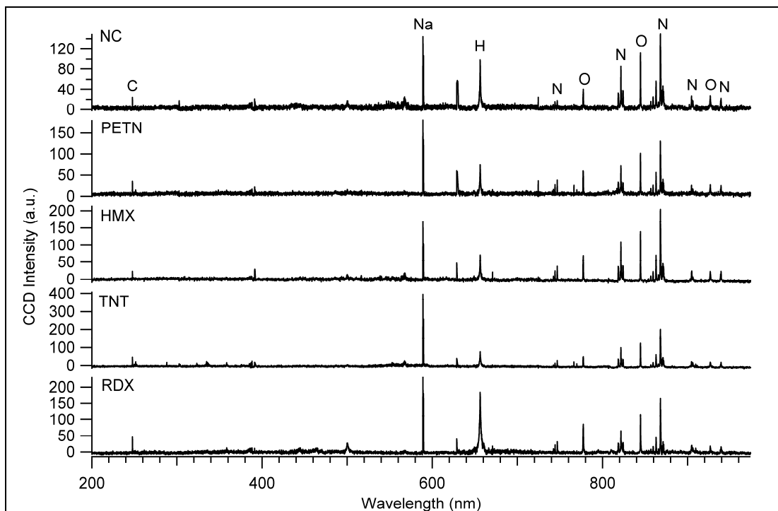
Figure 6. Single-shot LIBS spectra of pure energetic compounds: NC, PETN, HMX, TNT, and RDX.
