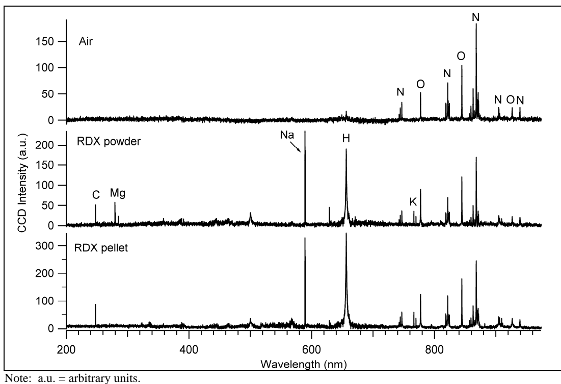
Figure 5. Representative single-shot LIBS spectra of an air spark, RDX powder, and an RDX pellet.
