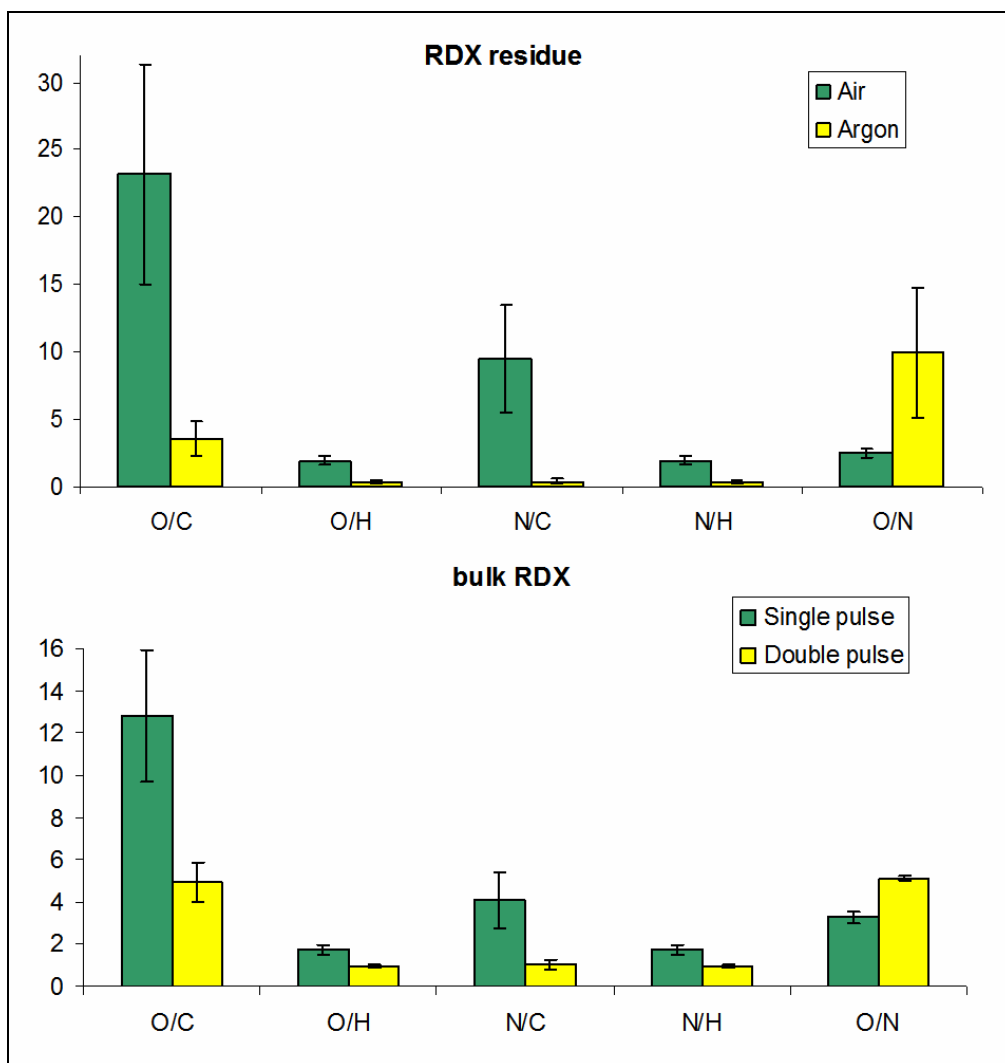
Figure 14. Peak atomic emission ratios from RDX residue on Al in air and in argon (top) and from bulk RDX with single pulse and double pulse ( \Delta t = 2 \mu s ) LIBS (bottom). (The error bars represent one standard deviation. The same trend is observed in both cases, indicating that double pulse LIBS results in ratios indicative of the sample composition rather than the air entrained in the plasma.)
