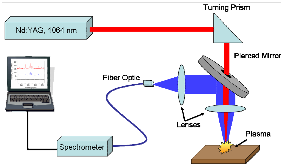
Figure 2. Basic LIBS experimental setup. (The laser is fired, passed through a turning prism and pierced mirror, and is focused on the sample surface to induce a microplasma. The resulting light emission characteristic of the sample composition is focused into a fiber optic and dispersed with a spectrograph to obtain the LIBS spectrum.)
