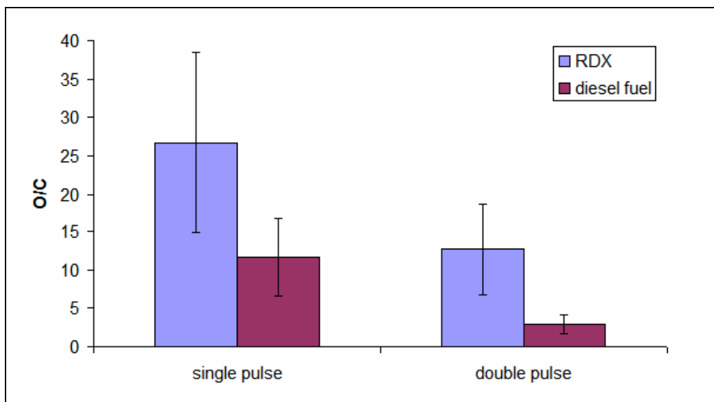
Figure 16. O/C peak atomic emission ratio comparison of RDX and diesel fuel for single pulse and double pulse ( \Delta t = 2 \mu s) LIBS. (The error bars represent one standard deviation. The two samples can only be discriminated based on the O/C ratio by double pulse LIBS.)
