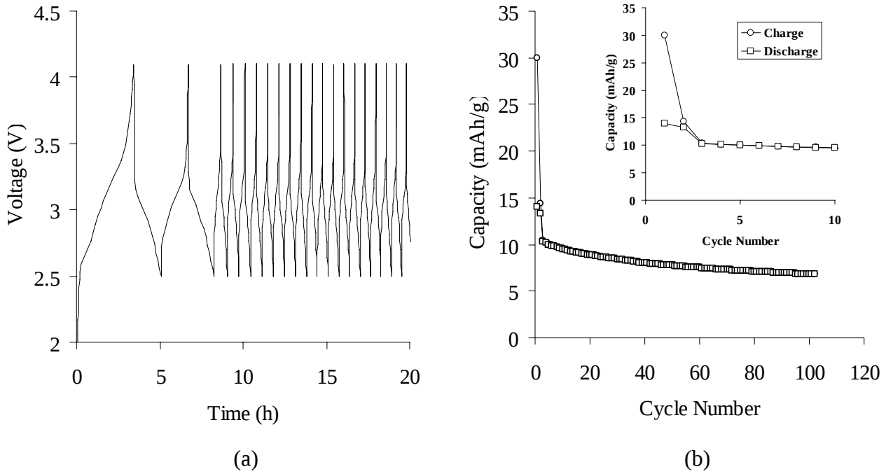
Figure 6. Liquid electrolyte full cell using non-woven carbon fabric and \text{LiFePO}_4 . (a) Voltage profile during the first 20 hours. (b) Charge and discharge curves. Inset shows an enlarged graph of cycles 1-10.
