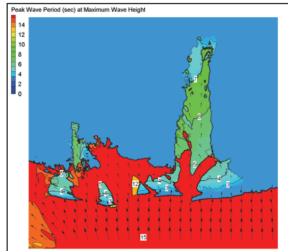
Figure 13. Mississippi-Alabama modeled peak wave period corresponding to the maximum wave height for 00:30 on 28 August 2005 to 00:00 UTC on 30 August 2005 (periods in seconds).
