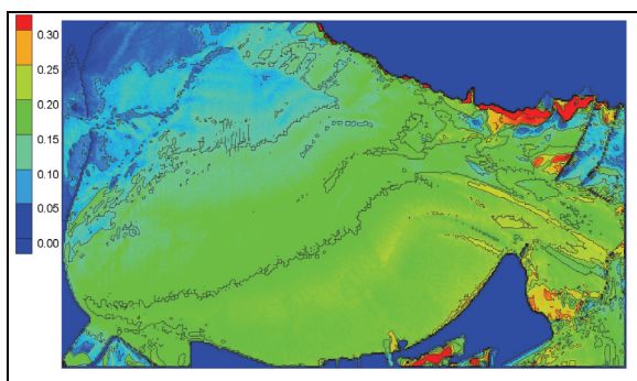
Figure 14. Differences in maximum wave height (in meters) for sensitivity run with 5 percent increase in wind speed for Lake Pontchartrain (plus 5 percent – base).
