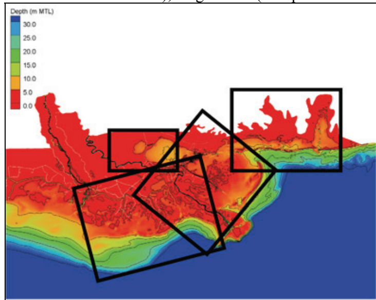
Figure 1. STWAVE modeling domains
