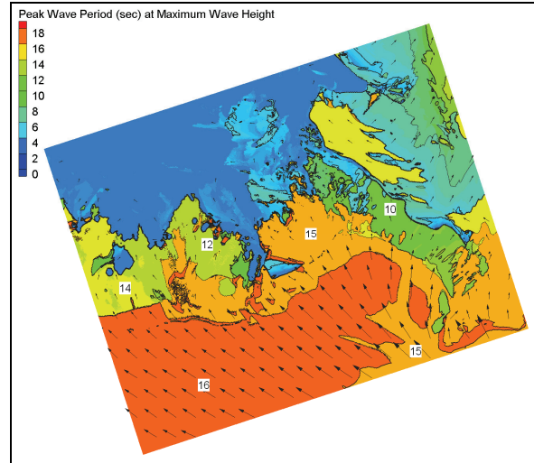
Figure 11. South Louisiana modeled peak wave period corresponding to the maximum wave height for 06:30 to 18:00 UTC on 29 August 2005 (periods in seconds).
