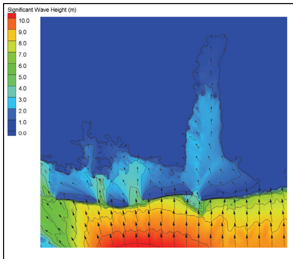
Figure 12. Mississippi-Alabama maximum modeled wave height for 00:30 on 28 August 2005 to 00:00 UTC on 30 August 2005 (wave heights in meters).
