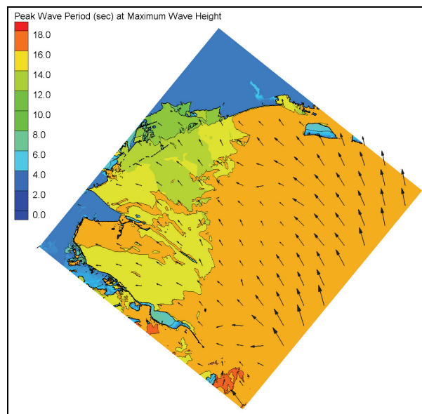
Figure 9. Southeast Louisiana modeled peak wave period corresponding to the maximum wave height for 00:30 UTC on 28 August to 00:00 UTC on 30 August 2005 (periods in seconds).
