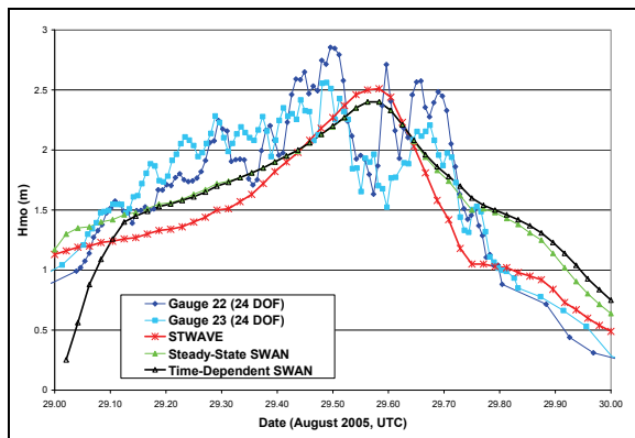
Figure 19. Time-dependent and steady-state SWAN and STWAVE modeled significant wave heights for Lake Pontchartrain measured and measured wave height.
