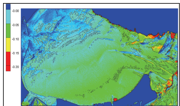
Figure 15. Differences in maximum wave height (in meters) for sensitivity run with 5 percent decrease in wind speed for Lake Pontchartrain (minus 5 percent – base).
