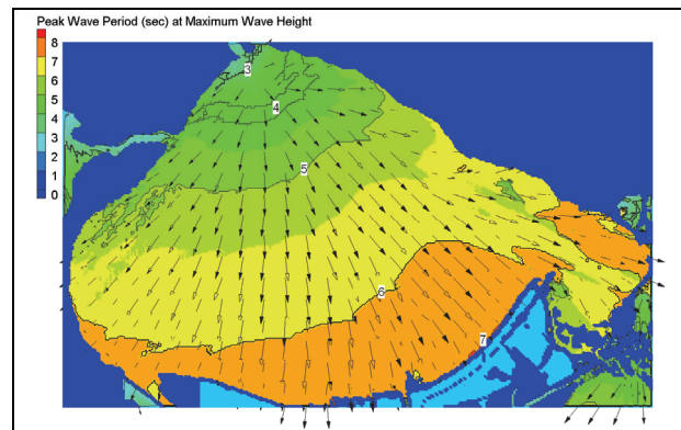
Figure 4. Lake Pontchartrain modeled peak wave period corresponding to the maximum wave height for 00:30 UTC on 28 August to 00:00 UTC on 30 August 2005 (periods in seconds)
