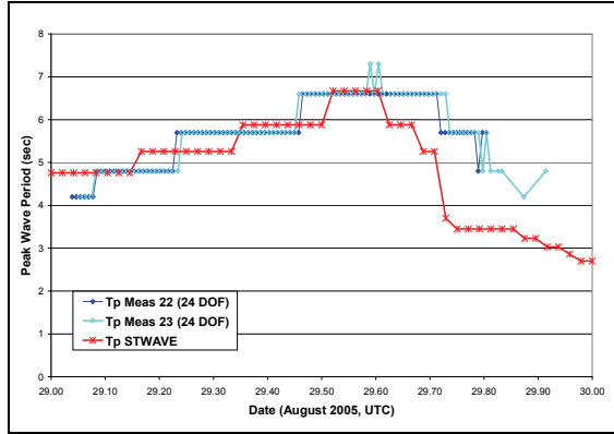
Figure 6. Lake Pontchartrain measured and modeled peak wave period.
