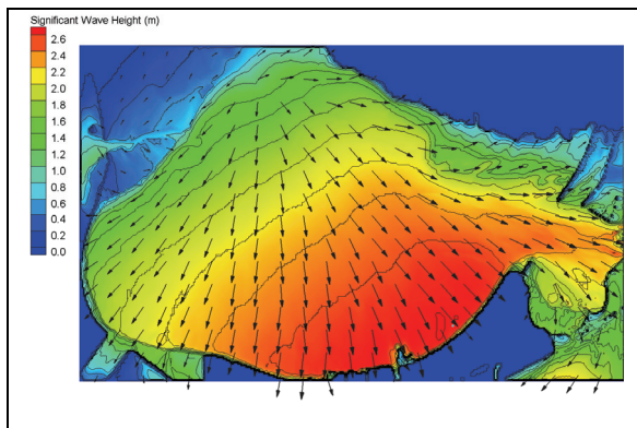
Figure 3. Lake Pontchartrain maximum modeled significant wave height and corresponding mean direction for 00:30 UTC on 28 August to 00:00 UTC on 30 August 2005 (wave heights in meters).
