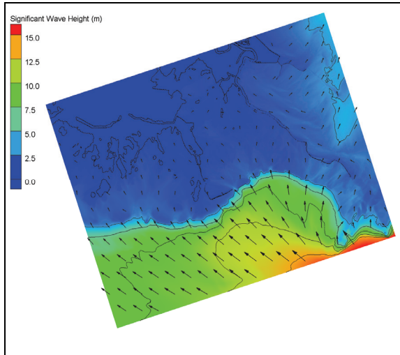
Figure 10. South Louisiana maximum modeled wave height for 00:30 28 August 2005 to 00:00 UTC on 30 August 2005 (wave heights in feet).
