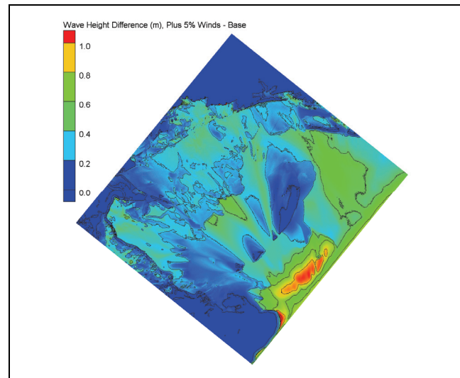
Figure 16. Differences in maximum wave height for sensitivity run with 5 percent increase in wind speed for Southeast Louisiana (plus 5 percent – base).
