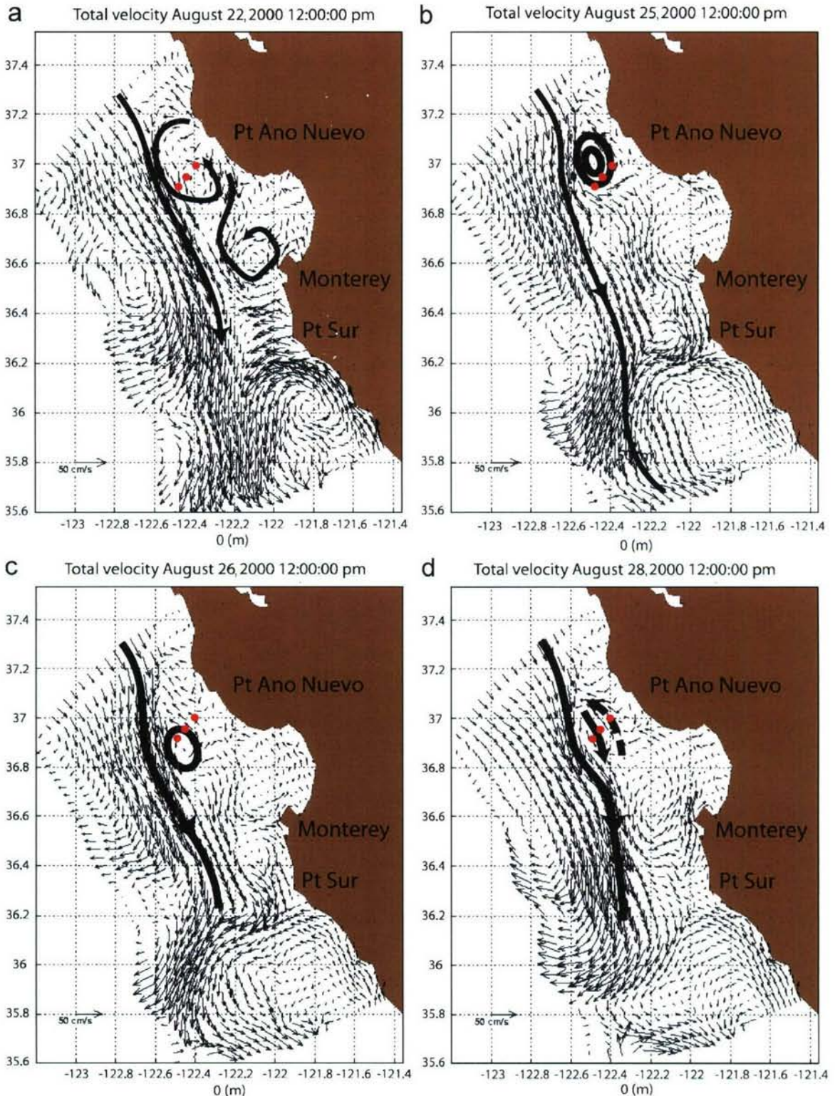
Fig. 8. Surface circulation predictions with the ICON model for: (a) 22 August 2000, (b) 25 August 2000, (c) 26 August 2000 and (d) 28 August 2000. Sketched lines emphasize features. Solid red circles show CTD stations as in Fig. 7.
