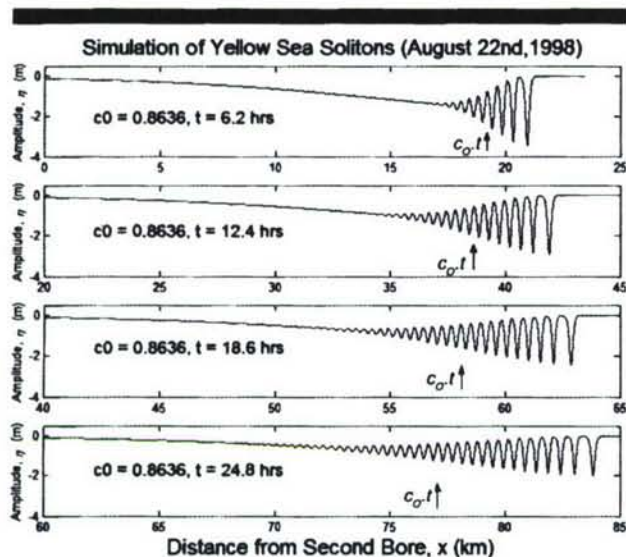
Figure 11. Soliton evolution modeled for two tidal periods. The arrows correspond to the centroid of the packet c_0 t which moves with the linear phase speed c_0 . The front of the packet moves with the nonlinear phase speed c .
