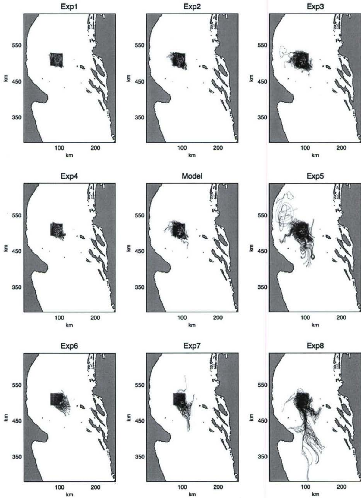
Fig. 9. Same as Fig. 4, but for Set-D.
