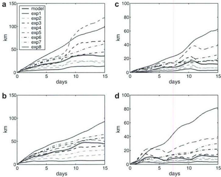
Fig. 11. Dispersion with respect to the launch locations, \rho(t) , for Exp-1 to Exp-8 in: (a) Set-A; (b) Set-B; (c) Set-C and (d) Set-D in NCOM.
