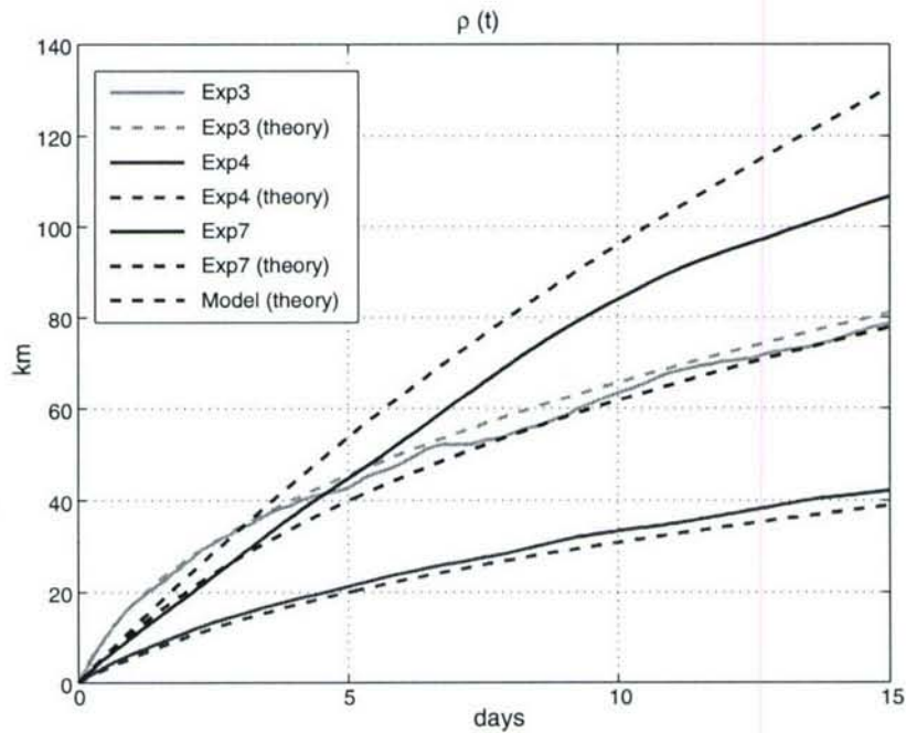
Fig. 6. Time evolutions of \rho(t) from the random field model (solid lines) and \rho_t(t) (dashed lines) for selected experiments.
