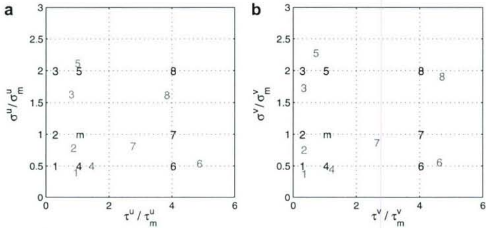
Fig. 10. Scatter plot of the targeted ( \frac{\sigma}{\sigma_m}, \frac{\tau}{\tau_m} ) and achieved ( \frac{\sigma_c}{\sigma_m}, \frac{\tau_c}{\tau_m} ) parameters for Exp-1 to Exp-8 calculated from particles released in NCOM, and averaged over Sets A to D in (a) zonal and (b) meridional directions.
