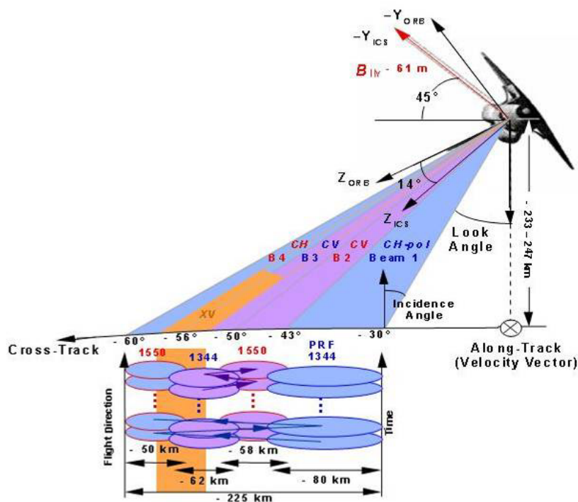
Fig.3.1 Scan scheme for the SRTM ScanSAR-Mode in C - Band using two polarizations coded in blue and pink in order to avoid too much resolution reduction reaching an improvement of a factor of 2 against normal Scan-SAR-Mode. Both swath and beam of X – SAR are coded in light brown. (Image Courtesy JPL)
