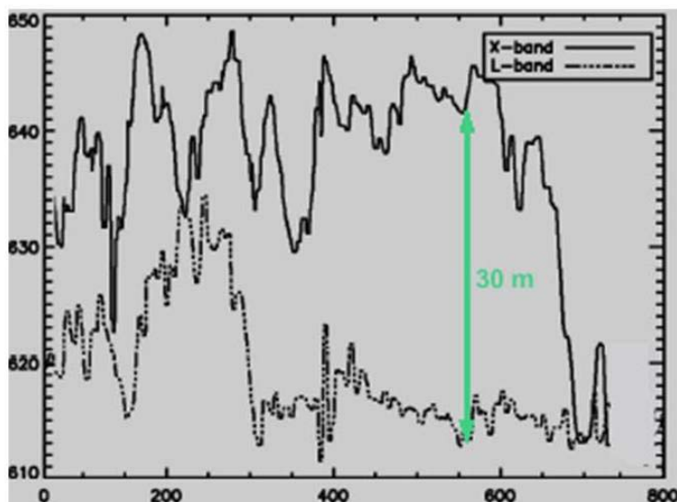
Fig. 4.1 X-Band and L-Band airborne Interferometry curves taken from E-SAR (DLR) The curves show the Difference in penetration of the two frequencies. L-Band penetrates down to the ground, X-Band will be reflected for the upper crown layer. (Ulbricht 1999)
