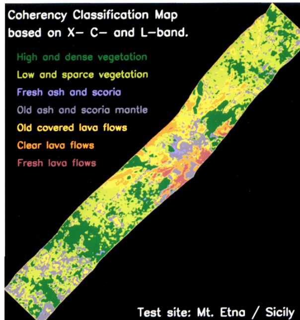
Fig. 9.4 Seven class coherence map based on L -, X -, and C -Band as well established using the procedure depicted in Fig. 9.3
