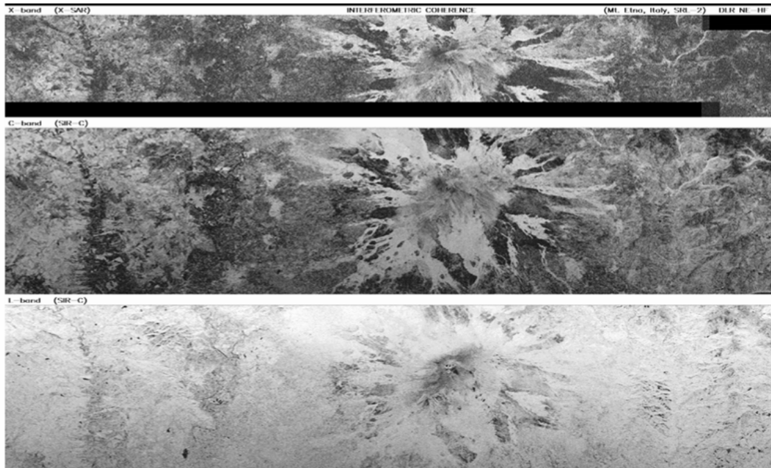
Fig. 9.1 Set of ground range coherence maps in X -, C -, L--Band ( sequence from top to bottom), white indicates high coherence black indicates low coherence.
