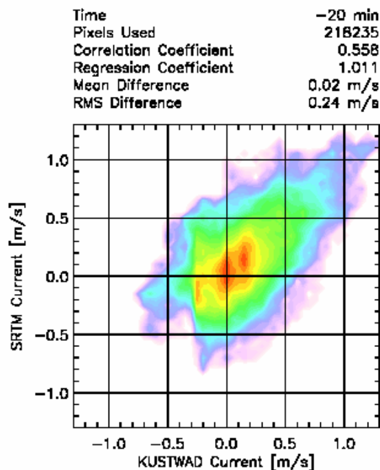
Fig.7.2 Scatter diagram showing the distribution of SRTM-derived vs. KUSTWAD-derived current components in the SRTM look direction, as well as corresponding statistical quantities, for the tidal phase 20 minutes before the SRTM overpass.
