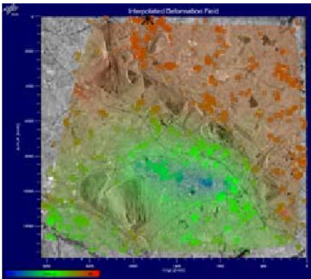
Fig.5.3 Example: estimated subsidence map, ± 4cm from blue to red
