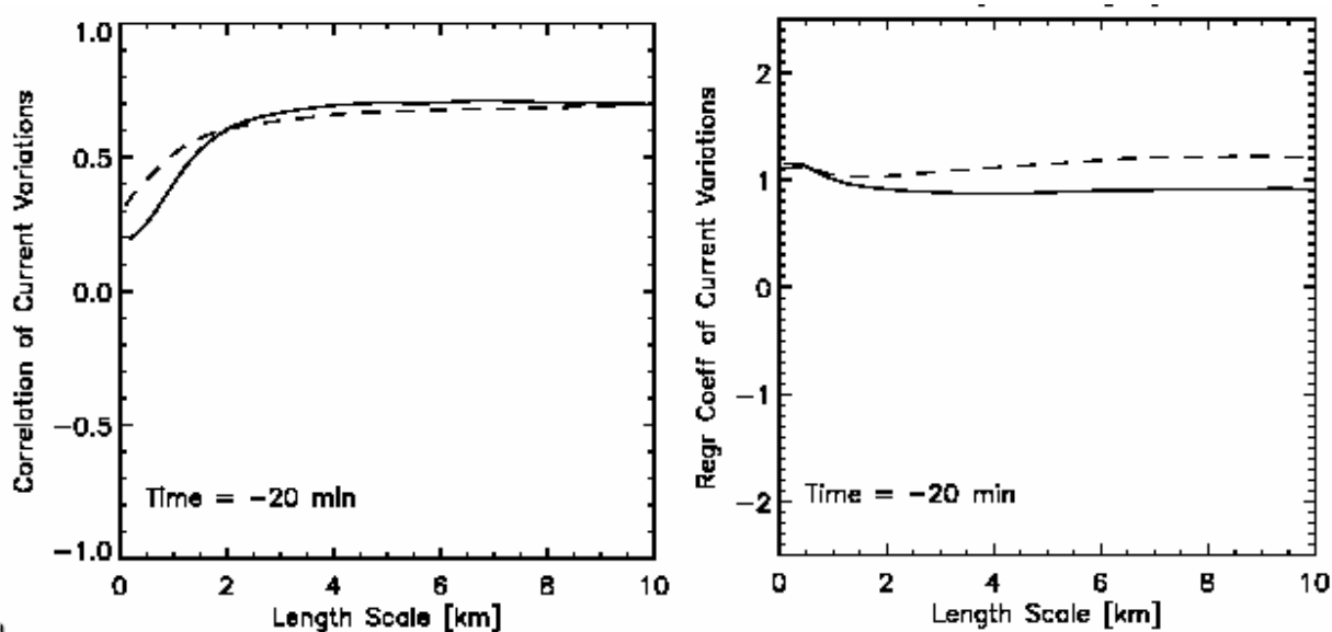
Fig.7.3. Correlation (left) and regression coefficient (right) of variations in the SRTM and KUSTWAD currents at different spatial scales parallel (solid lines) and perpendicular (dashed lines) to the SRTM look direction.
