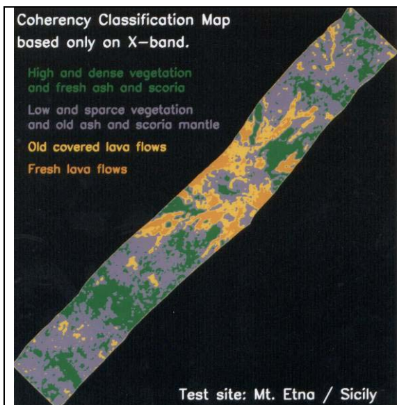
Fig. 9.2 Four class coherence map based on X-Band only
