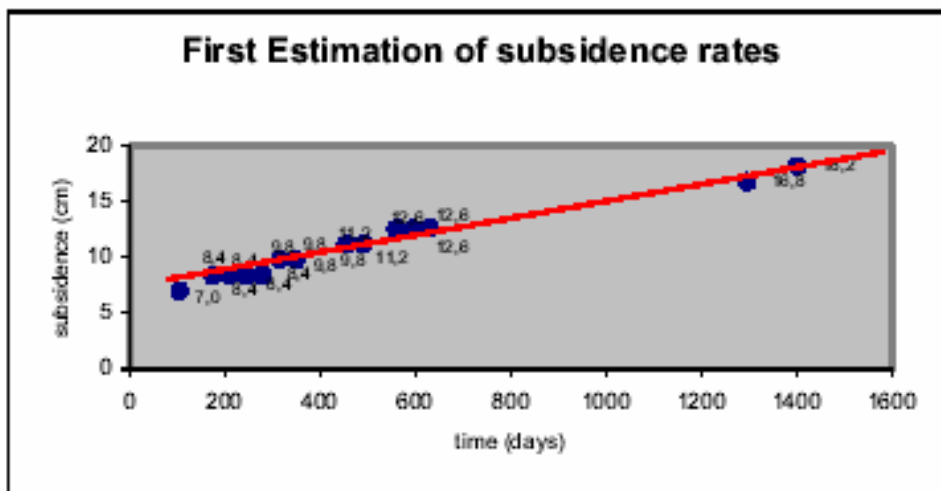
Fig.5.2 Time series of an Differential Interferogramme
