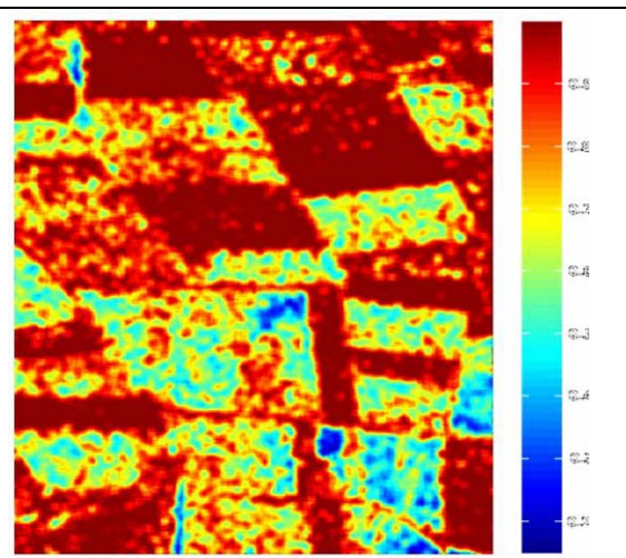
Fig. 10.3b Soil surface roughness Map ks (Hajnsek et. al. 2000)
