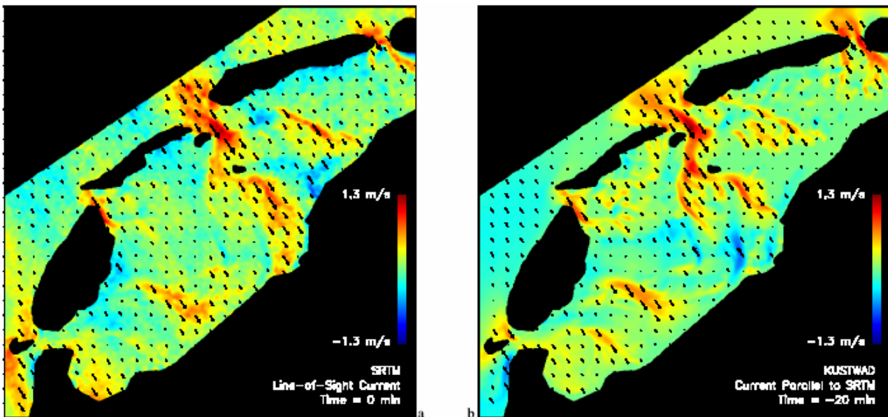
Fig.7.1 Line-of-sight current field in the test area as derived from the SRTM data (left) and as obtained from KUSTWAD for the tidal phase 20 minutes before the SRTM overpass (right); grid resolution is 100 m × 100 m; data points with valid currents from SRTM and KUSTWAD are shown only.
