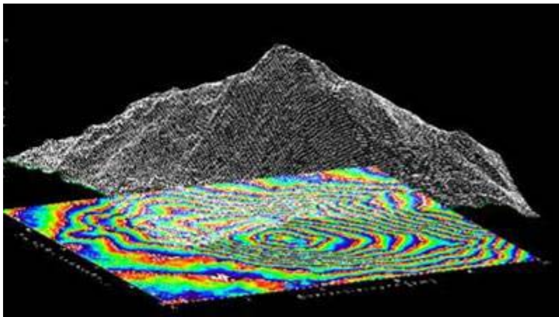
Fig 2.2 Digital Elevation Model and Interferogramme of Mount Etna taken in X-Band during the SIR-C Mission
