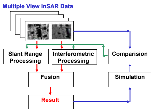
Fig. 6.1: Procedure for the extraction of building models from a combination of SAR images and associated interferometric data [6] (Bolter, 2001).
