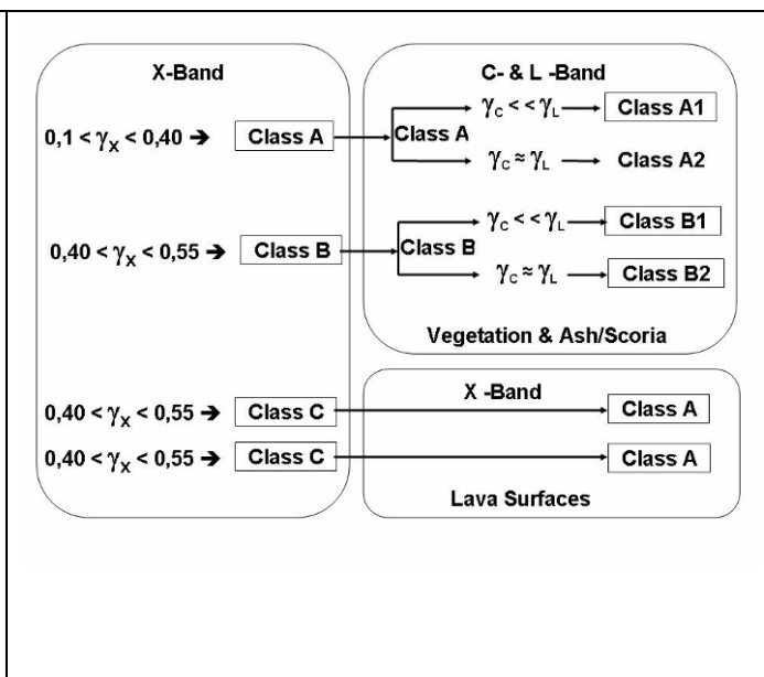
Fig. 9.3 Schematic representation of the interpretation procedure accomplished over the coherence Maps
