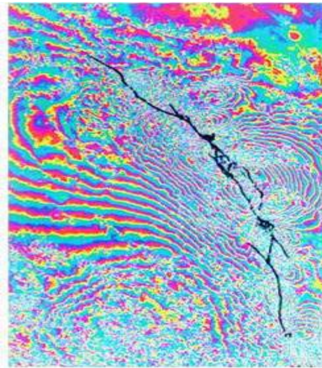
Fig.2.1 Interferogramme showing the deformation of the ground caused by the so called Landers Earthquake. Each cycle of interference colours (red through blue) represents an additional 28 mm (half the 56 mm wavelength of the ERS1-SAR) of ground motion in the direction of the satellite.[Massonnet, 1993]
