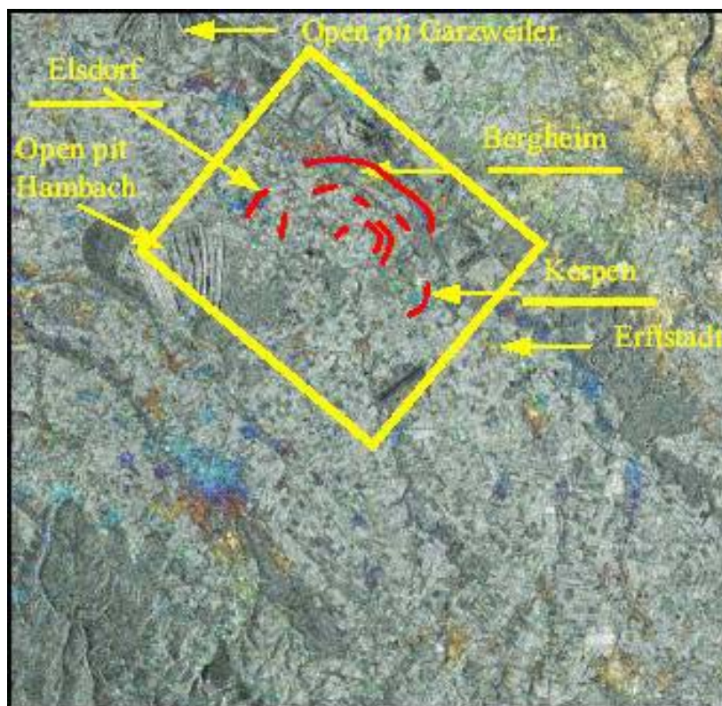
Fig. 5.1 Differential Interferogramm with amplitude overlay
