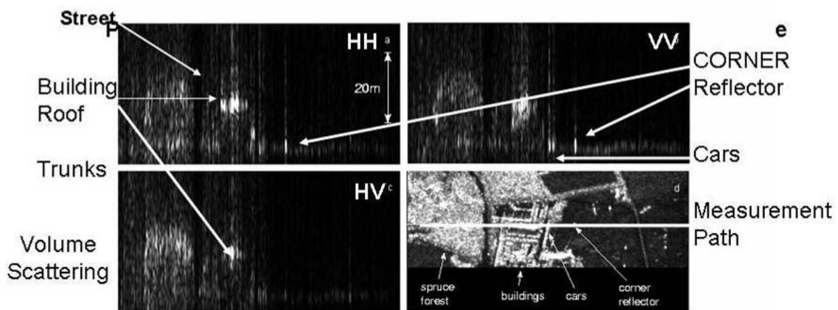
Fig.4.2: Tomography for Scattering Analysis. Different scattering mechanisms along the white line at different altitudes at different polarizations.a:HH; b:VV; c: HV. d: measurement path. The buildings roof is bright, The bright HH and VV single bounce is the corner reflector, double bounces happen at parts of the buildings roof and at the lower parts of trunks, in tree crowns & under story volume scattering dominates.(Reigber 1999)
