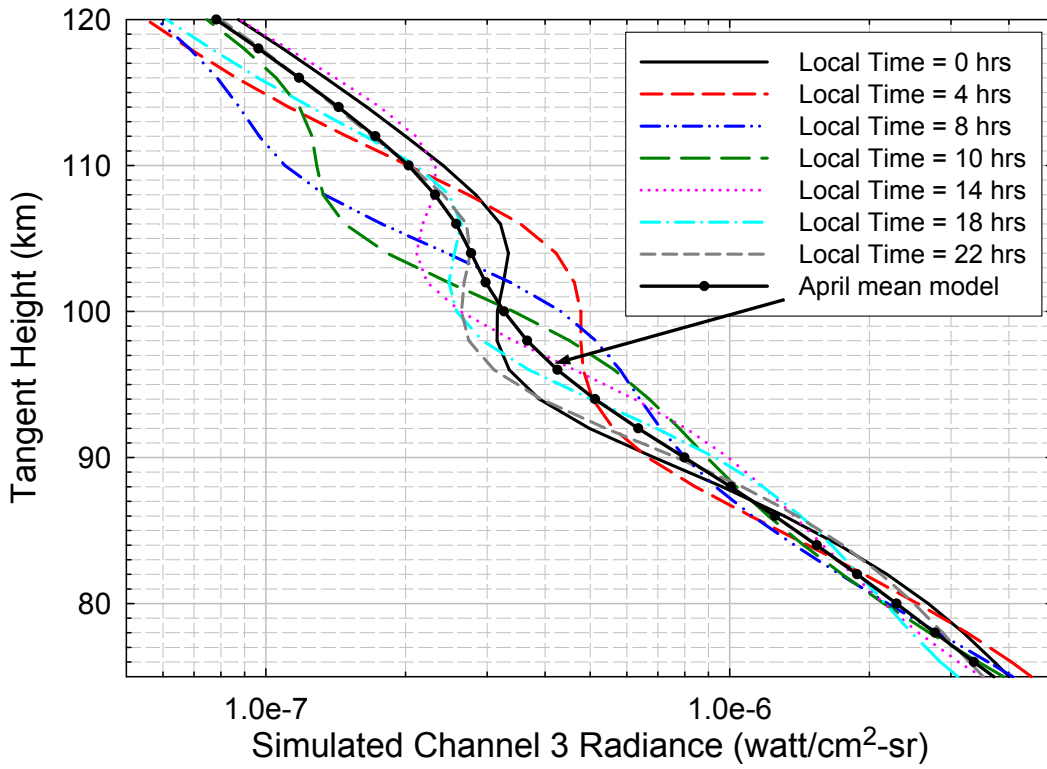
Figure 11. Predicted radiance at the equator in April for different local times, from GSWM/ARC modeling. Zonal mean radiance is also shown.
