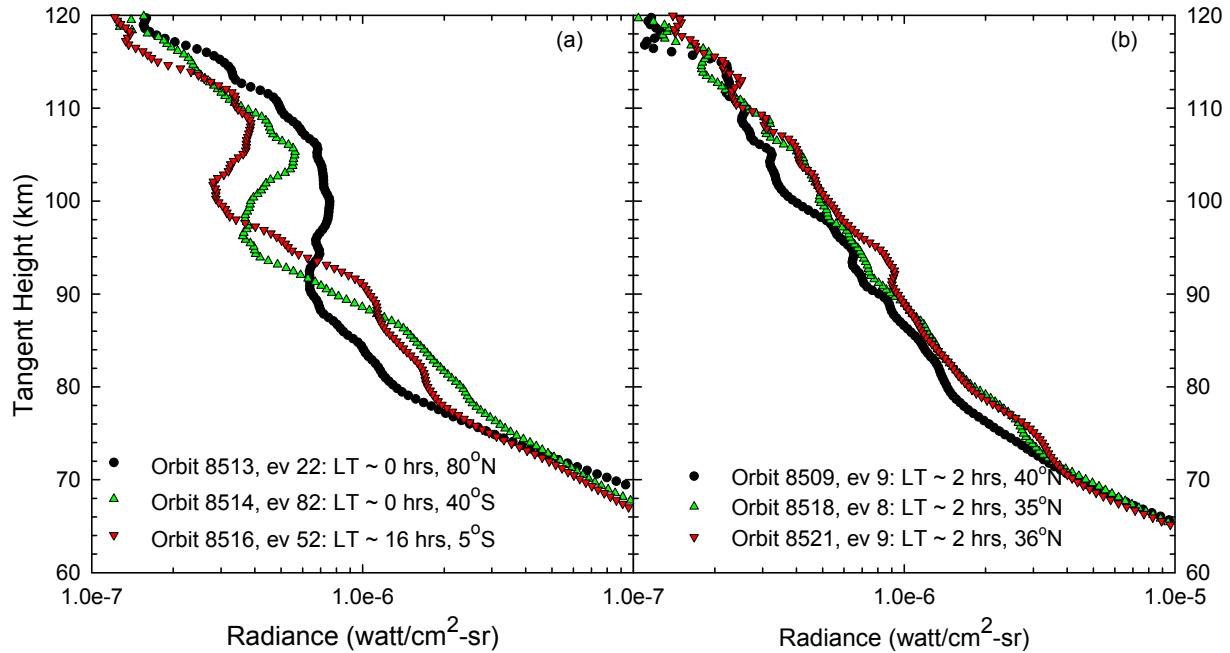
Figure 1. SABER limb radiance from events of July 3, 2003. (a) Three cases with positive gradients at different heights above 90 km; (b) Three cases with no such features
