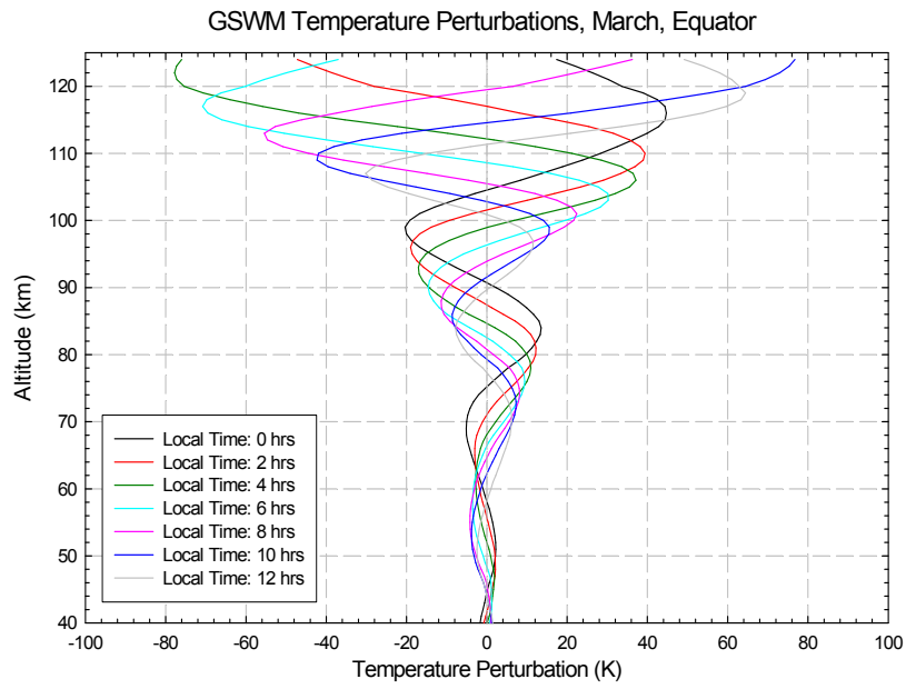
Figure 9. GSWM predictions of temperature perturbations for March at the equator, for different local times.
