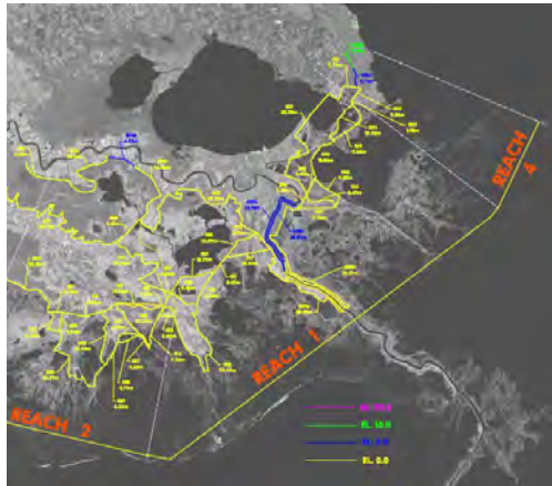
Figure 108 Locations of Reach 1 and Reach 4 for differentiation in soil parameters
