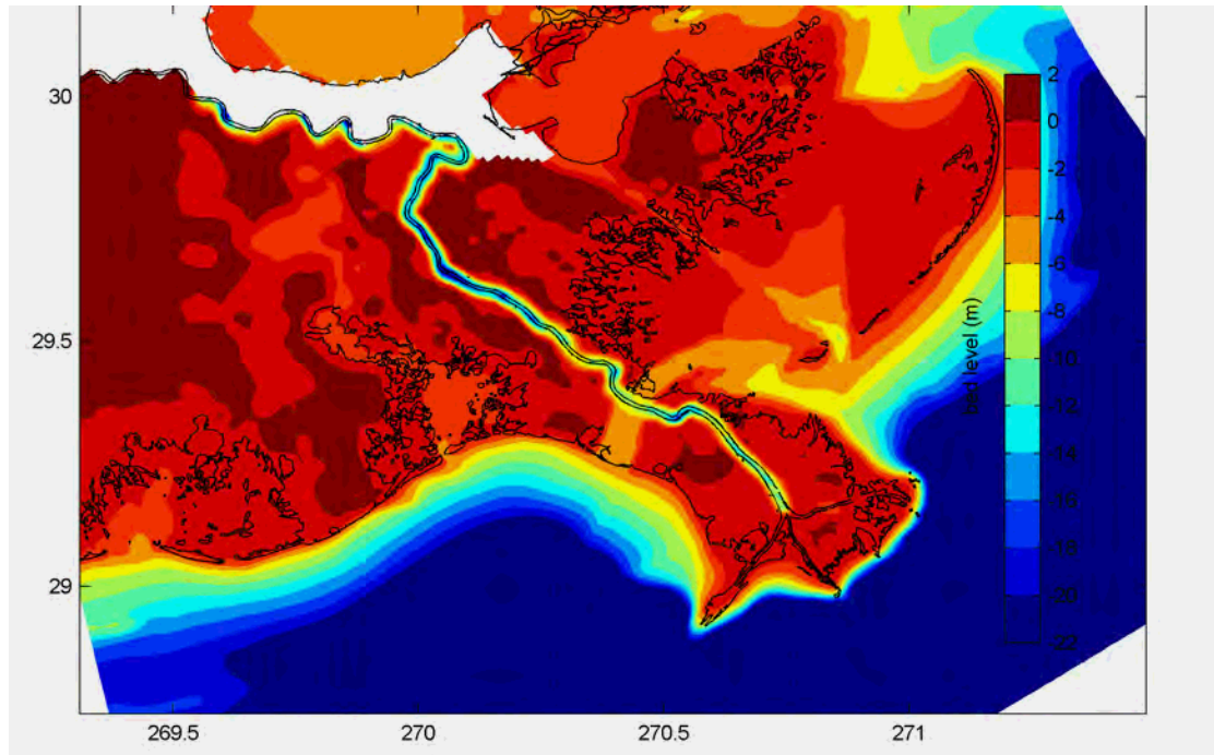
Figure 84 Bathymetry with wide and shallow diversion channels (m)
