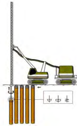
Figure 119 Schematic representation of improving the subsoil by mix in place techniques
