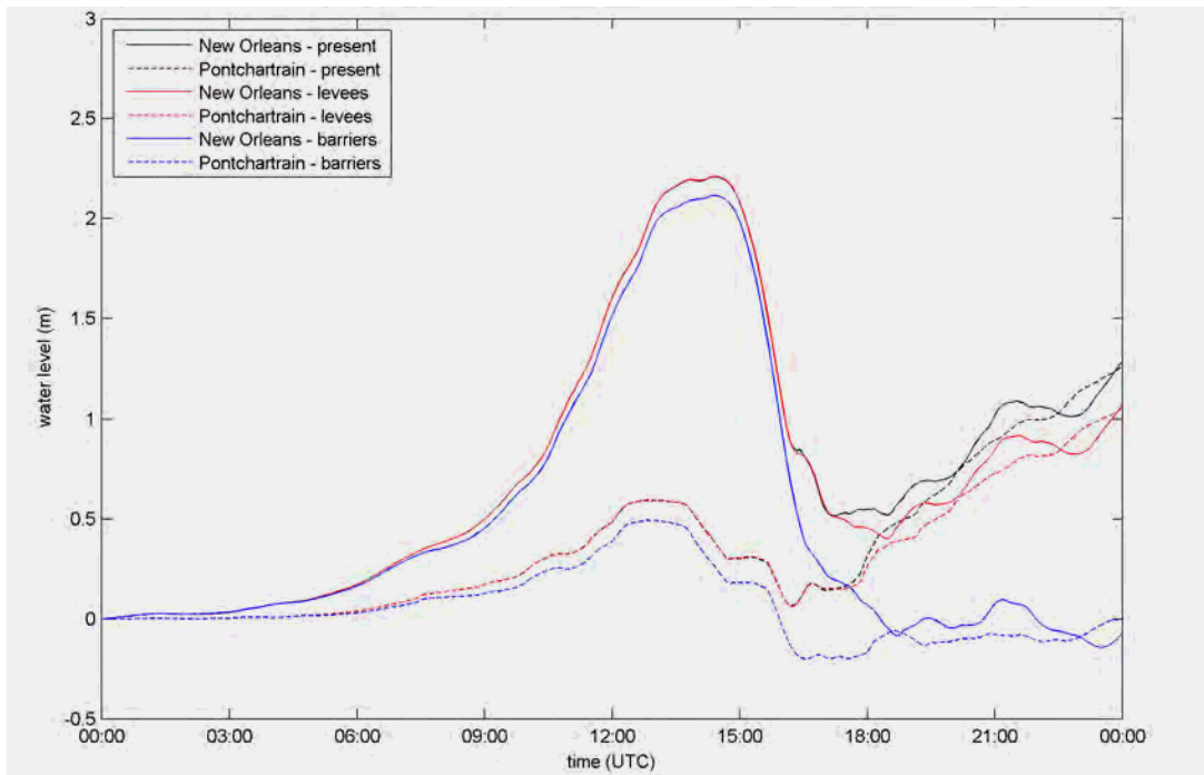
Figure 78 Water levels near New Orleans and in the middle of lake Pontchartrain for different barrier configurations.
