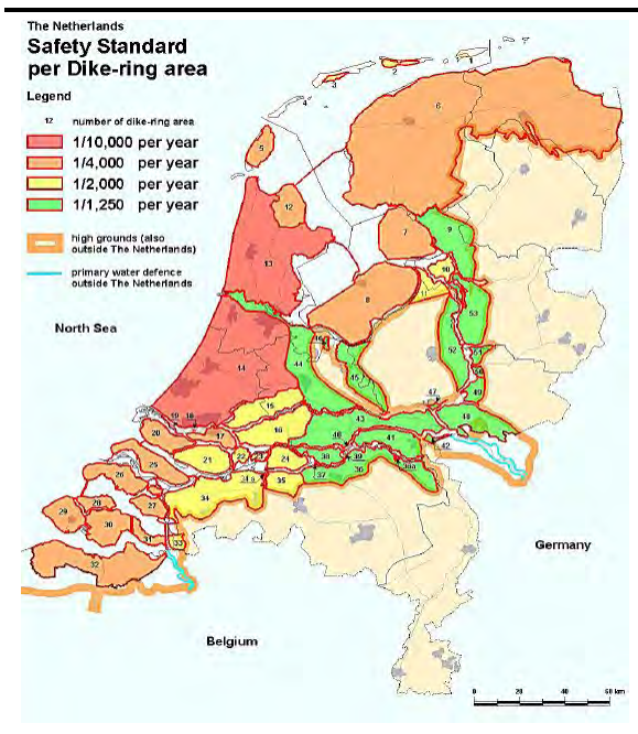
Figure 147 Flood protection standards for primary flood protection infrastructure
