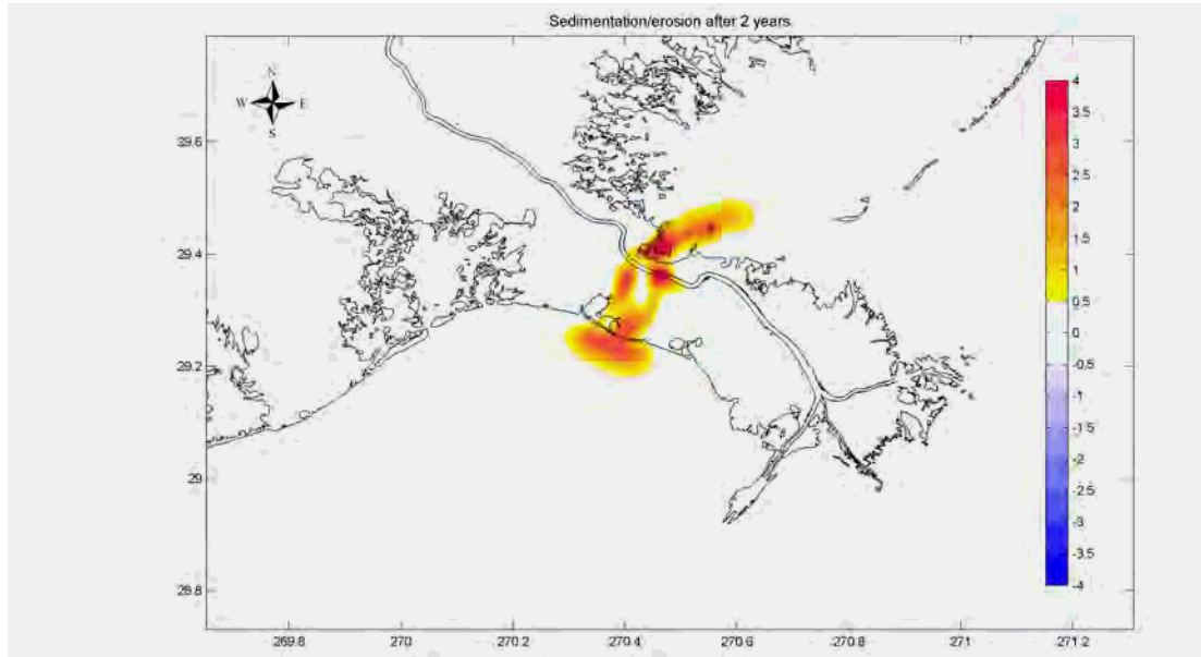
Figure 85 Deposition of river sediments over 2 year in the present situation (m).
