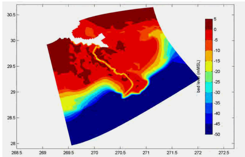
Figure 90 Model bathymetry (m)
