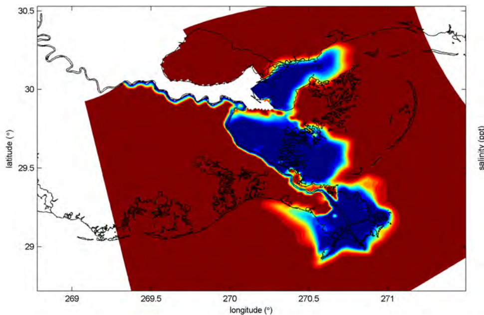
Figure 89 Salinity levels after on month (crevassing in Barataria Basin)
