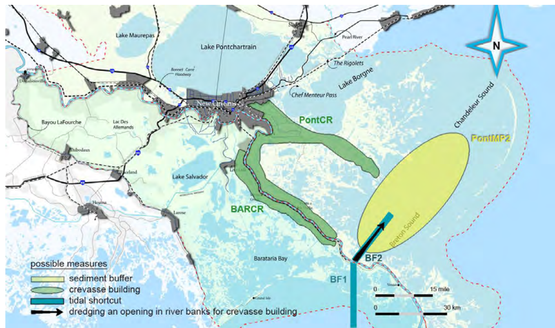
Figure 12 Interventions for long-term natural surge reduction (codes of measures are explained in Appendix H).
