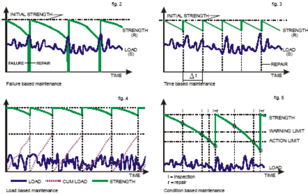
Figure 141 Maintenance concepts
