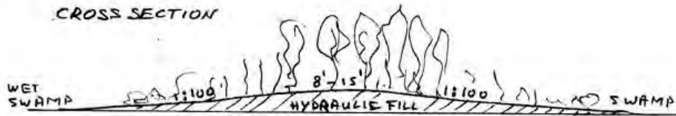
Figure 125 Schematic cross-section ridge-levee (distorted scale)
