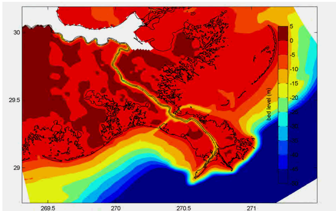
Figure 81 Bathymetry with narrow diversion channels (m).
