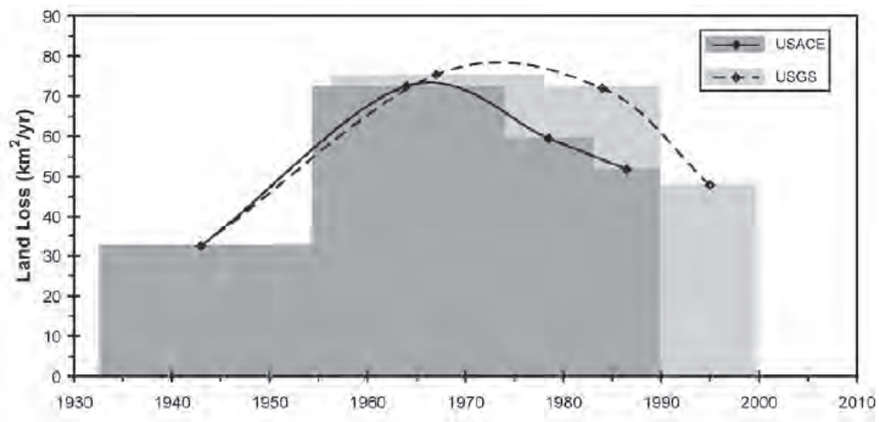
Figure 41 Land-loss rates, Louisiana delta plain, 1932-2000. Data from the U.S. Army Corps of Engineers (USACE; Britsch and Dunbar, 1993) and the U.S. Geological Survey (USGS; Barras et al., 2003). Copied from Bernier et al. (2006).
