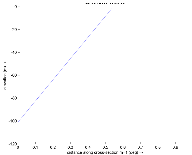
Figure 59 Cross-shore profile for the straight coast case.
