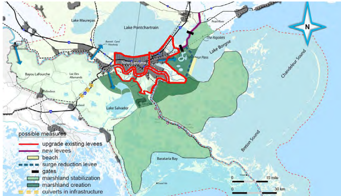
Figure 24 Measures in the Preferred Strategy.
