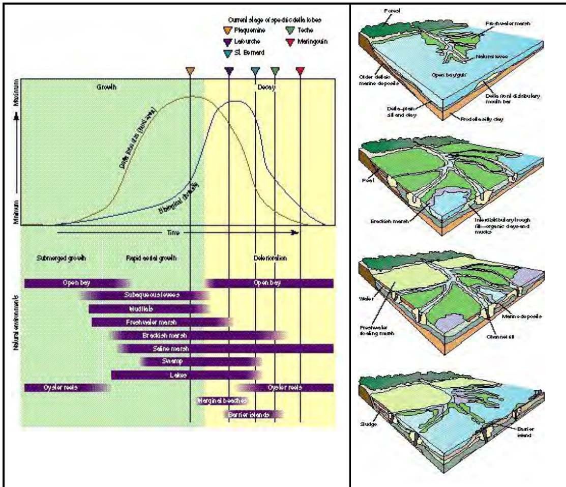
Figure 44 Graphical depiction of the growth and decay of a delta. Habitat and biological diversity peak in the early to middle stage of the decay phase. © Houston Geological Society. Figure copied from http://biology.usgs.gov/s+t/SNT/noframe/gc138.htm
