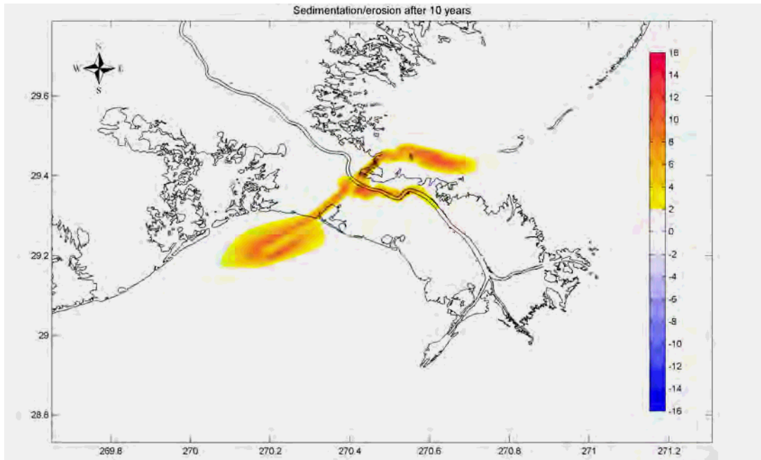
Figure 82 Deposition of river sediments over 10 year with narrow diversion channels (m)
