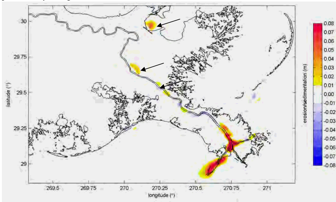
Figure 88 Erosion and sedimentation (m) after crevassing in Lake Borgne
