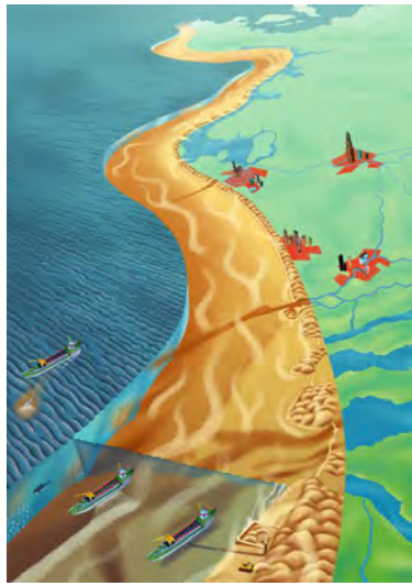
Figure 153 Coastal sediment system
