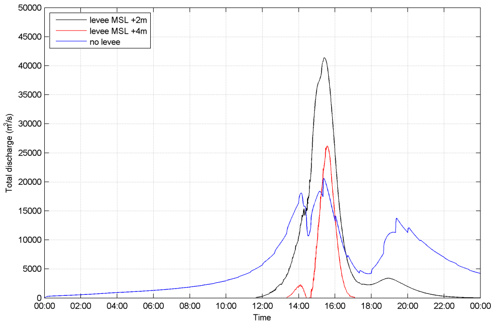
Figure 67 Discharge over levee for different levee crest heights
