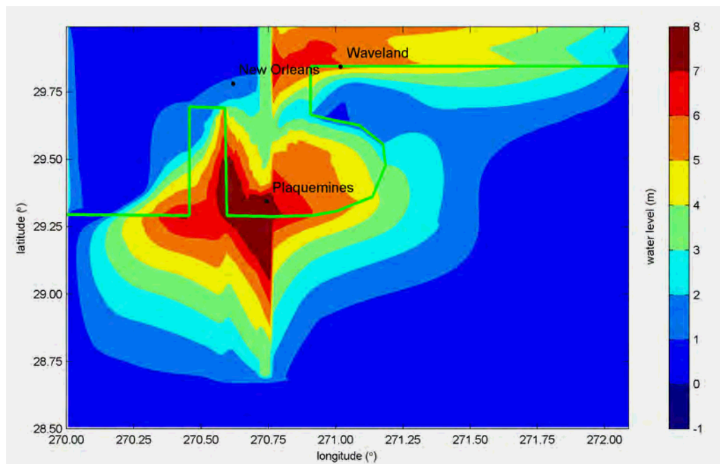
Figure 72 Maximum surge levels reference (present) situation
