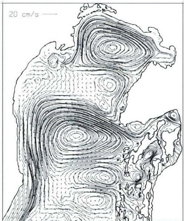
Figure 14. Model 10-m currents at 09Z, 12 January 2003.
