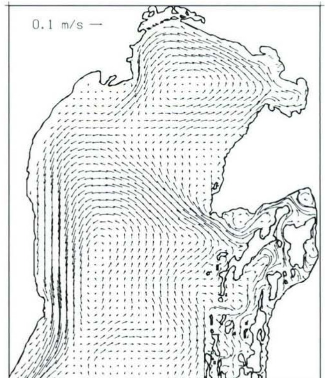
Figure 7. Model mean currents for January–February at 5 m.
