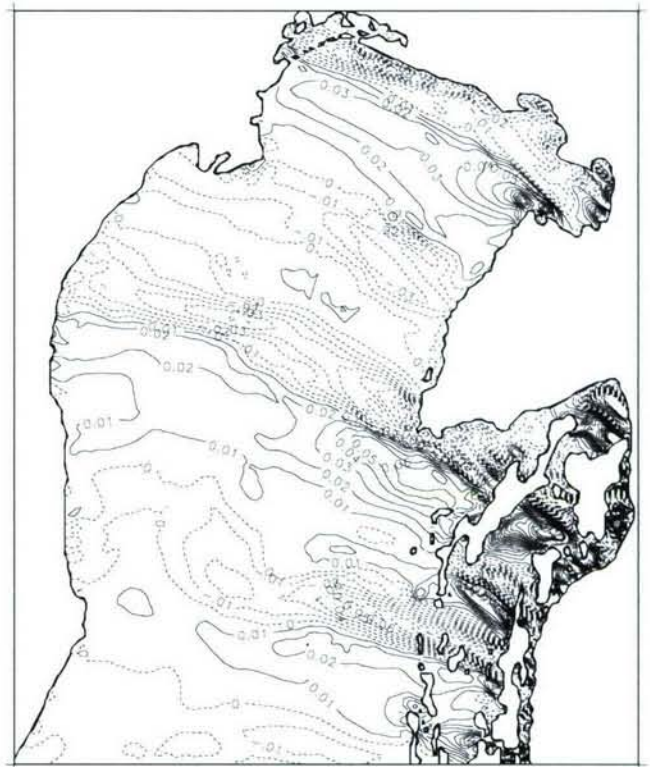
Figure 15. Time-averaged COAMPS wind stress curl for period 09Z, 11 January, to 09Z, 12 January 2003. Contour interval is 0.01 Pa/km.
