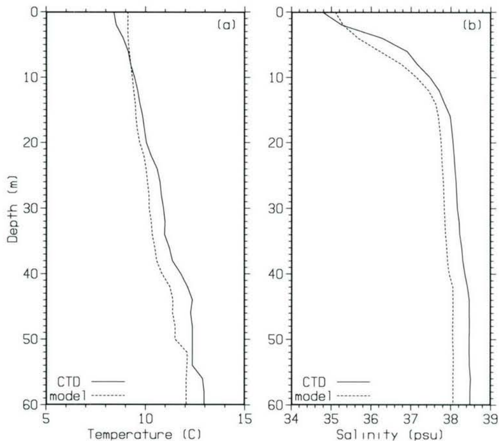
Figure 10. Model and CTD mean (a) temperature and (b) salinity profiles for January–February.
