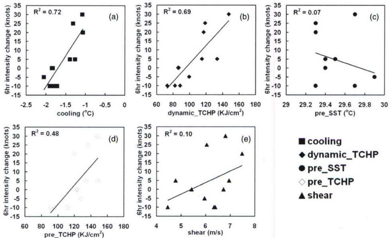
Fig. 18. Intensity change of 6 h of Dianmu with the five parameters, i.e., (a) self-induced SST cooling, (b) dynamic TCHP, (c) pretyphoon SST, (d) pretyphoon TCHP, and (e) vertical wind shear.
