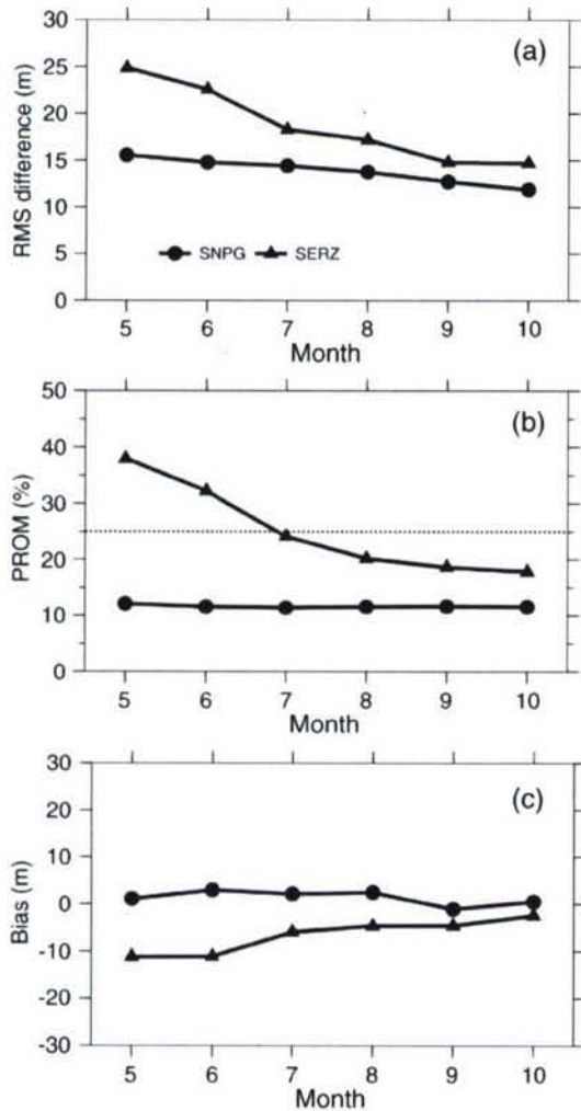
Fig. 8. (a) Monthly rms difference, (b) PROM, and (c) bias of the TLM_WNP-estimated D26 in SNPG and SERZ. The dotted line in (b) depicts the accuracy threshold of 25% PROM.
