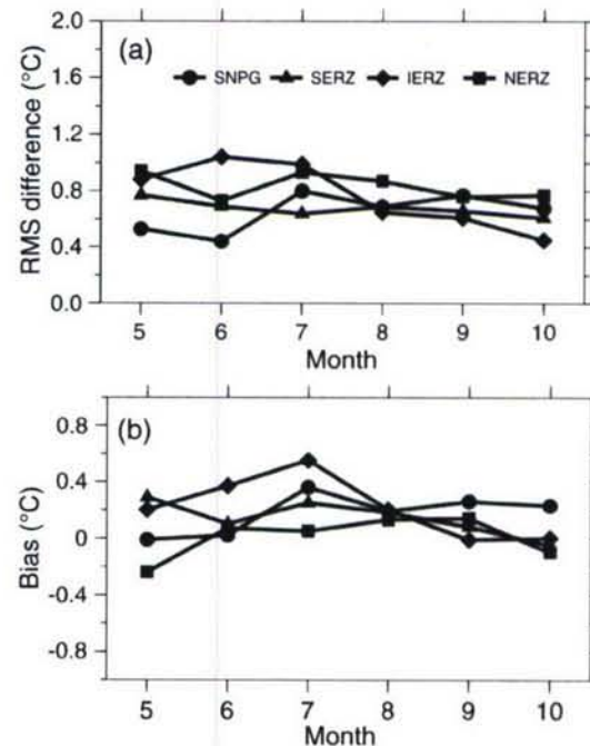
Fig. 9. Comparison of the value of (a) rms difference and (b) bias for the SST in the TLM_WNP in the SNPG, SERZ, IERZ, and NERZ.
