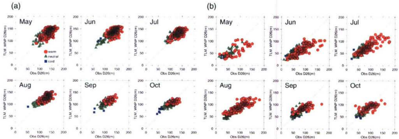
Fig. 7. As in Fig. 4, the monthly scatter plots of the TLM_WNP-estimated D26 and the in-situ GTSP D26 in the (a) SNPG and (b) SERZ during 2002–2005.
