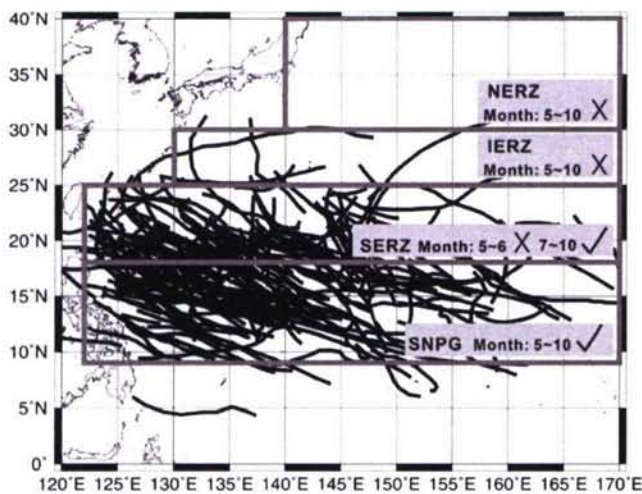
Fig. 10. Tracks of the 562 typhoons in the past 45 years (1960–2004) passing the western North Pacific and the applicable areas.
