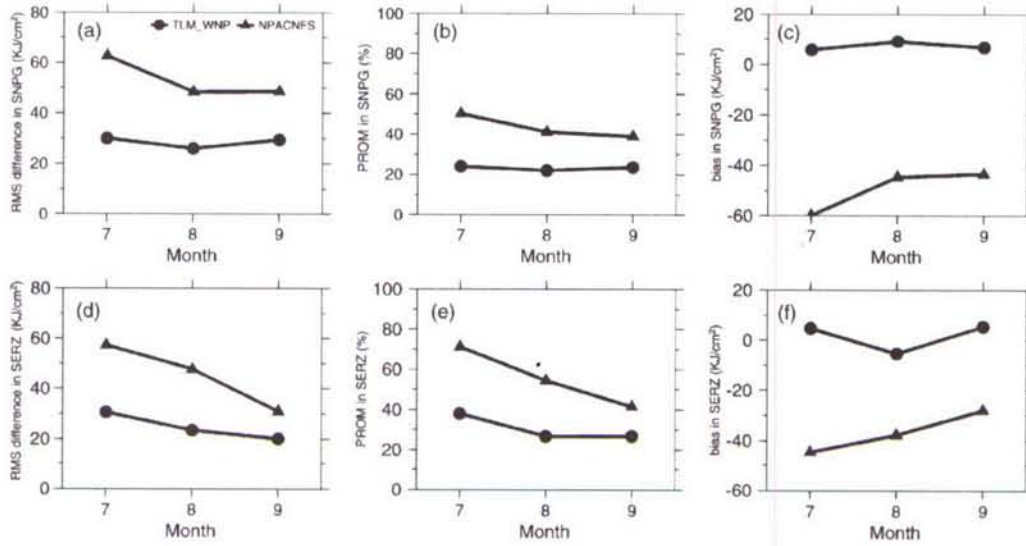
Fig. 13. Comparison of the value of the monthly rms difference, PROM, and bias for the TCHP estimation using the TLM_WNP and the NPACNFS profiles for (a)–(c) SNPG and (d)–(f) SERZ.
