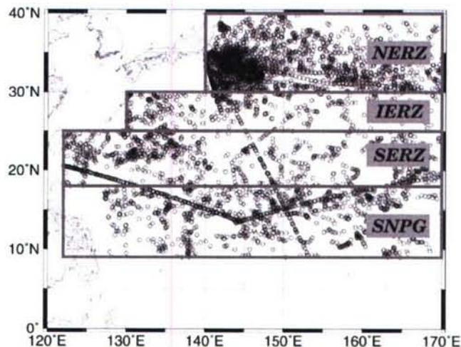
Fig. 3. Locations of the four validation zones in the western North Pacific including the SNPG, the SERZ, the IERZ, and the NERZ. Circles denote the locations of the 5684 GTSPP in-situ profiles that were used in the validation.
