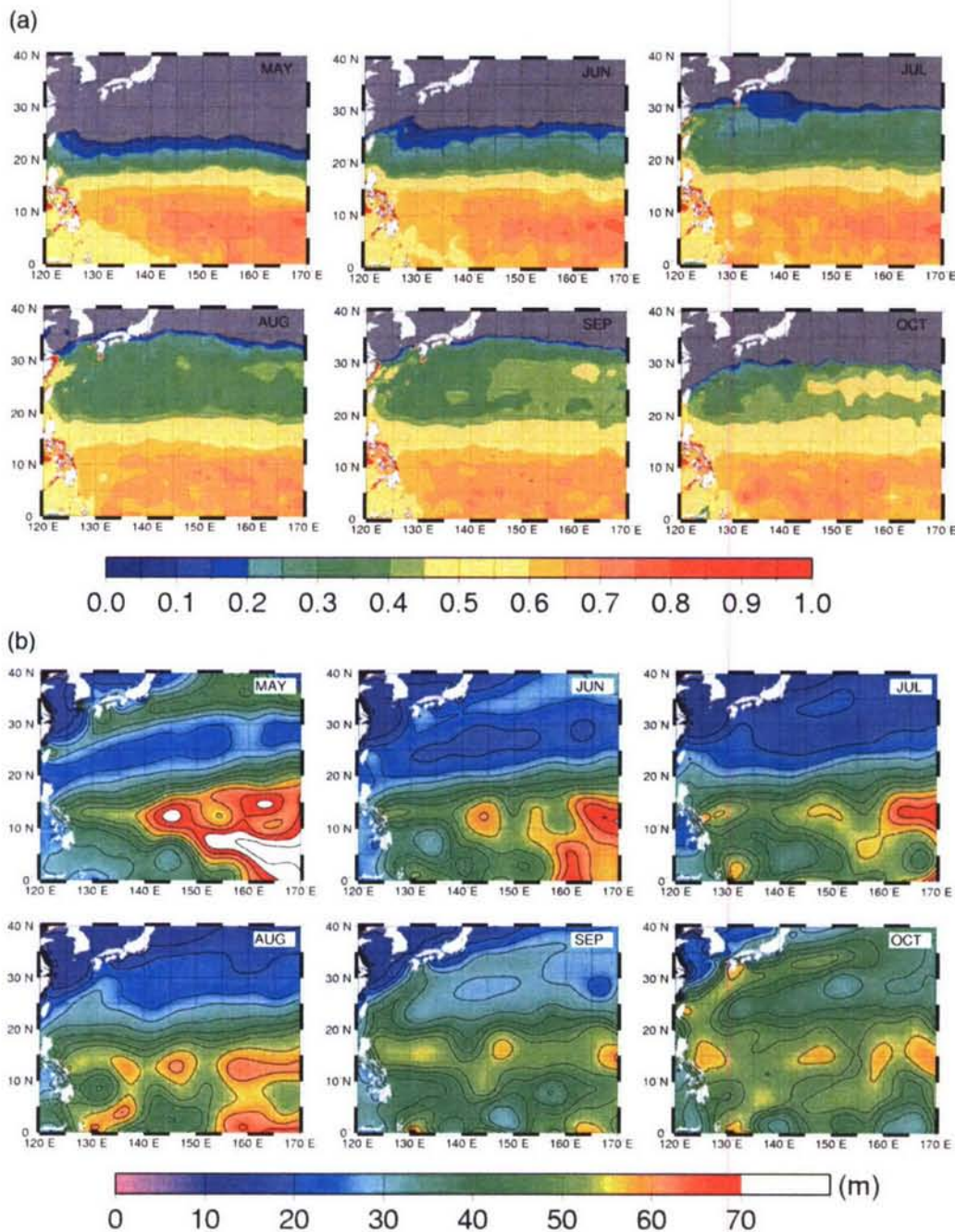
Fig. 2. (a) Monthly climatological ratio between D26 and D20 during May–October in the western North Pacific (Data source: NOAA/NODC/WOA01, [33]). Gray represents land or areas where the SST is lower than the 26 °C and no ratio can be calculated. (b) Monthly climatological mixed-layer depth from the U.S. NRL.
