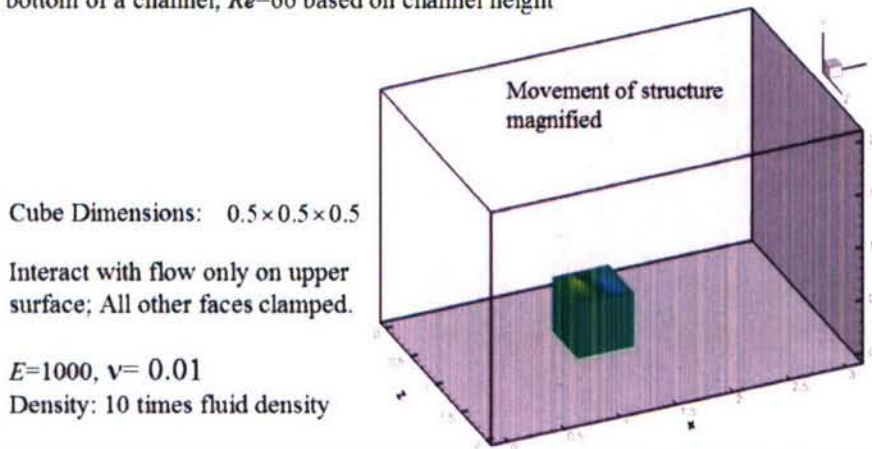
FSI- Nektar with StressNektar : Flow past a cube at bottom of a channel; Re=66 based on channel height
