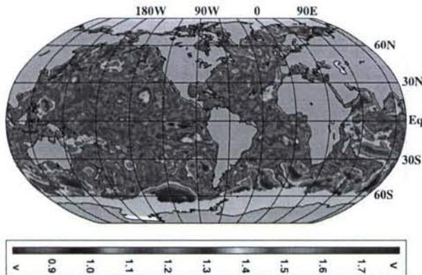
Figure 1. Spatial variations of wind drag coefficient over the global ocean on 1 Aug 2005 (00Z). Note values in the color bar must be multiplied by 10^{-3} . Effects of ocean currents and waves are excluded in calculating these drag coefficients. The regions where ice exists are masked out (shown in gray).
