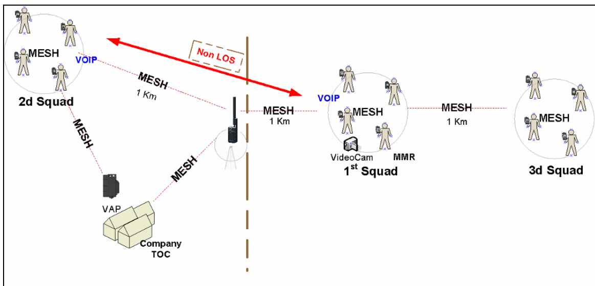
Diagram 1. Scenario 1 Mesh Only.
