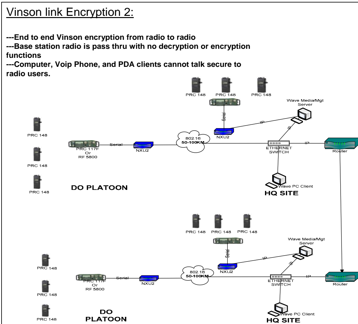
Diagram 9. End to End Audio Encryption Option Two
