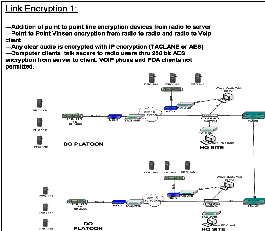
Diagram 8. Link Encryption Option One
