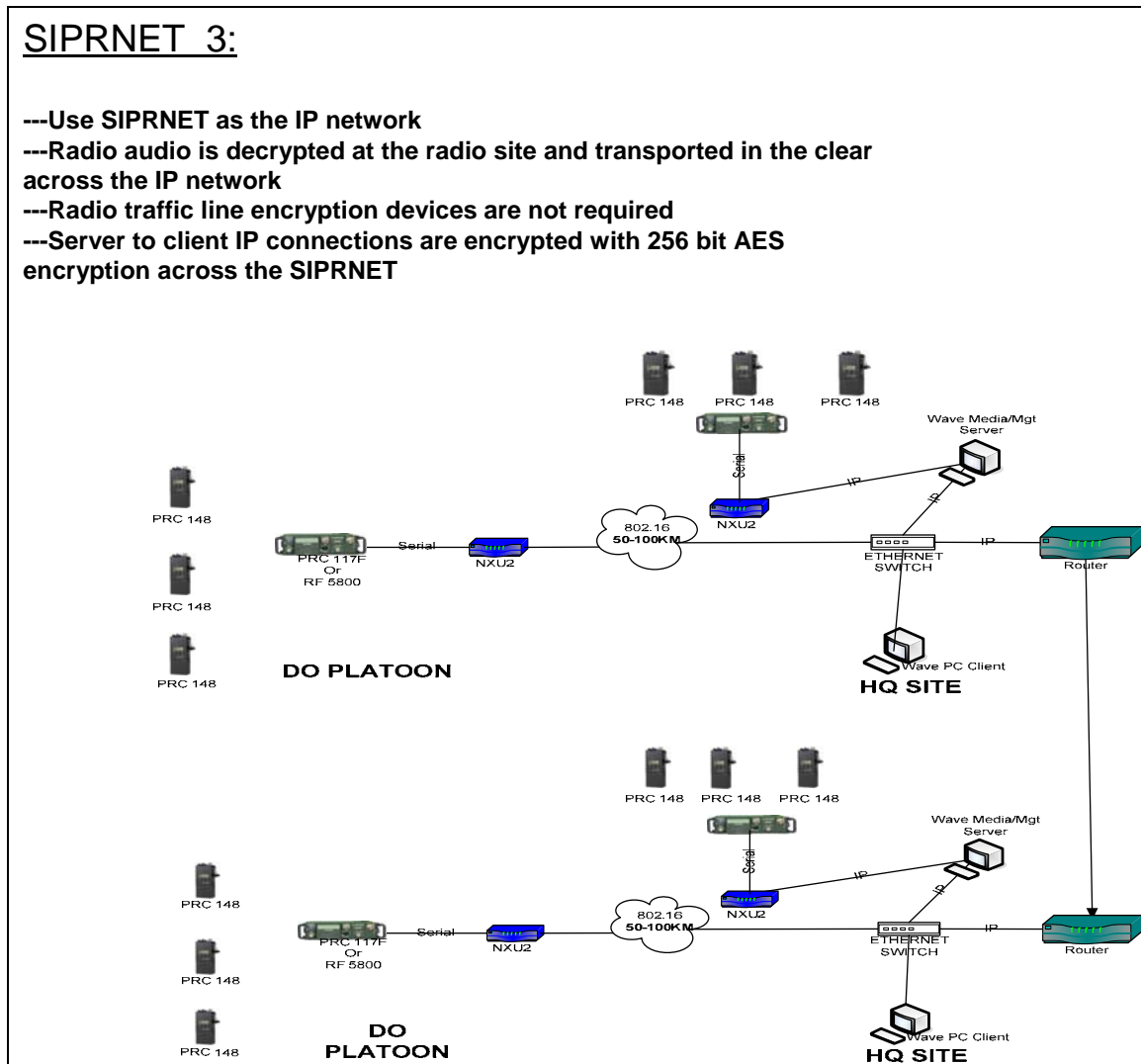
Diagram 10. SIPRNET Encryption Option Three
