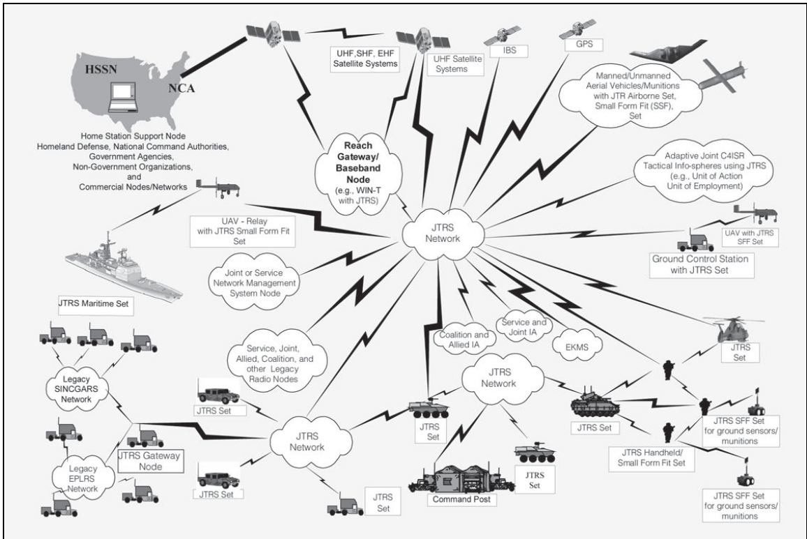
Figure 13. JTRS Operational Overview (From: [19])
