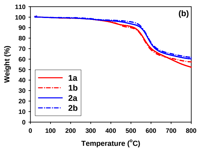
Figure 4. TGA thermograms for hyperbranched PEK's with heating rate of 10 °C/min.
