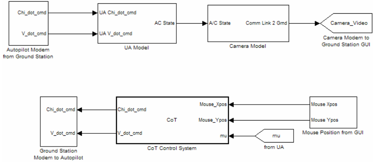
Figure 12. COT Concept with realistic subsystem divisions in Simulink
