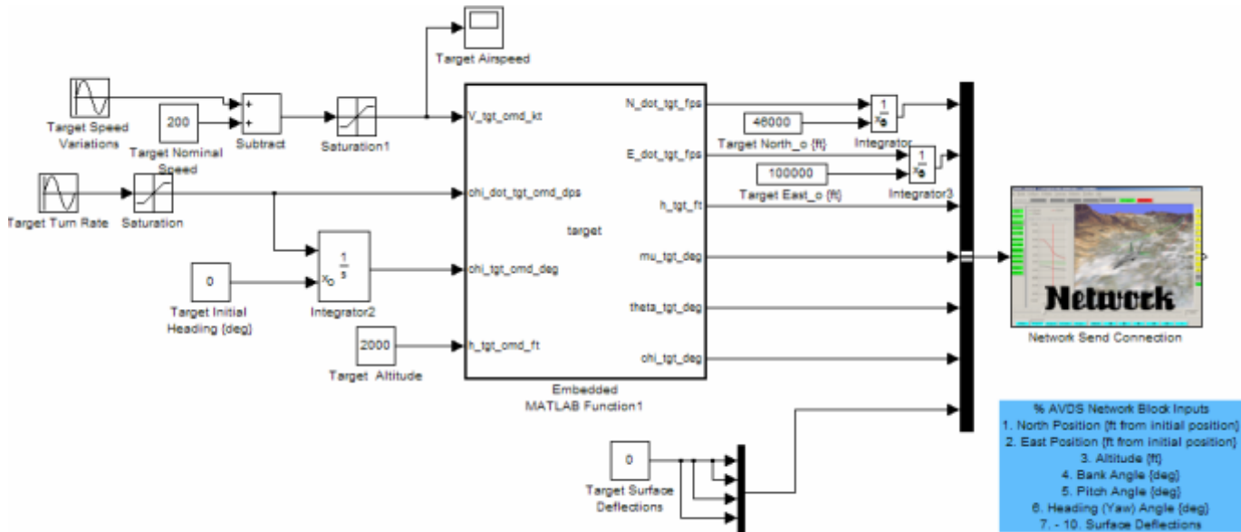
Figure 15. Target Model in Simulink
