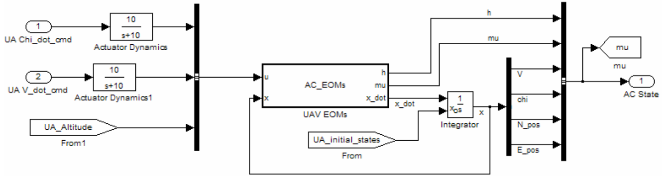
Figure 14. UA Model in Simulink
