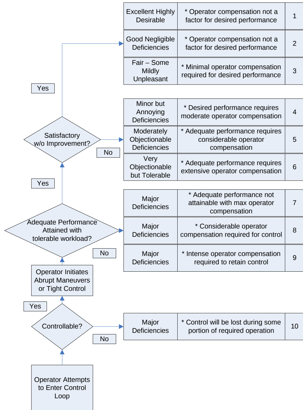
Figure 17. Proposed UAS Operator Rating Scale
