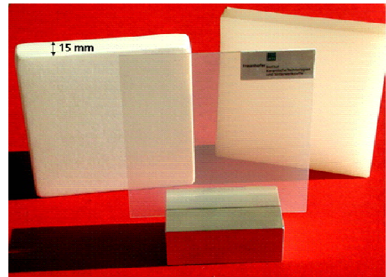
Figure 5b: High transparency of sintered sub- \mu\text{m} \text{Al}_2\text{O}_3 with real in-line transmission \sim 60\% at 0.8\text{ mm} thickness (central sample). The same material is translucent at larger thickness (right), it becomes white (opaque) when the residual porosity is 0.1\text{--}0.5\% (left).
