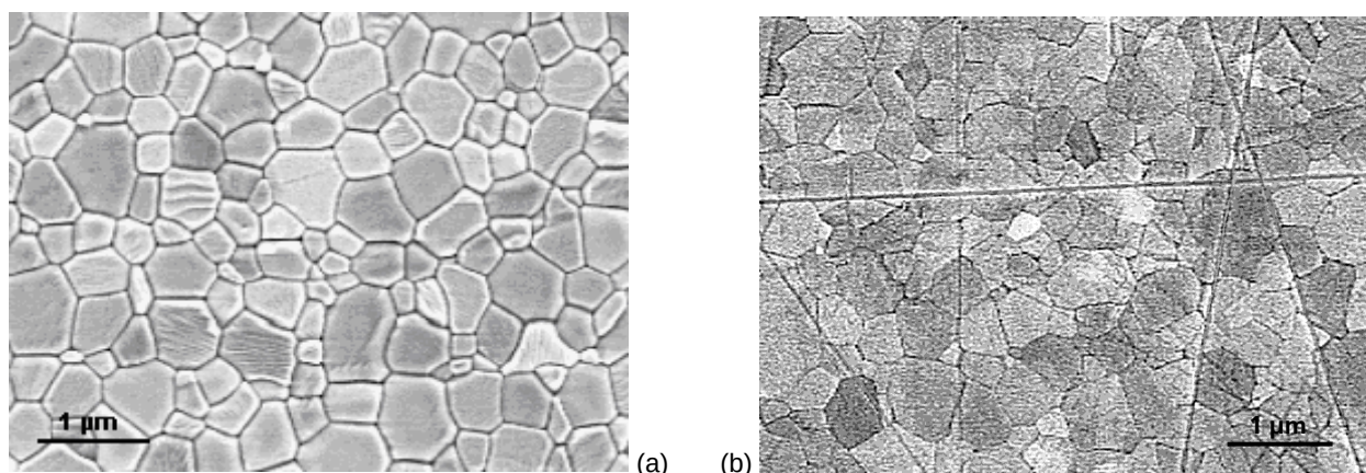
Figure 4: Microstructures of (a) transparent \text{Al}_2\text{O}_3 after HIP 1200 °C and of (b) spinel HIP-ed at 1260 °C.
