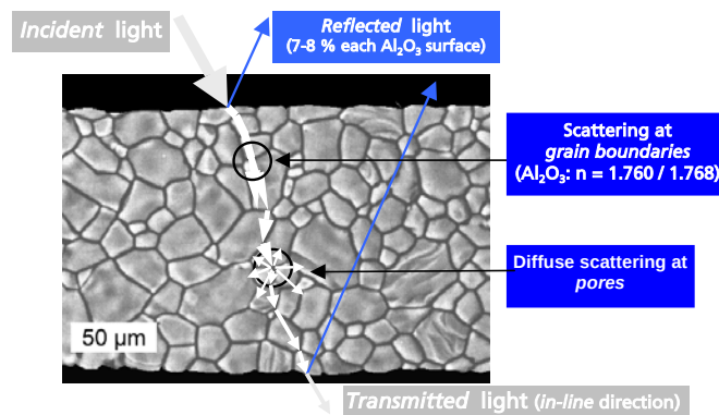
Figure 1: Light transmission through polycrystalline alumina ( \text{Al}_2\text{O}_3 ; example: coarse [translucent] grade).
