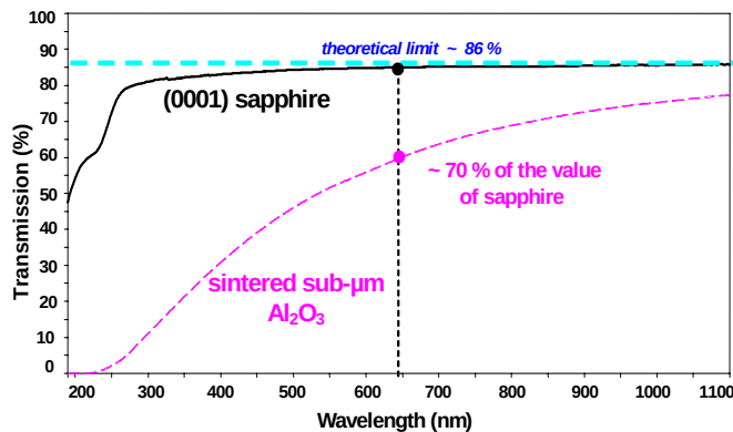
Figure 5a: Strong dependence of transmission through sintered sub- \mu\text{m} \text{Al}_2\text{O}_3 on the wavelength [2] - another consequence of the strong grain size effect displayed in Fig. 2b. The results are given for 0.8\text{ mm} thickness.
