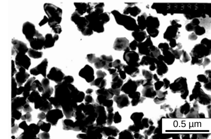
Commercial powder ~ 200 nm
