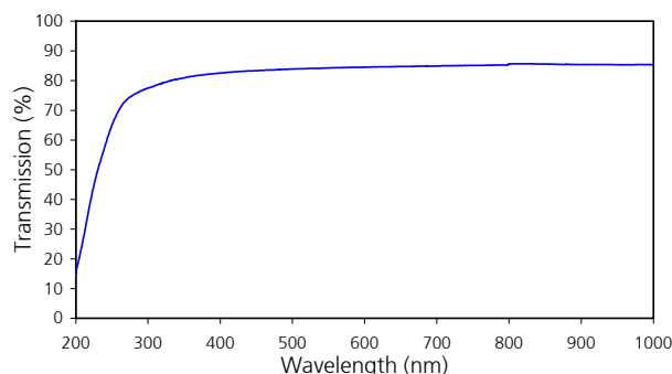
Figure 6a: Small dependence of transmission through sintered sub- \mu\text{m} spinel on the wavelength in the visible range (data for 0.94\text{ mm} thickness).
