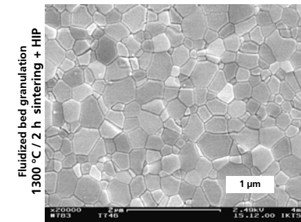
grain size 410 nm (relative density > 99.95 % [!])
