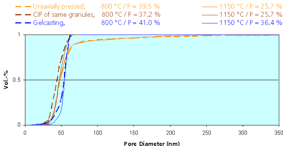
Figure 3: Pore size distributions of \text{Al}_2\text{O}_3 bodies formed by different shaping approaches from an \text{Al}_2\text{O}_3 powder with particles of about 150-200 nm.
