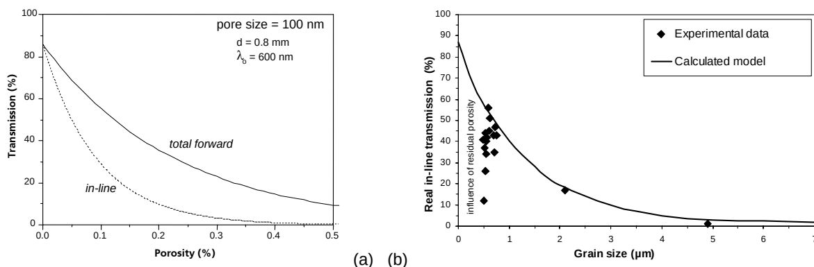
Figure 2: Influences of porosity and grain size on the light transmission through \text{Al}_2\text{O}_3
