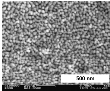
Nanocorundum powder 40 nm
