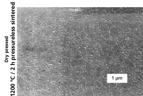
grain size 250 nm (relative density 97.0 % [!])
