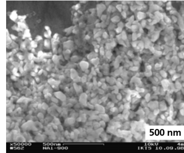
Nanocorundum powder 80 nm
