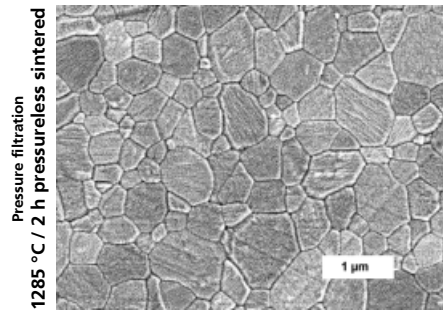
grain size 600 nm (relative density 99.1 %)
