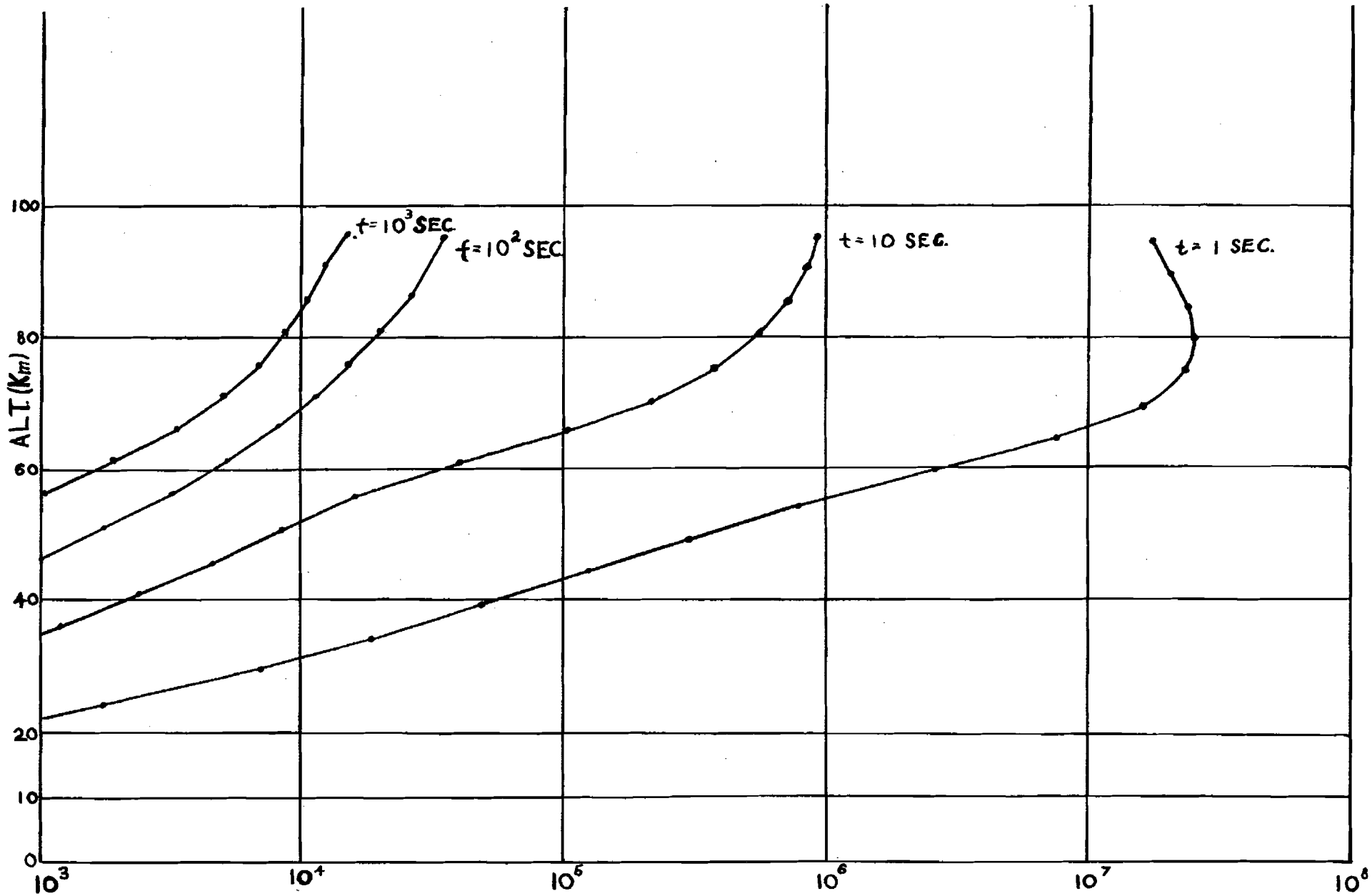
ELECTRON DENSITY ( e/cm^3 ) \beta + \gamma INDUCED ELECTRON DENSITIES FIG. 8 (S) RD II-23
