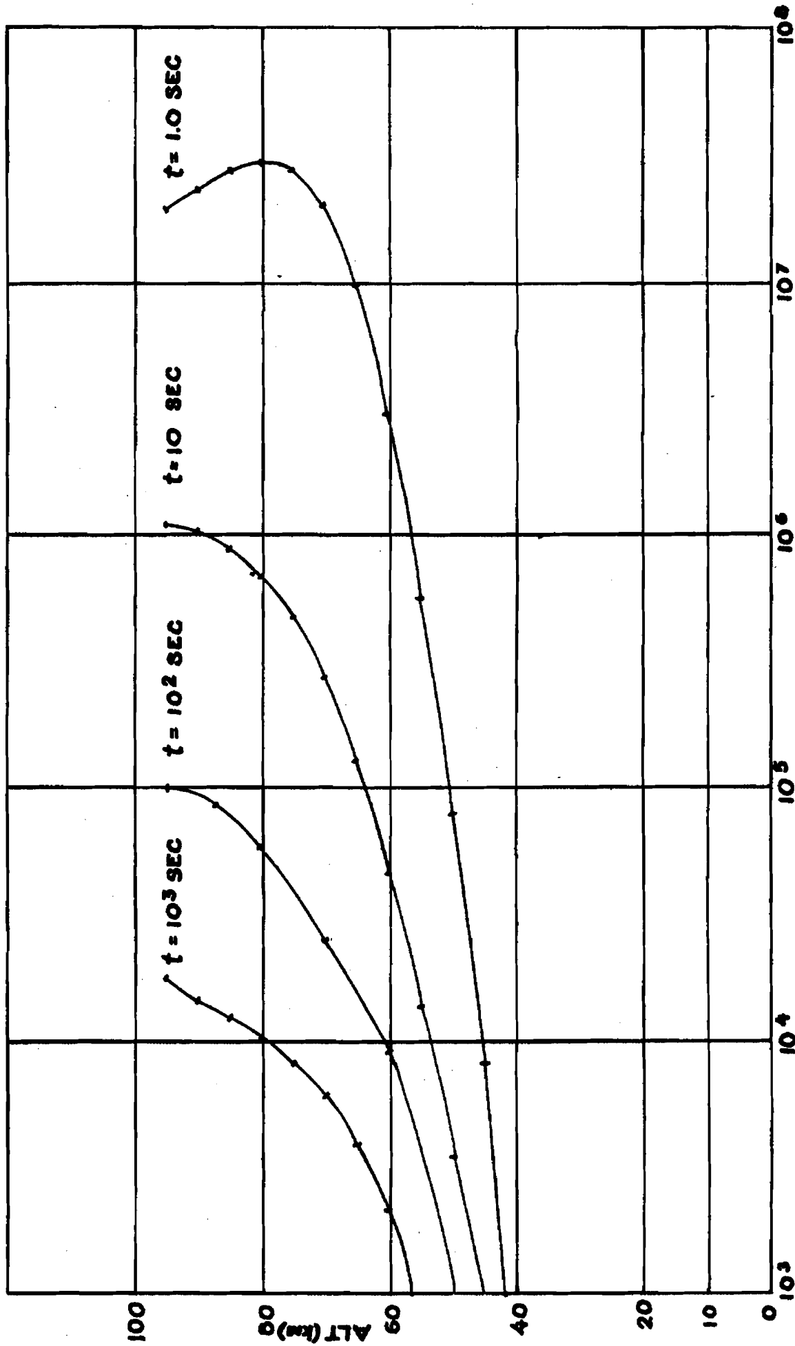
FIG. 10 ELECTRON DENSITY ( e/cm^3 ) INDUCED ELECTRON DENSITIES
