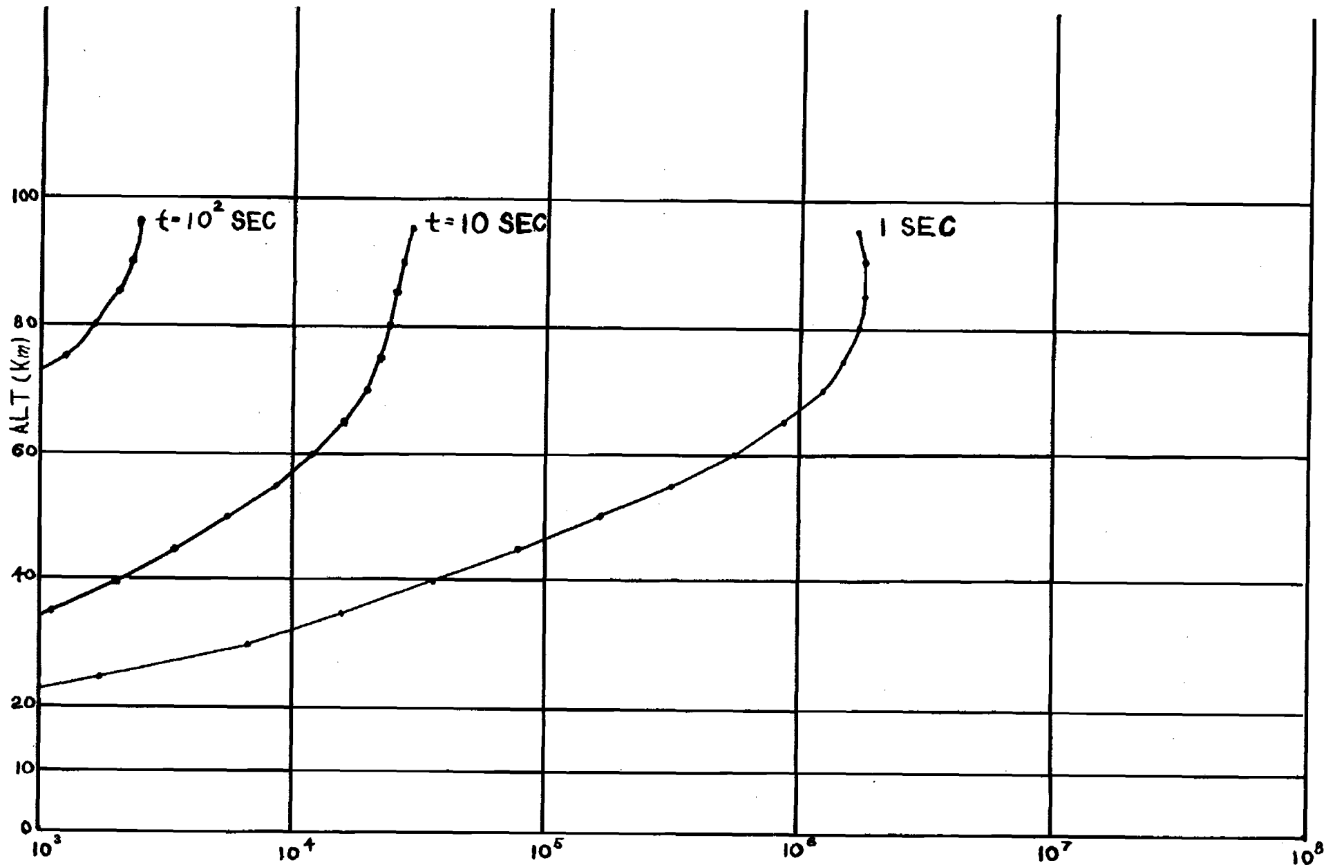
ELECTRON DENSITY ( e/cm^3 ) & INDUCED ELECTRON DENSITIES
