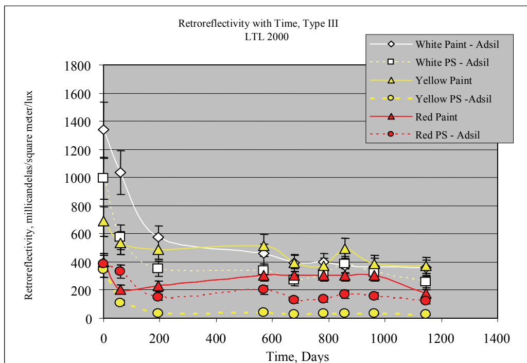
Figure 11. Retroreflectivity of Type III beads measured by the LTL-2000 retroreflectometer for Test 2 at Tyndall AFB. Note that the Adsil™ coating was applied prior to the data point near 200 days of service.
