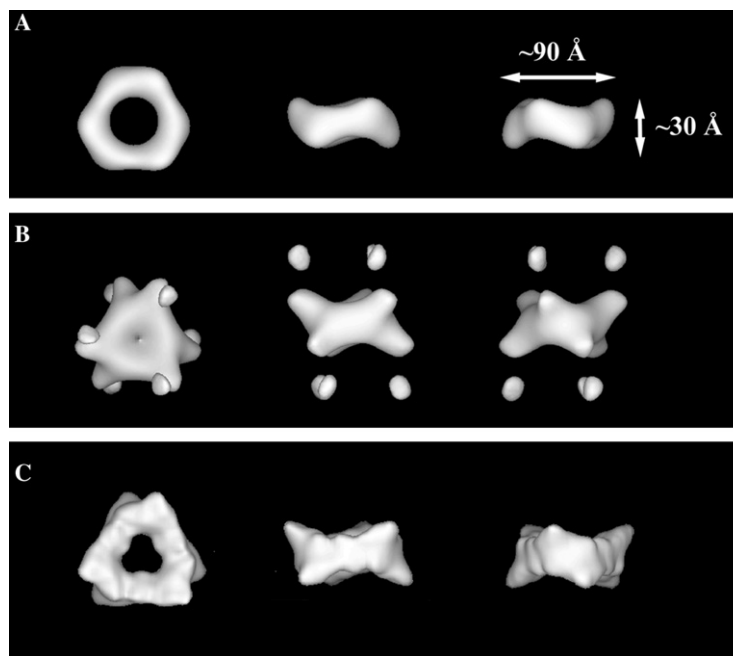
Fig. 2. EM reconstruction of truncated (31–212) and full-length (31–326) VP40. The left column shows that top view of each EM reconstruction, the middle column was obtained by a 90^\circ rotation of the top view along the x -axis, and the right column is a 60^\circ rotation of the middle column along the y -axis. (A) The EM reconstruction of truncated hexameric VP40 at a resolution of \sim 30 Å reveals a pore-like structure formed by the oligomerization of the N-terminal domain. The pore-like structure has an outside diameter of \sim 90 Å, an inside diameter of \sim 30 Å, and a height of \sim 30 Å. The homodimers that comprise the pore-like structure have a width of 55 Å (adapted from Ruigrok et al., 2000). (B) The EM reconstruction of the nearly full-length hexameric VP40 refined to \sim 30 Å shows that the C-terminal domain alternates between positions above and below the pore-like structure. The C-terminal domain is responsible for membrane-binding. The lower electron density of the C-terminal domains relative to the N-terminal domains suggests that the C-terminal domains are conformationally flexible (adapted from Scianimanico et al., 2000). (C) The EM reconstruction of truncated hexameric VP40 refined to \sim 20 Å shows the surface features of the pore-like structure in greater detail. The donut-like shape of hexameric VP40 at \sim 30 Å decomposes to two triangles offset by \sim 30^\circ . Additionally, the circular channel at \sim 30 Å becomes a cloverleaf shape at \sim 20 Å. The side view of the pore-like structure shows a chair-like conformation.
