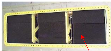
Figure 33. Spark-Initiated Combustion
