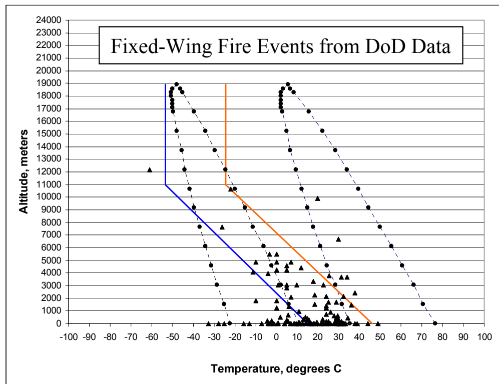
Figure 18 DoD Aircraft Fire Events vs. Flammability Profiles
