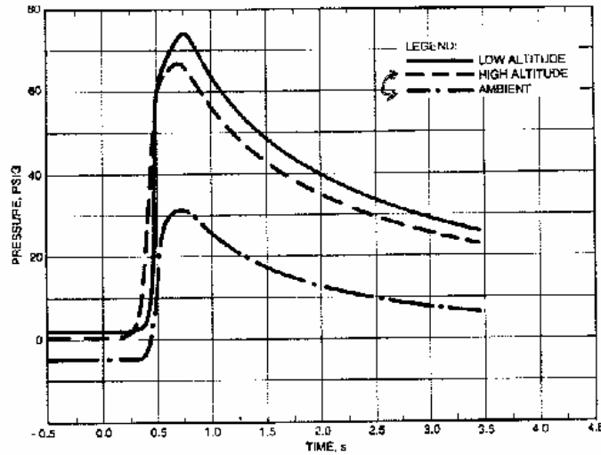
Figure 33. Spark-Initiated Combustion
