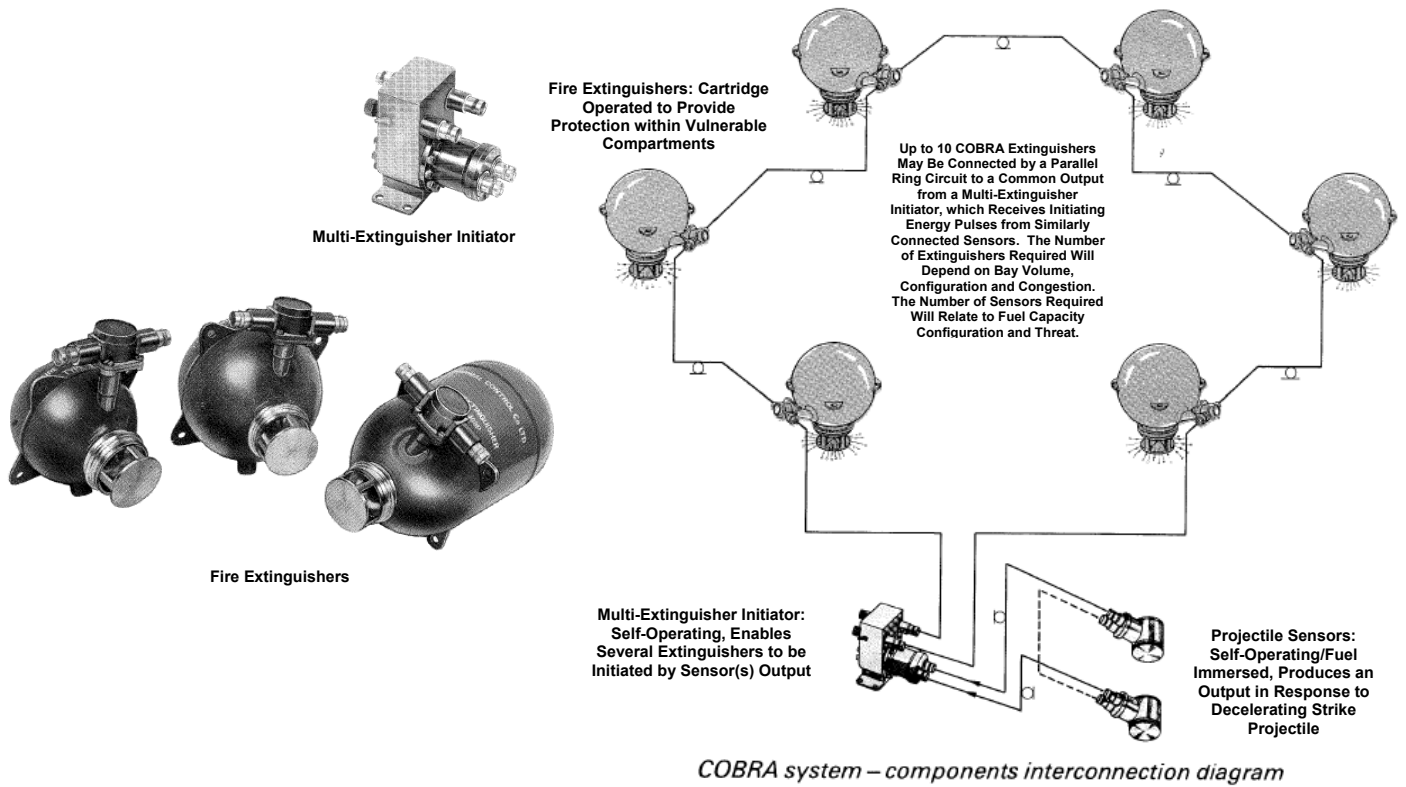
Figure 30. Non-DoD Aircraft Halon 1301 Dry Bay Fire Protection System [30, 31] (Reprinted with permission by Aircrew Limited, U.K.)
