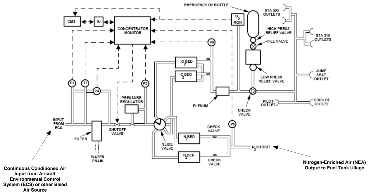
OBIGGS Schematic [33]
