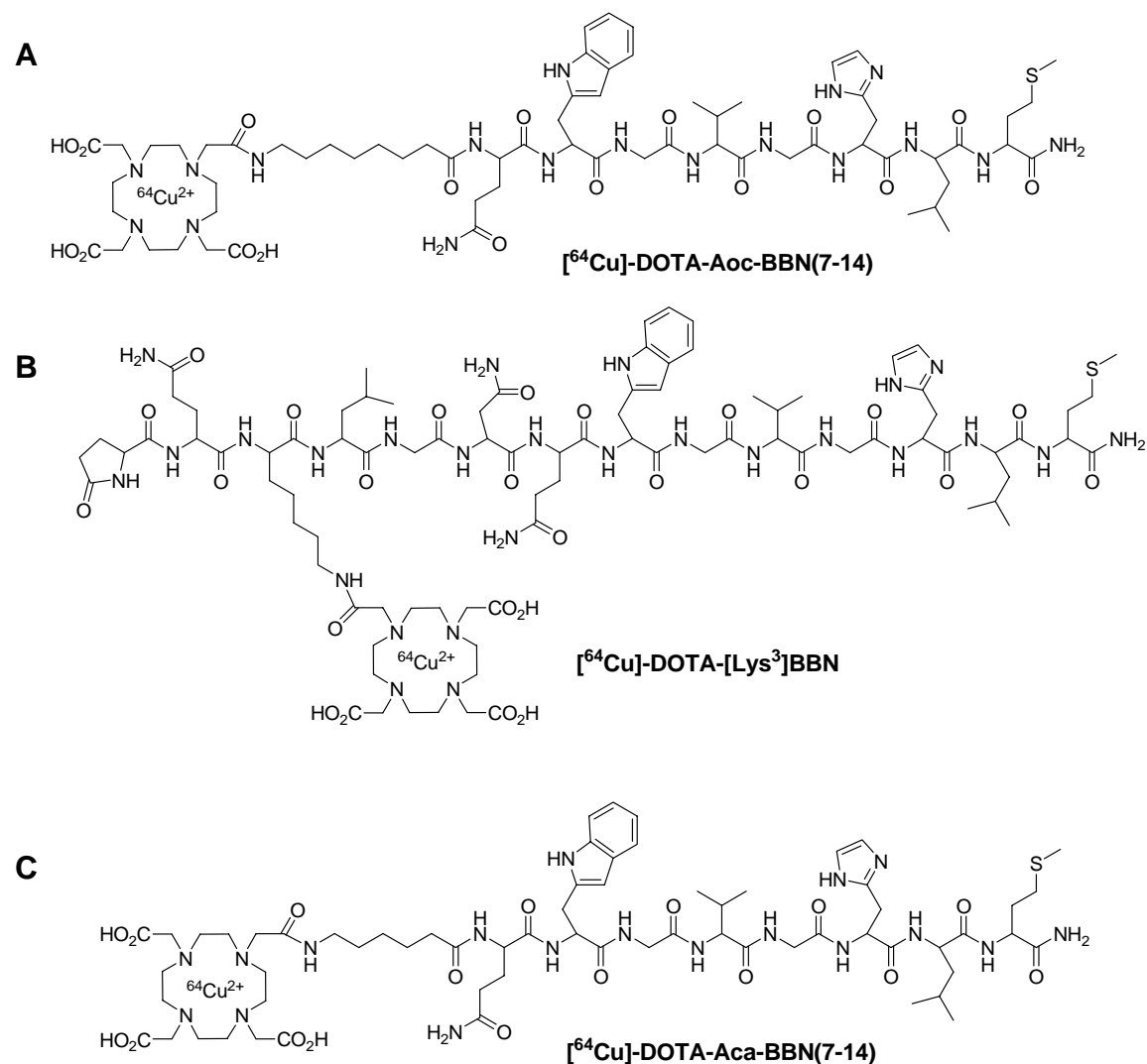
Fig. 1. Schematic structures of (A) [ 64 Cu]-DOTA-Aoc-BBN(7-14) [30] and (B) [ 64 Cu]-DOTA-[Lys 3 ]BBN and (C) [ 64 Cu]-DOTA-Aca-BBN(7-14).
