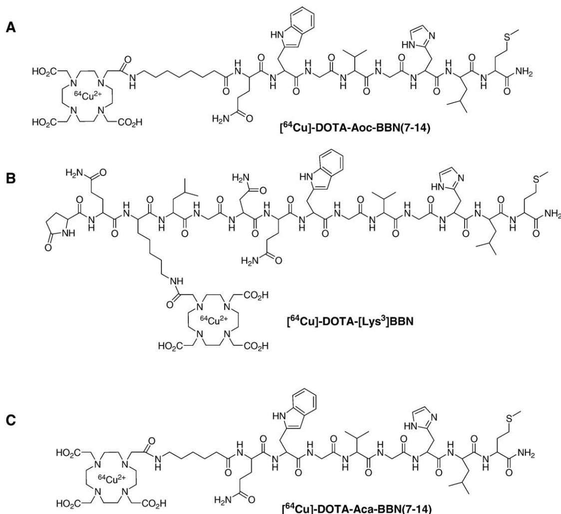
Fig. 1. Schematic structures of (A) [\text{}^{64}\text{Cu}]\text{-DOTA-Aoc-BBN(7-14)} [30], (B) [\text{}^{64}\text{Cu}]\text{-DOTA-[Lys}^3\text{]BBN} and (C) [\text{}^{64}\text{Cu}]\text{-DOTA-Aca-BBN(7-14)} .
