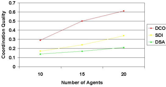
Figure 5: Role Allocation Simulations
