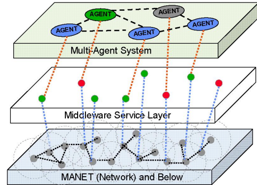
Figure 2: Layered Design Issues
