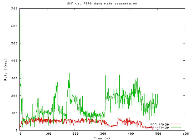
Figure 7: P2PS Middleware (unicast) vs. SMF pipes
