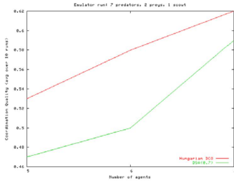
Figure 6: Early Simulation and Emulation Results
