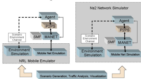
Figure 3: Example Modeling Approach
