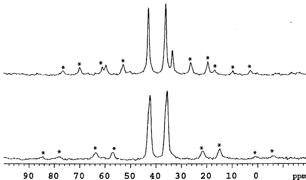
Figure 1. ^{13}C SSMAS NMR spectra of CEPS* on ambient C90 concrete: initial spectrum on bottom, 11-month spectrum on top. The * in the spectra designate the spinning side bands.
