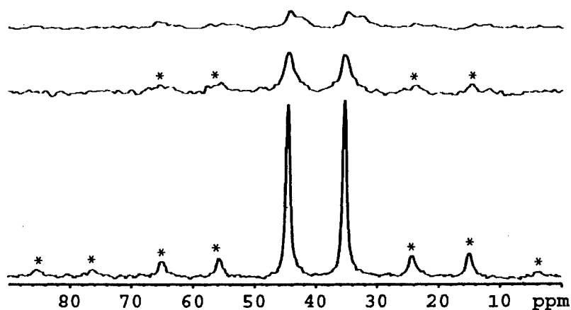
Figure 2. ^{13}C SSMAS NMR spectra of HD* on ambient C90 concrete; spectra in order from bottom to top were acquired at 1 hr, 14, and 39 weeks. The * in the spectra designate the spinning side bands.
