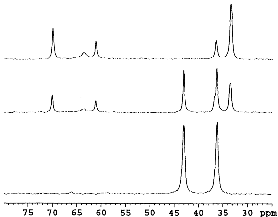
Figure 10. ^{13}\text{C} SS-MAS NMR spectra of CEPS* and water on concrete C03; spectra in order from bottom to top were acquired at 1 hr, 9 months, and the 9-month sample at 50^\circ\text{C} for 6 weeks.
