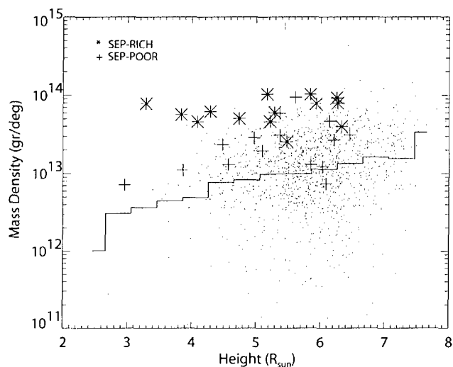
Figure 4. CME mass densities in grams per degree of angular width versus solar height in R_\odot . Dots are the 1996–2003 sample of 3462 CMEs with angular widths from 33^\circ to 132^\circ , and the lines show the averages per 0.4 R_\odot . Mass densities < 1.0e + 11 grams per degree are omitted from the plot. The SEP-rich and SEP-poor events are shown as * and + symbols.
