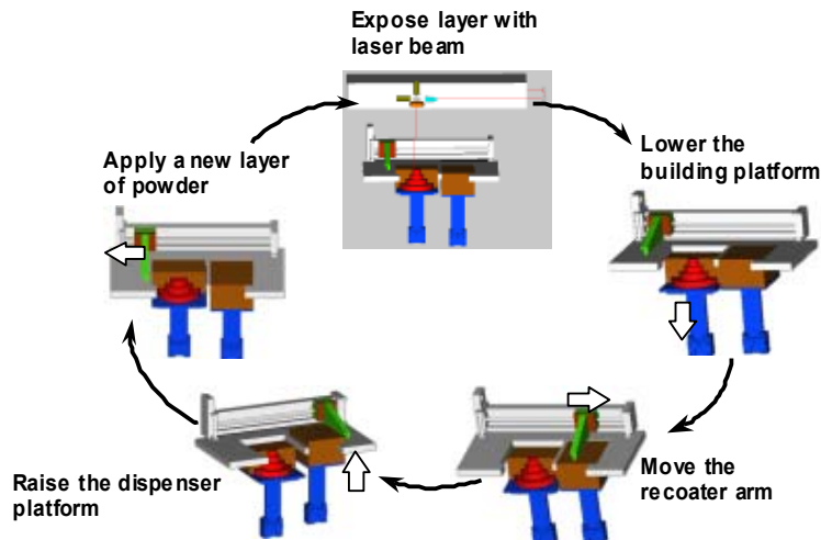
Figure B.4. DMLS operation sequence. (Courtesy EOS)
