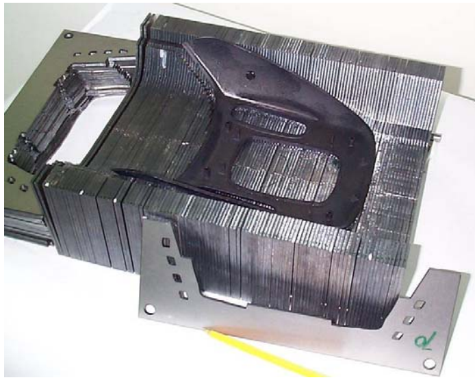
Figure B.26. Example of a laminated tool shown in a partially assembled state.
