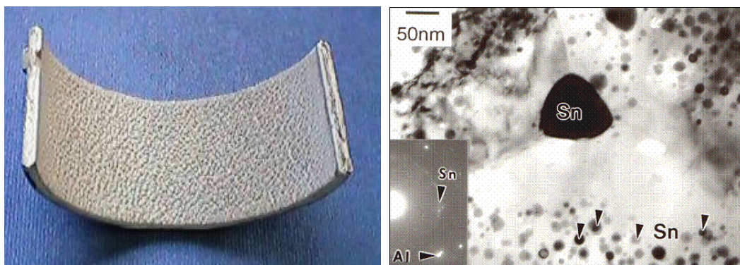
Figure B.28. Thermal spraying example.
