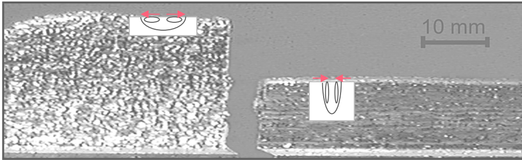
Figure 4.3. Laser-clad layers of 316L using gas-atomized particles ( left ) and water-atomized particles ( right ). The higher density structure ( right ) is attributed to reversal of Marangoni convection in the melt pool due to slightly different chemistry of the powder associated with the atomization method. The surface tension-driven convection is shown qualitatively in the inserts. (Courtesy Professor L. Li)
