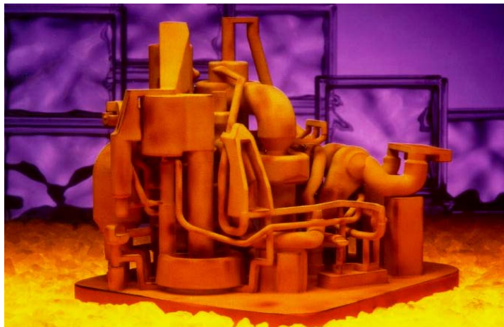
Figure 1.2. Complex SFF part created in a selective laser sintering process. (Courtesy 3D Systems)
