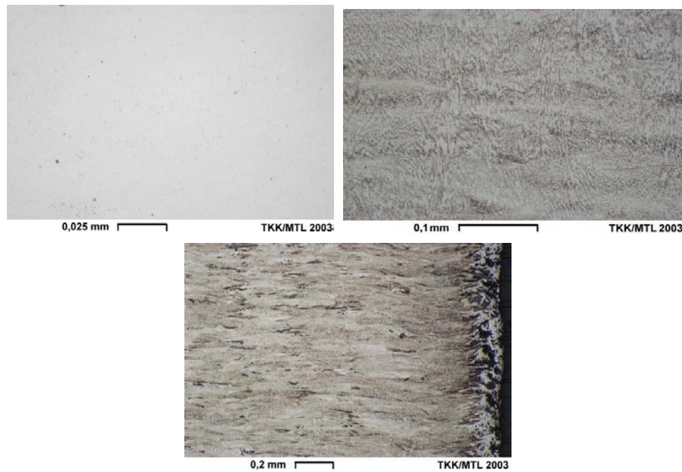
Figure B.6. Micrographs of DirectSteel H20 structure
