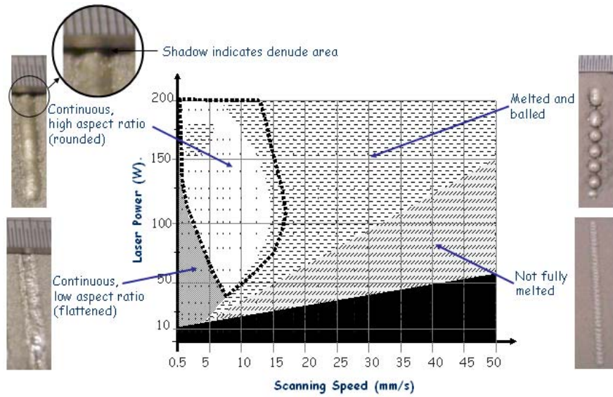
Figure 2.23. Typical process map showing the dependence of the metal melt zone morphology upon processing parameters such as laser power and scanning speed (Hauser, Childs, et al. 2003). The map indicates areas of undesirable melting, non-melting, bead-like flow, and flattened flow. The material is 314 HC stainless steel with a CO 2 laser spot size of 1.1 mm. (Courtesy Professor Childs)
