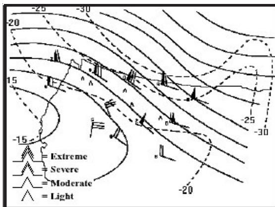
Figure 2-37. CAT in Thermal Troughs. CAT was reported from 28,000 to 37,000.
