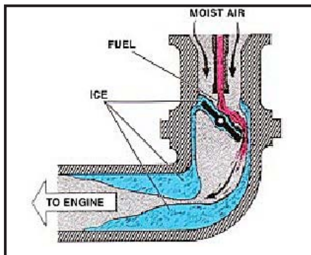
Figure 2-67. Carburetor Icing.
