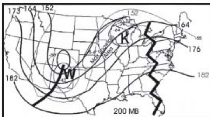
Figure 1-13. Snow Index (200-mb) Example. Determine amount of warm-air advection (difference between K and W) 64 - 42 = 22^{\circ}\text{C} . Divide by 2 for estimated snow amount (11 inches, in this case).
