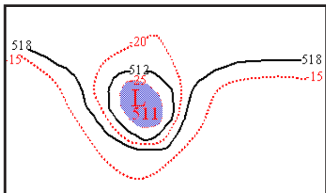
Figure 3-12. Barotropic Low.
