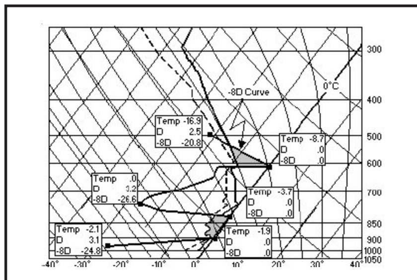
Figure 2-74. Example of -8\text{D} Method. The figure is a graphical presentation of the -8\text{D} method for forecasting icing.
