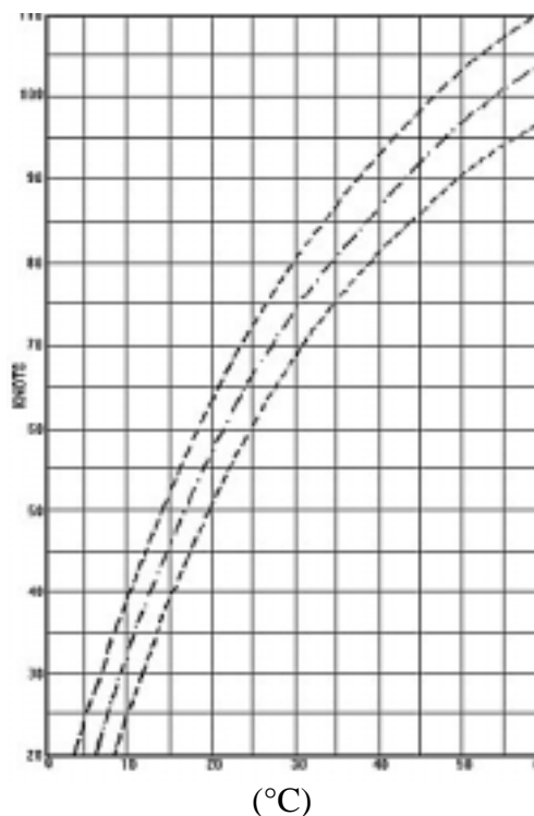
Figure 3-18. T2 Gust Computation Chart. See Step 6.
