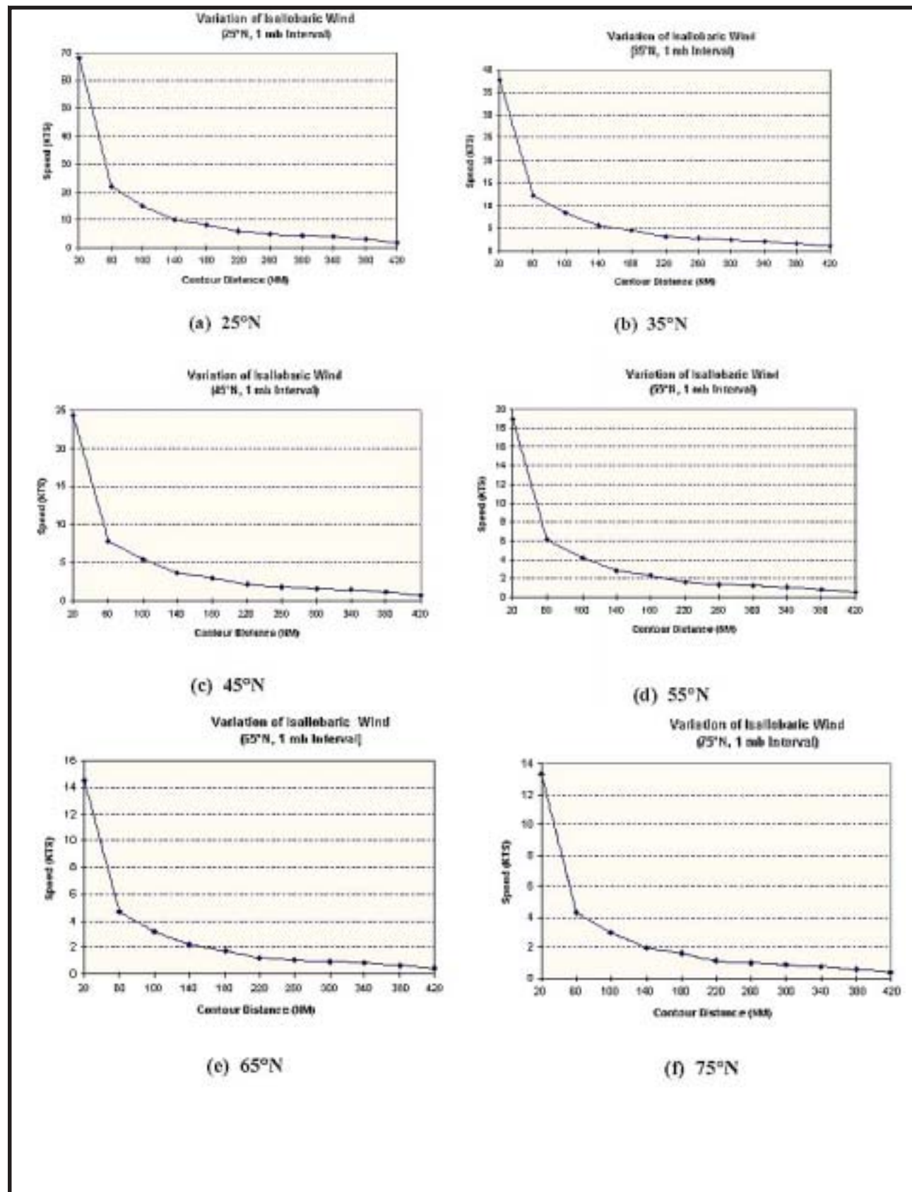
Figure 1-18a-f. Variation of Isallobaric Winds by Latitude.
