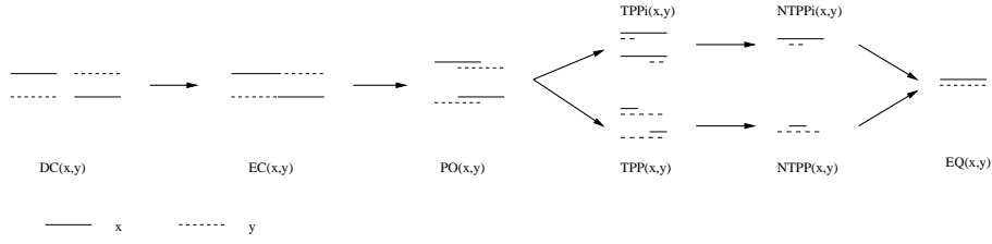
Figure 5. Geometric interpretations of \text{RCC}_1^8 relations between one-dimensional regions of a non-directed line.
