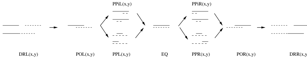
Figure 2. Possible geometric interpretations of the \text{RCC}_1^9 relations. For DRL, PPL, PPI, PPR, PPIR, and DRR two example configurations are given. One with and one without boundary intersection. The solid lines signify the interval x and dashed lines signify the interval y .
