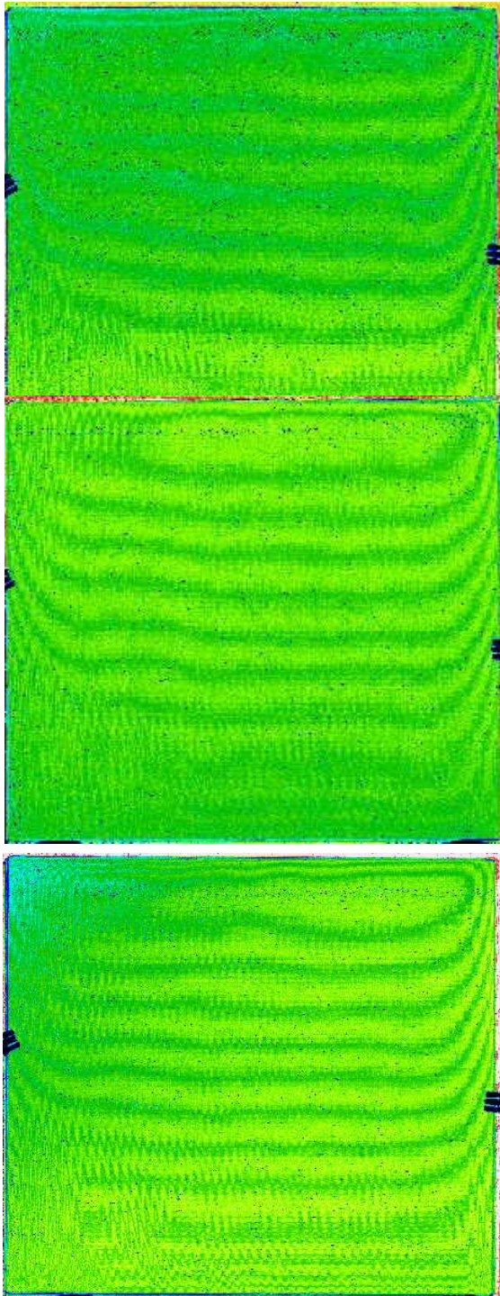
Figure 12 C-scan results for the three panels manufactured for preparation of the resin injection repair fatigue studies
