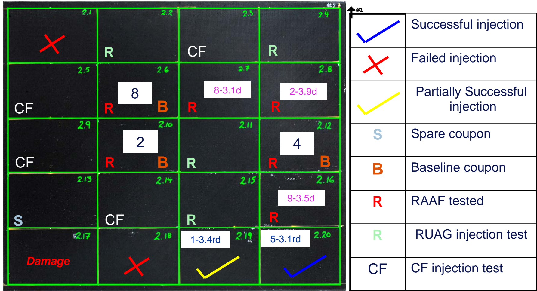
As manufactured Panel 2 with coupon locations identified. Numbers in white boxes represent baseline, bold black numeral, damaged, pink numeral with damage diameter and repaired test specimens, blue numeral with repaired damage diameter in inches. Numbers represent the fatigue resistance from worst (1) to best (7, 8 & 9).
