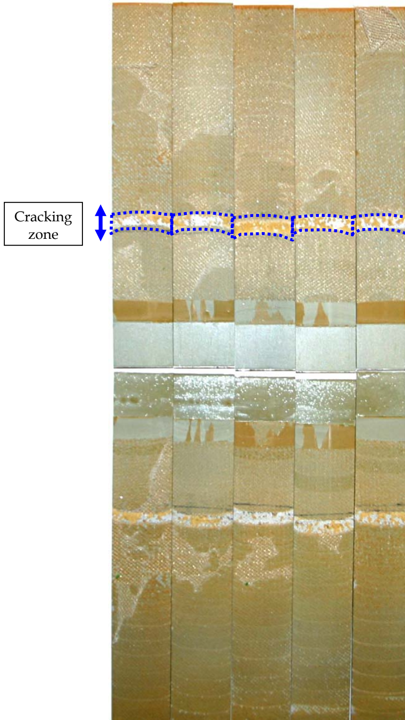
Al7075-T76 unclad aluminium treated with the grit blast and silane, primed with BR-127 and bonded with FM300-2K.
