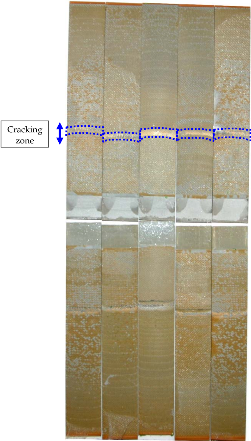
Al7075-T76 unclad aluminium treated with the grit blast and silane and bonded with FM300-2K.
