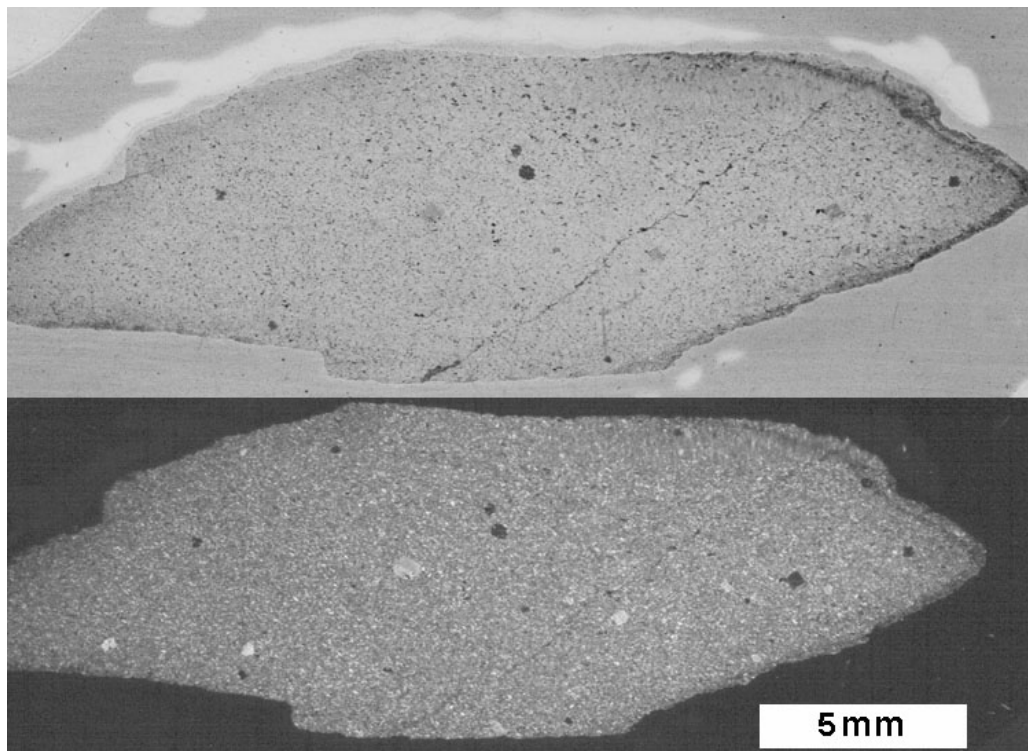
Figure 4.21. Artifact FBL072 (scanned thin section, plane-polarized light [top] and crossed polars [bottom]).
