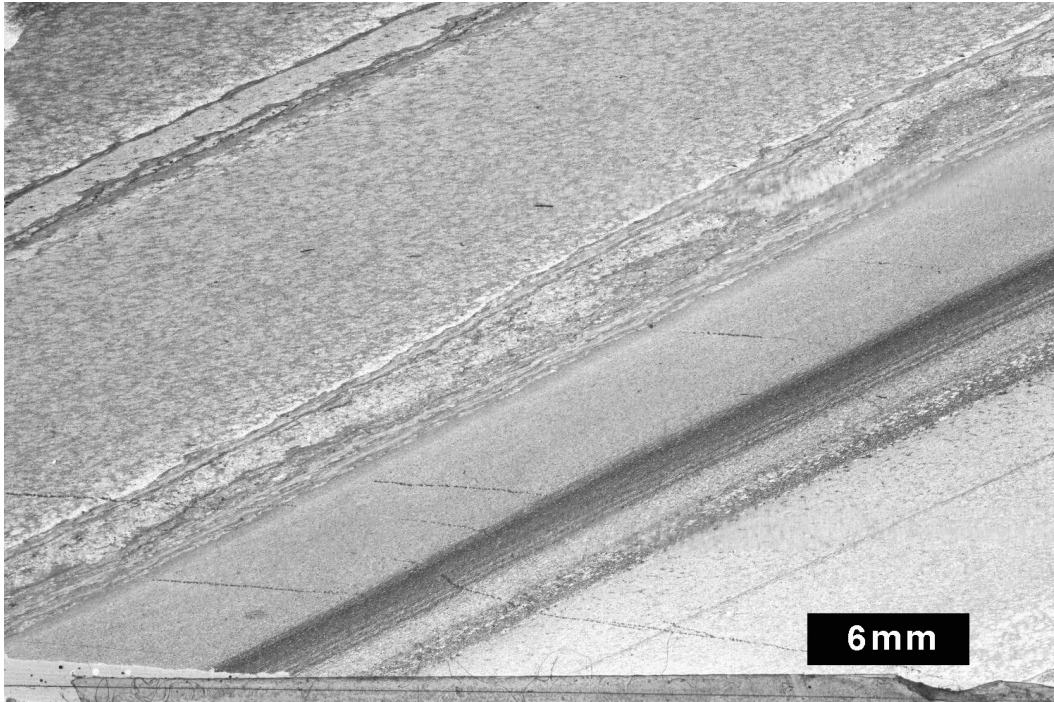
Figure 4.12. Chatham Pittsboro sample with fine laminae, grading, possible current ripples, and incipient cleavage (FBL028; scanned thin section, plane-polarized light).
