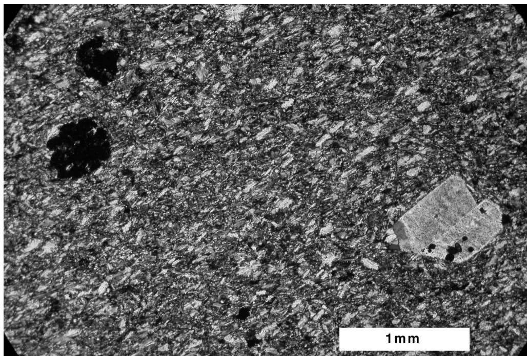
Figure 4.22. Groundmass lath alignment, plagioclase phenocryst, and garnet porphyroblasts in artifact FBL072 (crossed polars).
