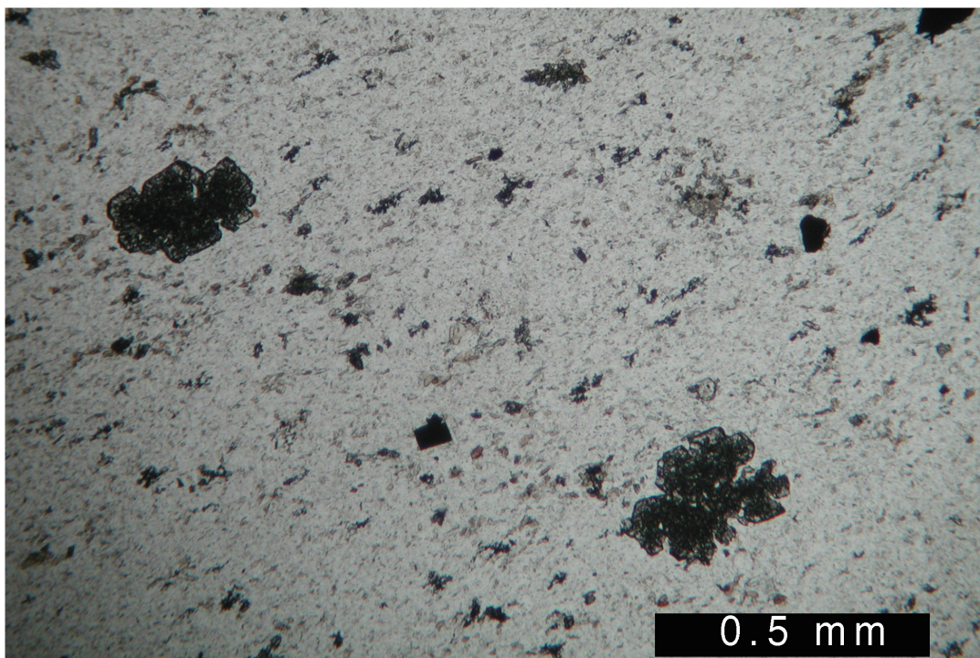
Figure 4.9. Garnet porphyroblasts in Uwharries Asheboro sample (FBL022; plane-polarized light).
