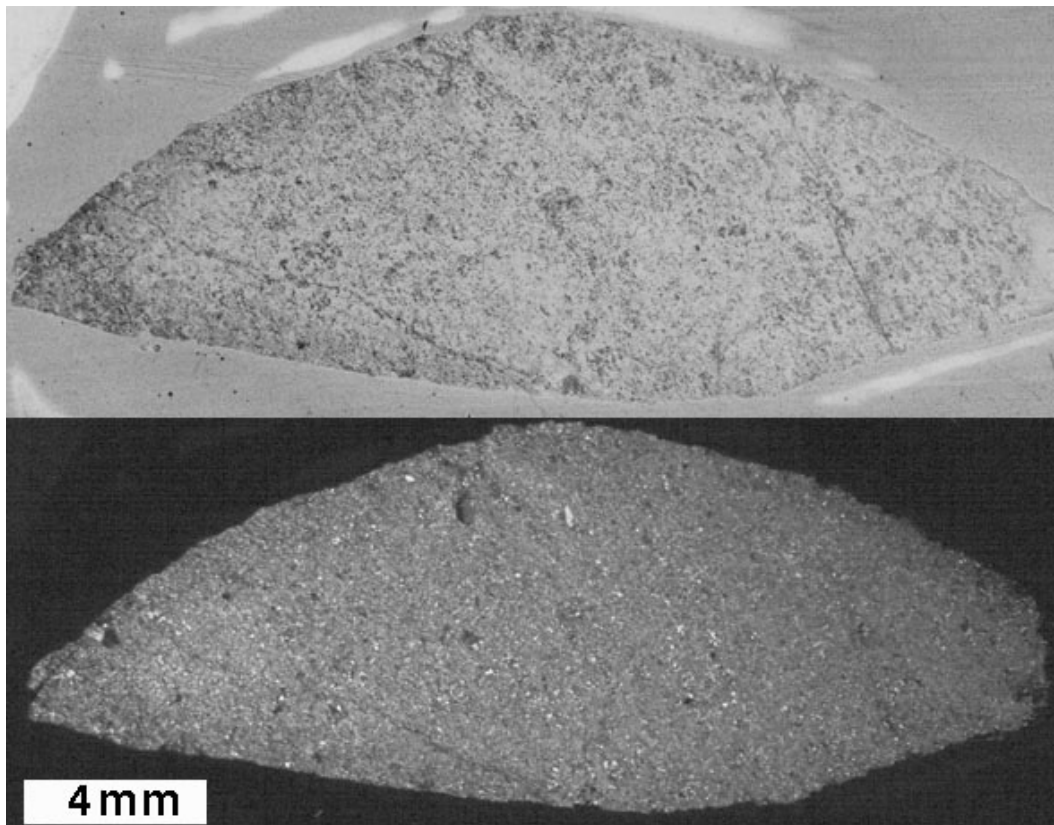
Figure 4.30. Artifact FBL079 (scanned thin section, plane-polarized light [top] and crossed polars [bottom]).
