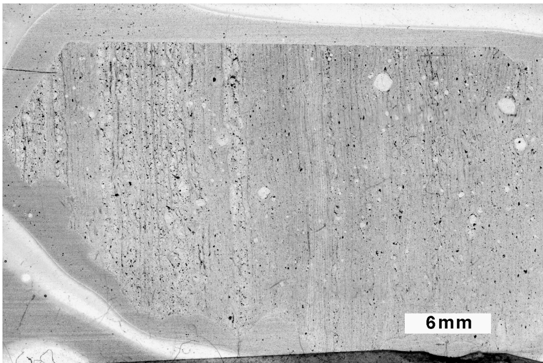
Figure 4.4. Strongly flow-banded dacite with quartz and plagioclase phenocrysts (FBL006; scanned thin section, plane-polarized light).
