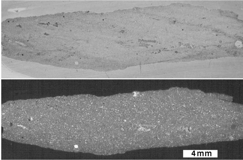
Figure 4.24. Artifact FBL074 (scanned thin section, plane-polarized light [top] and crossed polars [bottom]).
