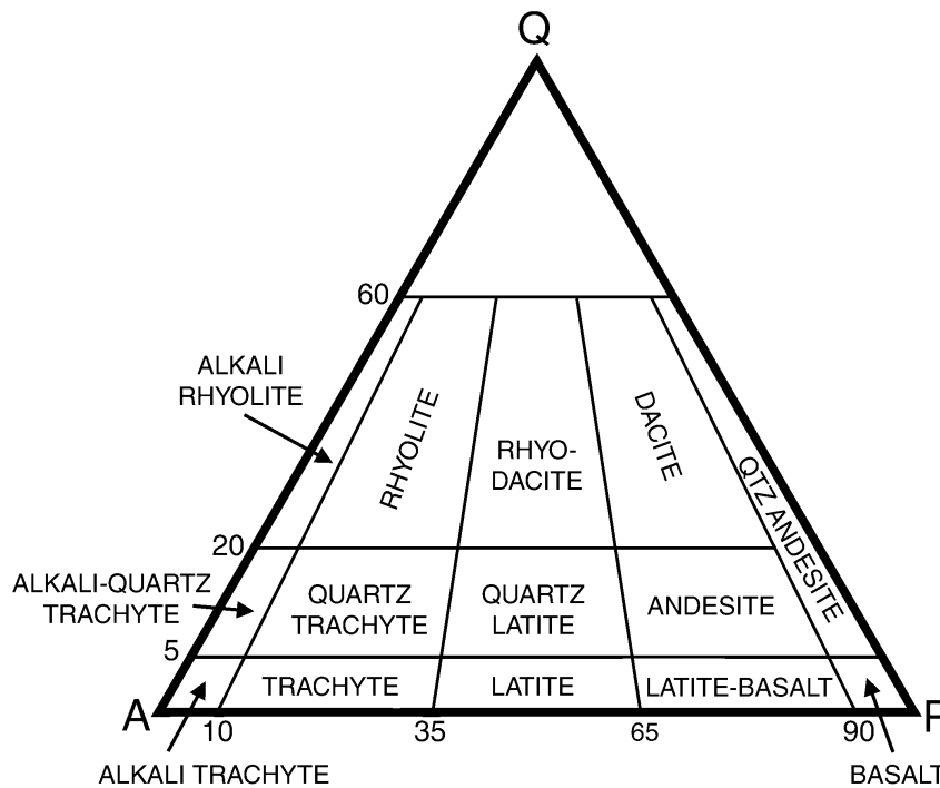
Figure 4.1. IUGS classification for volcanic igneous rocks (from Winter 2001).
