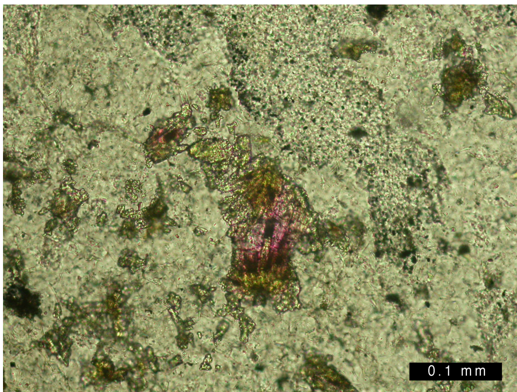
Figure 4.16. Piedmontite in groundmass of Chatham Silk Hope sample (FBL031; plane-polarized light). In color, this relatively rare mineral is bright pink and yellow pleochroic.
