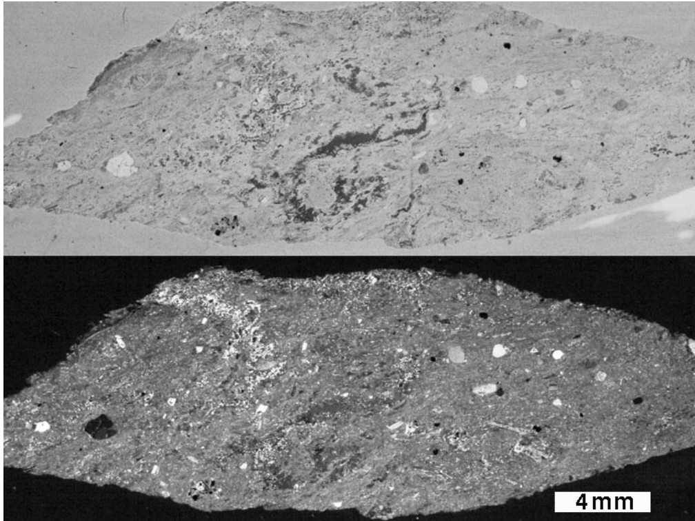
Figure 4.28. Artifact FBL078 (scanned thin section, plane-polarized light [top] and crossed polars [bottom]).
