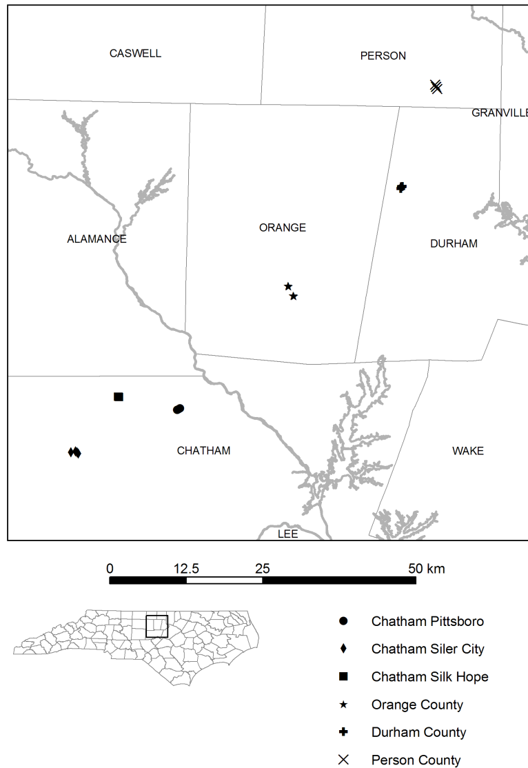
Figure 3.9. Quarry zones and sample locations in the northern portion of the study area.
