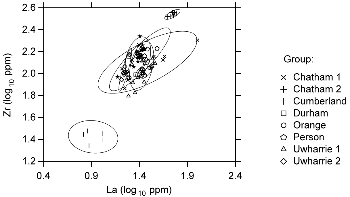
Figure 5.3. Bivariate plot of Zr versus La for the chemical groups. Ellipses represent 90% confidence level for membership in the groups. Artifacts are plotted as solid stars.
