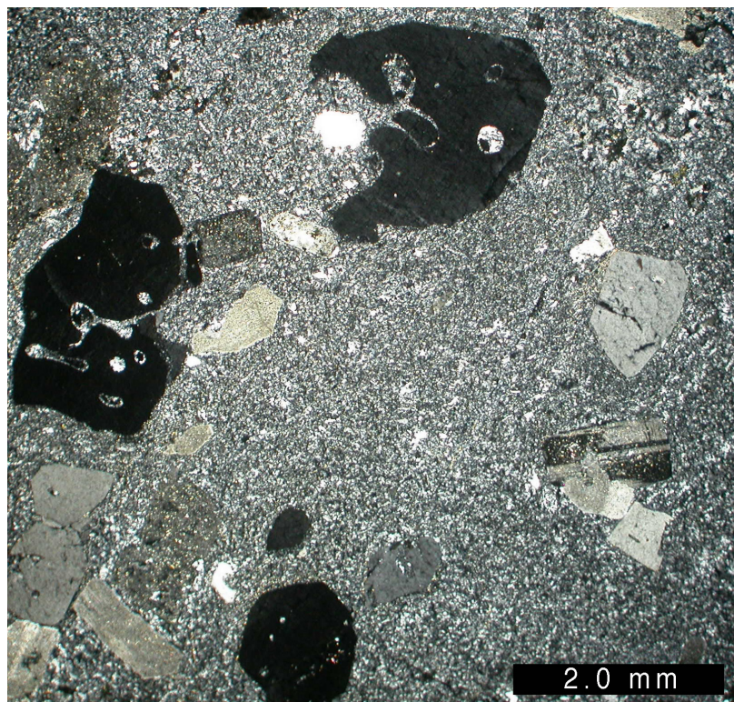
Figure 4.17. Euhedral and resorbed quartz phenocrysts, with plagioclase, in Orange County sample (FBL061; crossed polars).
