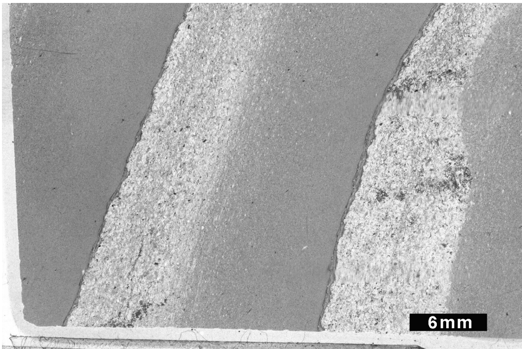
Figure 4.13. Chatham Pittsboro sample with graded bedding couplets (FBL029; scanned thin section, plane-polarized light). Stratigraphic younging direction is to the right.
