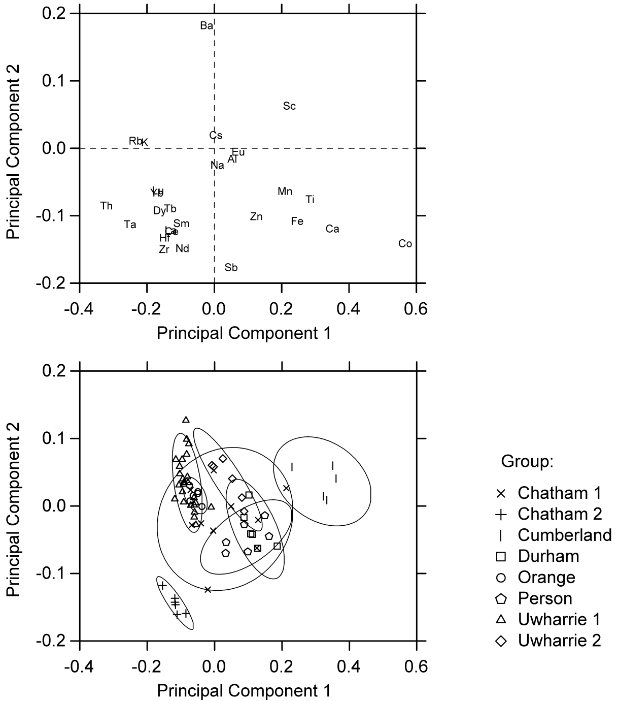
Figure 5.1. Biplot derived from PCA of the variance-covariance matrix of the NAA data showing principal component 1 versus principal component 2. Elements are shown in the top graph; analyzed specimens are shown in the bottom graph. Ellipses represent 90% confidence level for membership in the groups.
