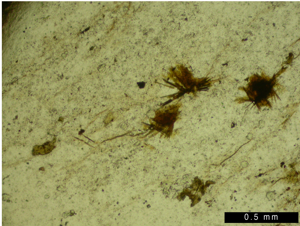
Figure 4.5. Metamorphic stilpnomelane (needle-like aggregates) in Uwharries Eastern sample (FBL005; plane-polarized light).
