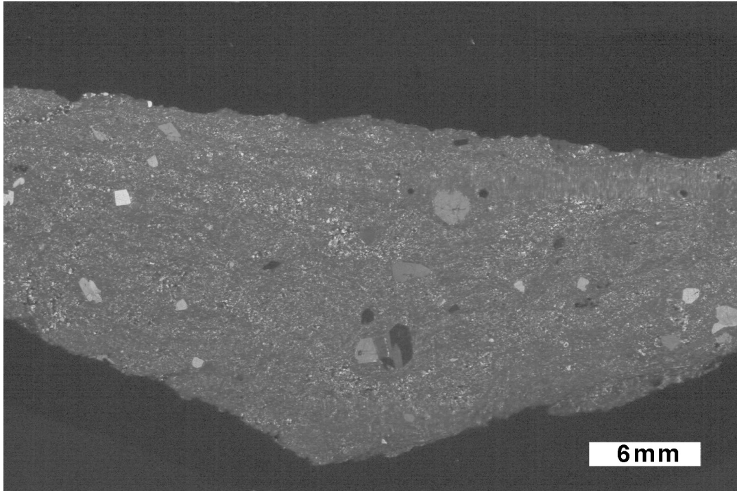
Figure 4.10. Uwharries Southeastern sample with quartz and plagioclase phenocrysts and weak banding (FBL052; scanned thin section, crossed polars).
