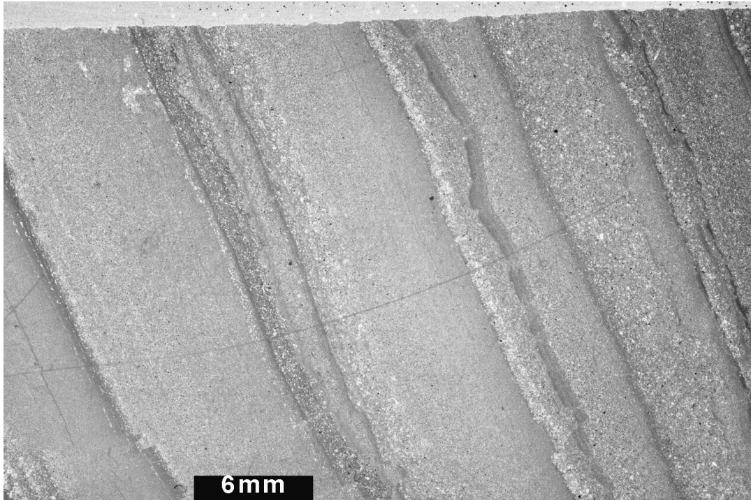
Figure 4.19. Person County sample with sedimentary laminae, grading (top to the right), and micro-faults (FBL046; scanned thin section, plane-polarized light).
