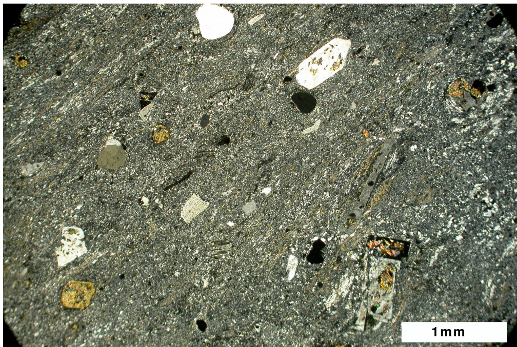
Figure 4.29. Weak alignment, phenocrysts, and pseudomorphs after amphibole or pyroxene (lower left and lower right) in artifact FBL078 (crossed polars).
