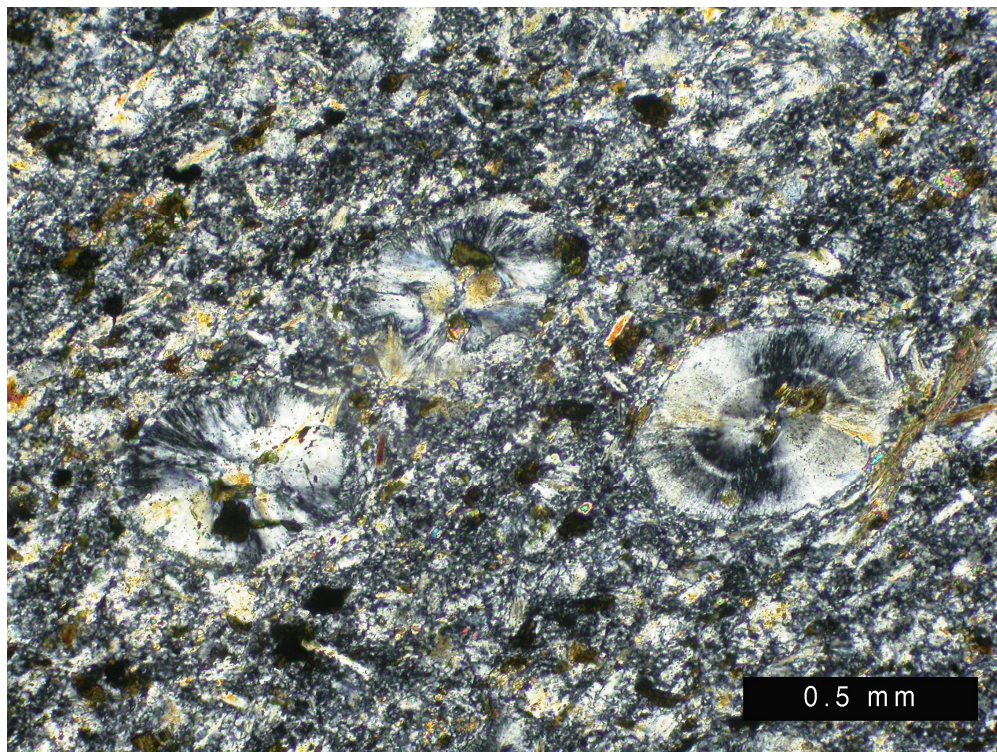
Figure 4.7. Uwharries Southern sample with spherulites (FBL017; crossed polars).
