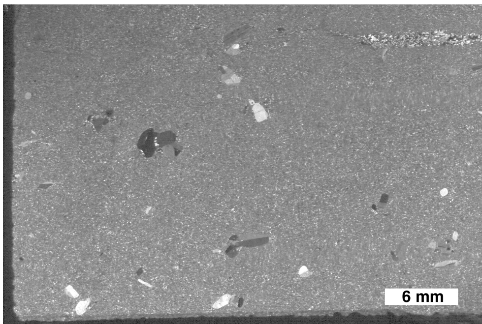
Figure 4.6. Uwharries Western sample with sparse plagioclase phenocrysts and fine groundmass (FBL010; scanned thin section, crossed polars).
