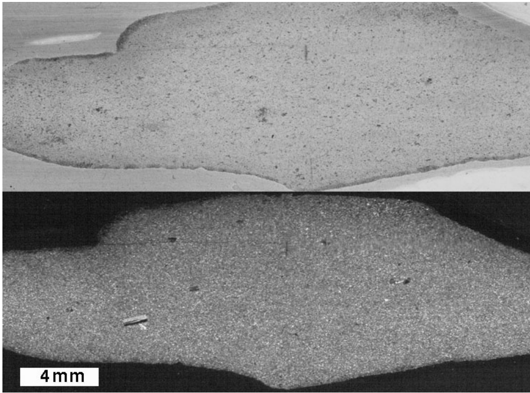
Figure 4.31. Artifact FBL080 (scanned thin section, plane-polarized light [top] and crossed polars [bottom]).
