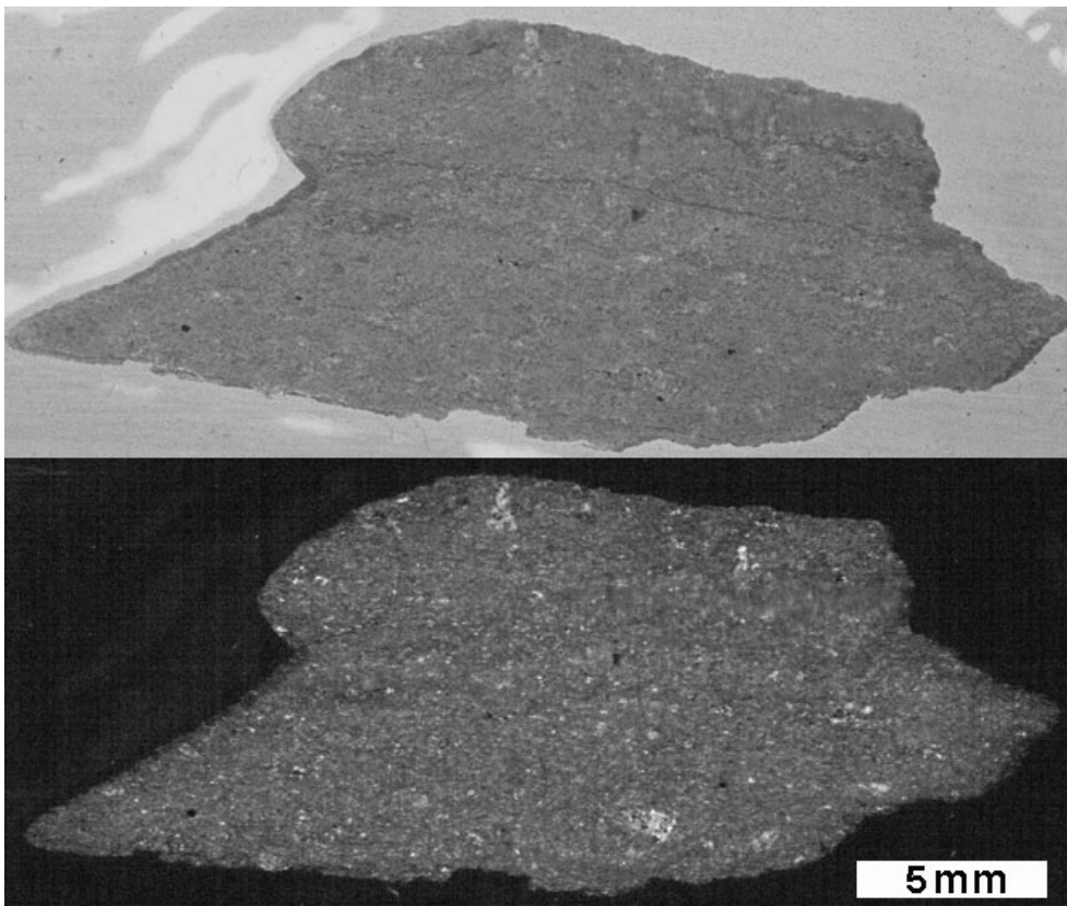
Figure 4.25. Artifact FBL075 (scanned thin section, plane-polarized light [top] and crossed polars [bottom]).
