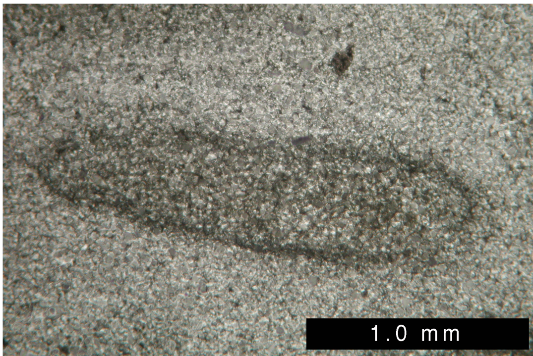
Figure 4.20. Elliptical feature (perhaps a trace fossil?) in metasiltsone from Person County (FBL045; plane-polarized light).
