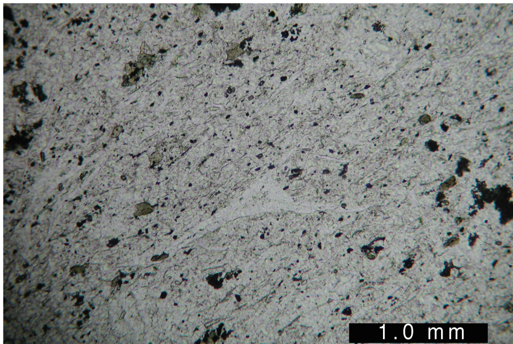
Figure 4.15. Y-shaped glass shard in Chatham Silk Hope sample (FBL031; plane-polarized light).
