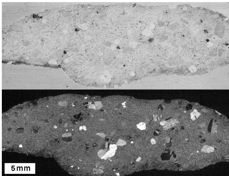
Figure 4.23. Artifact FBL073 (scanned thin section, plane-polarized light [top] and crossed polars [bottom]). Note euhedral and resorbed quartz phenocrysts and crystal-rich texture.
