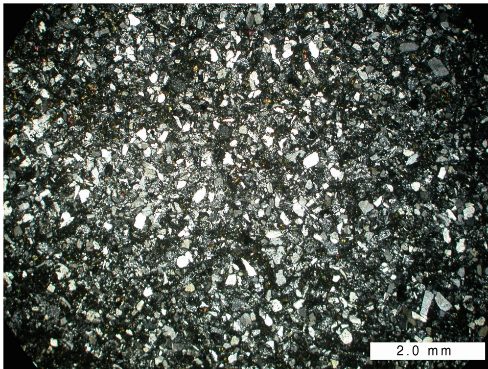
Figure 4.18. Durham County volcanic sandstone with clastic texture (FBL067; crossed polars).
