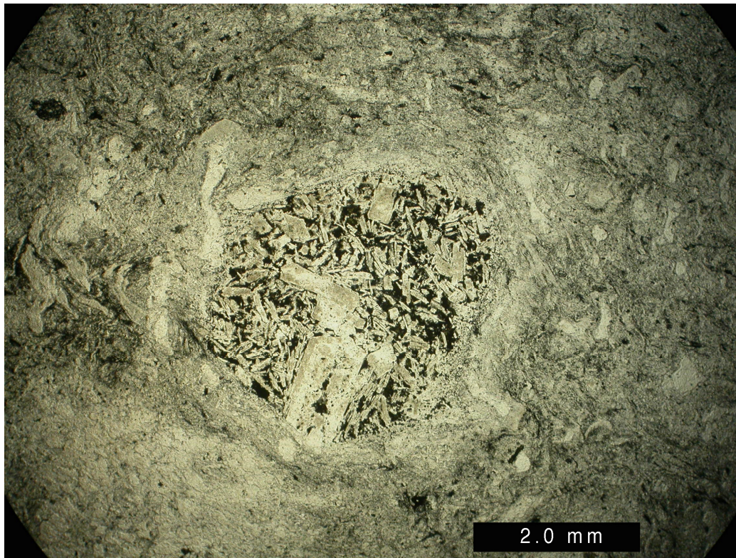
Figure 4.14. Basaltic fragment in Chatham Silk Hope sample (FBL034; plane-polarized light).
