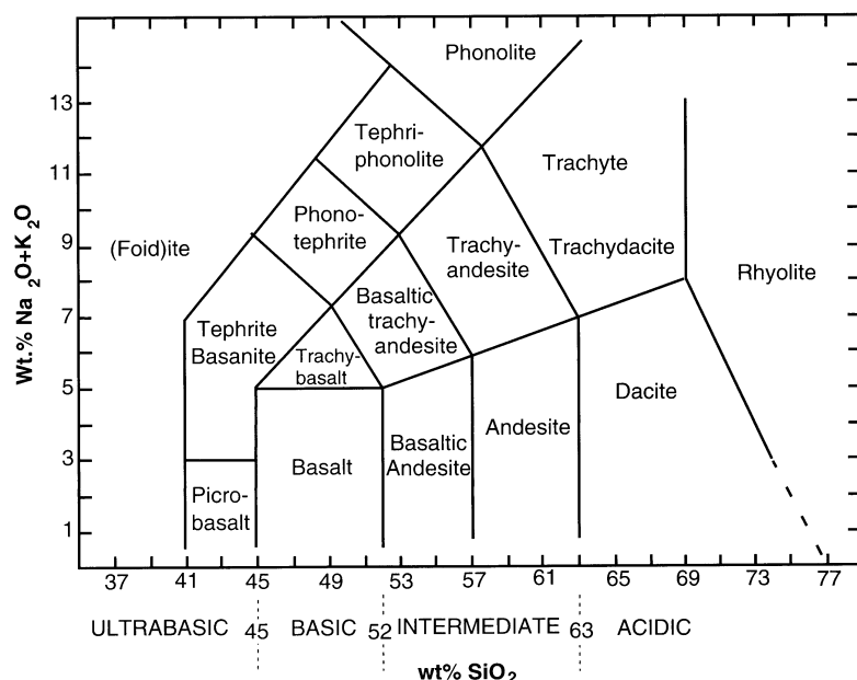
Figure 4.2. Total alkalis versus silica (TAS) classification of volcanic rocks (LeMaitre 1989).
