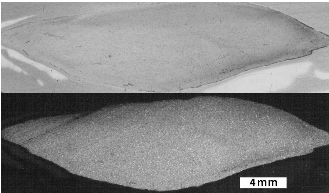
Figure 4.27. Artifact FBL077 (scanned thin section, plane-polarized light [top] and crossed polars [bottom]). Parallel lines are saw marks.
