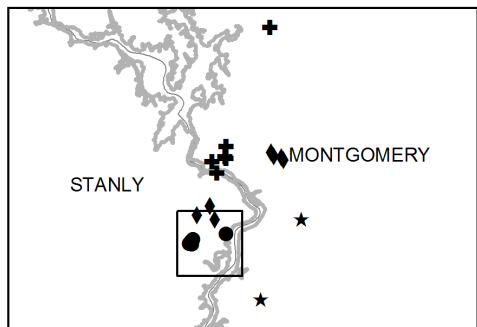
Figure B.2. Sample locations in the Uwharries Southern zone.
