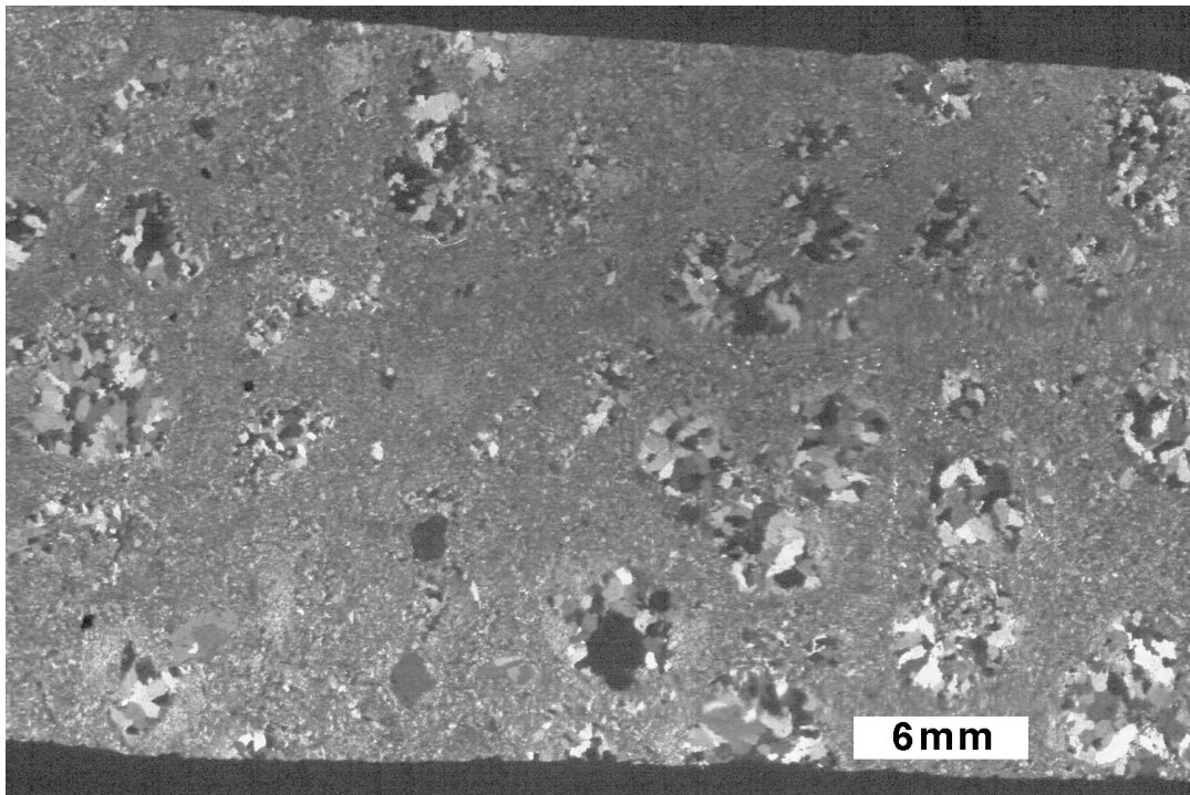
Figure 4.11. Uwharries Southeastern sample with circular quartz amygdules and sparse phenocrysts (FBL025; scanned thin section, crossed polars).
