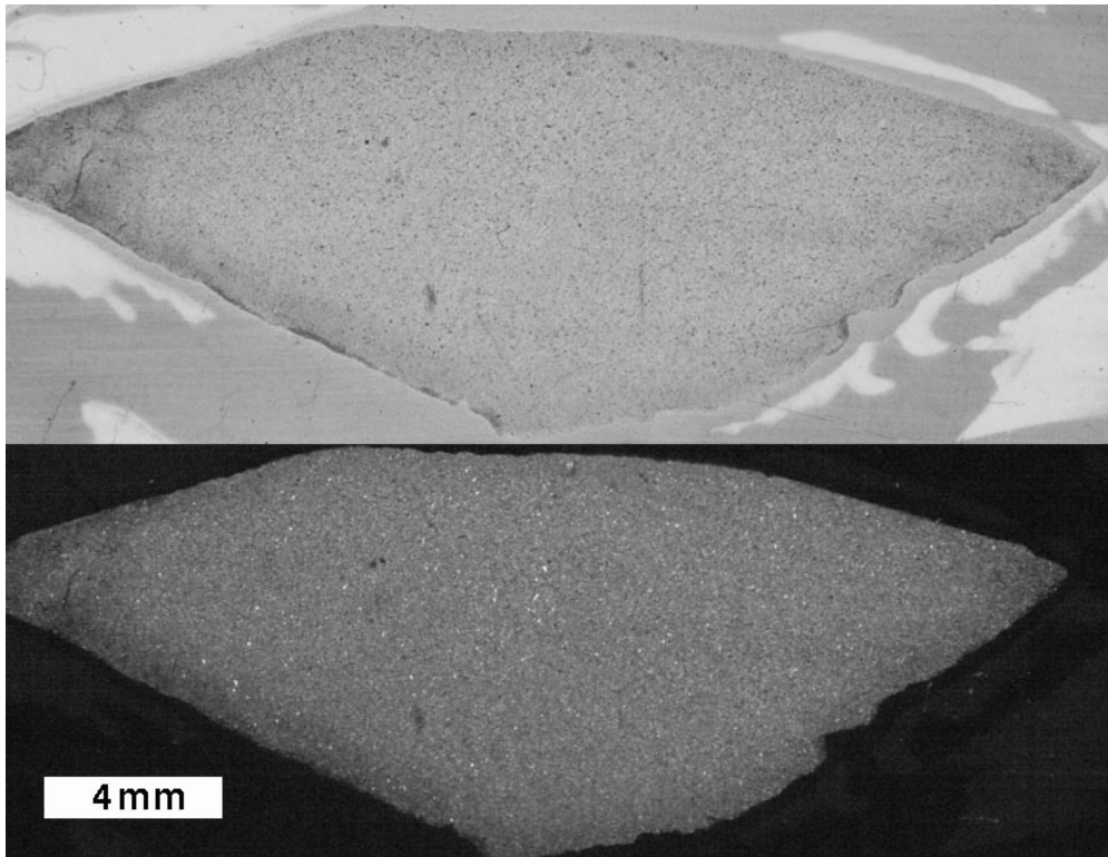
Figure 4.26. Artifact FBL076 (scanned thin section, plane-polarized light [top] and crossed polars [bottom]).
