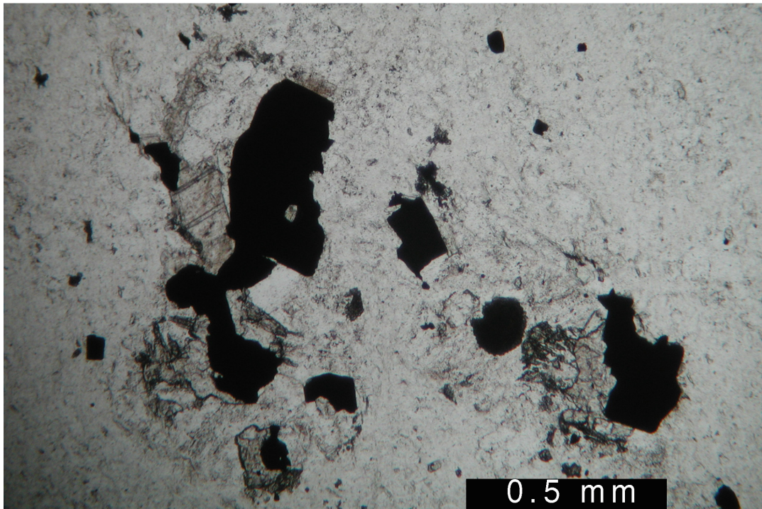
Figure 4.8. Uwharries Asheboro sample with mineral clusters of pyrite + calcite + epidote (FBL021; plane-polarized light).
