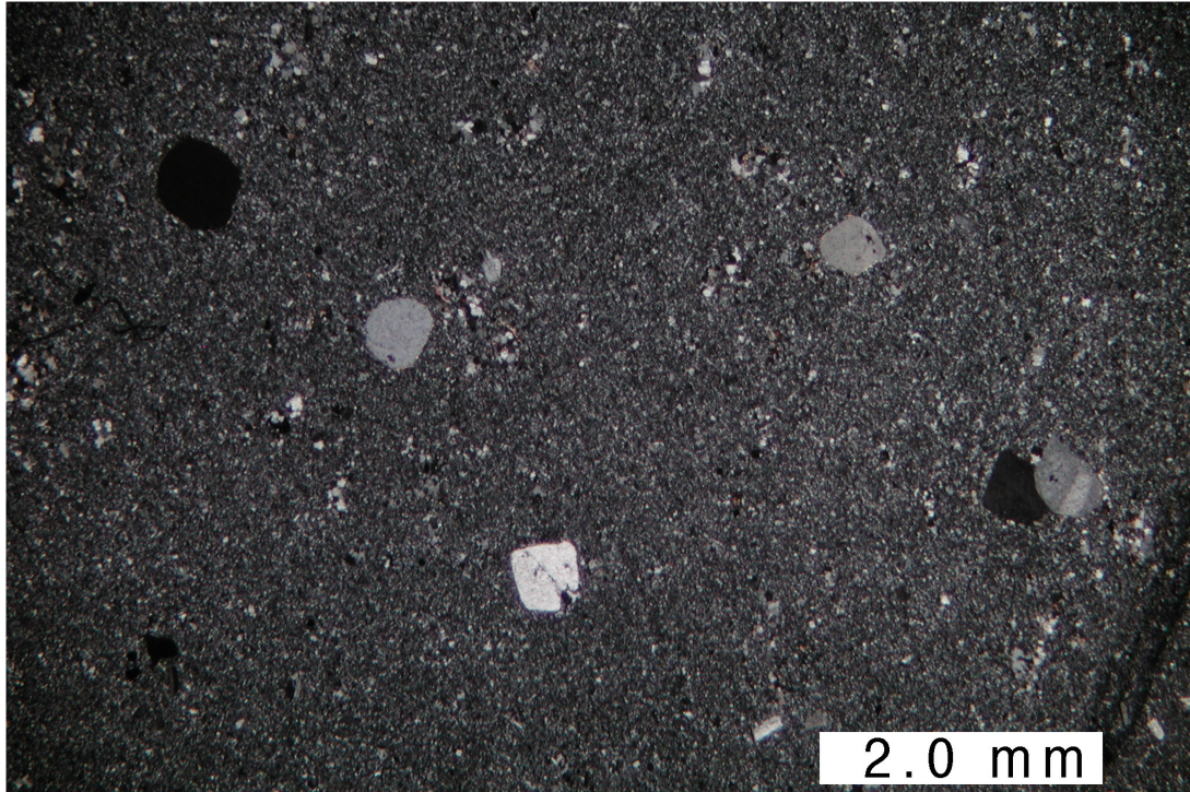
Figure 4.3. Typical Uwharries Eastern sample with quartz and plagioclase phenocrysts (FBL004; crossed polars).
