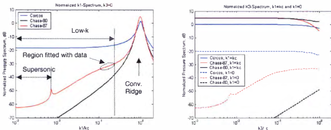
Figure 4. Normalized Corcos's, Chase-1980 and Chase-1987 Spectra Displayed as Logarithmic Spectra as a Function of Logarithmic Wavenumbers in k_1 and k_3 .
