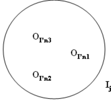
Figure 4: Multi-Resolution Space
