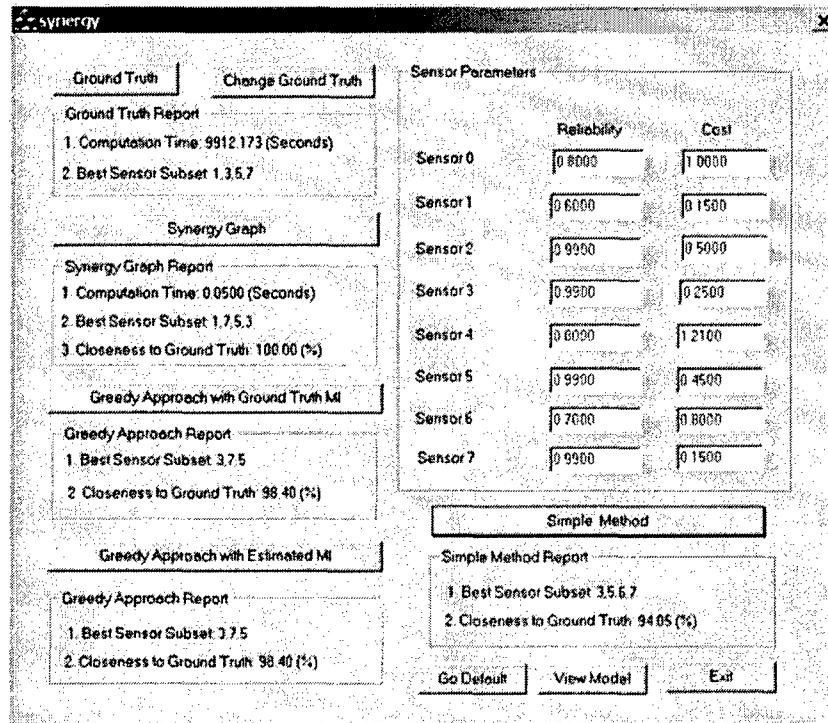
Figure 12: The active fusion demo software interface that uses mutual information as sensor selection criterion and uses the graph-theoretic approach for sensor selection.
