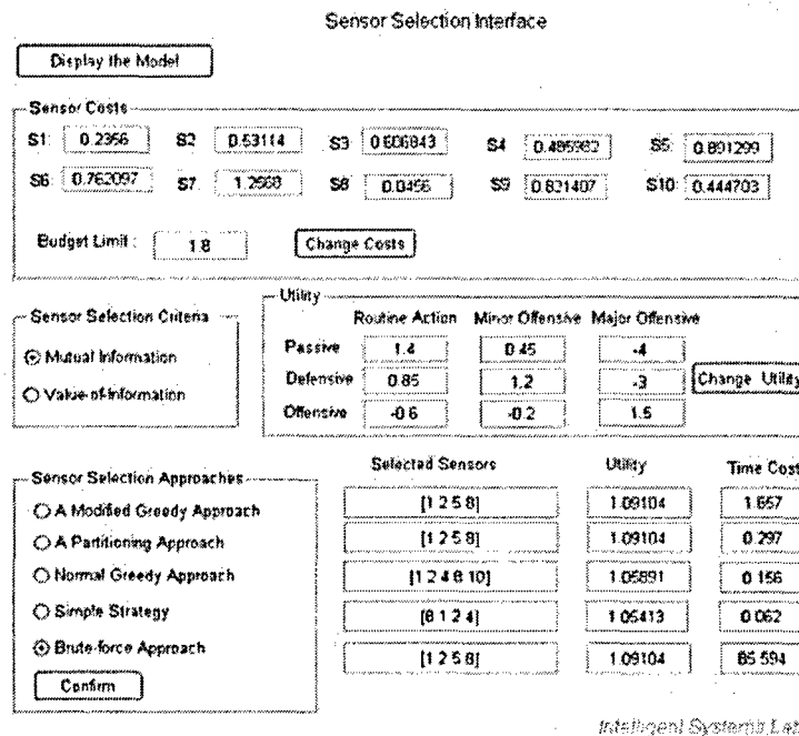
Figure 13: The active fusion demo software interface that uses either mutual information or value of information as sensor selection criteria and uses the greedy approach for sensor selection.
