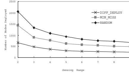
Fig. 9. Performance of DIFF_DEPLOY, MIN_MISS and RANDOM with various sensing ranges for differentiated detection requirements.
