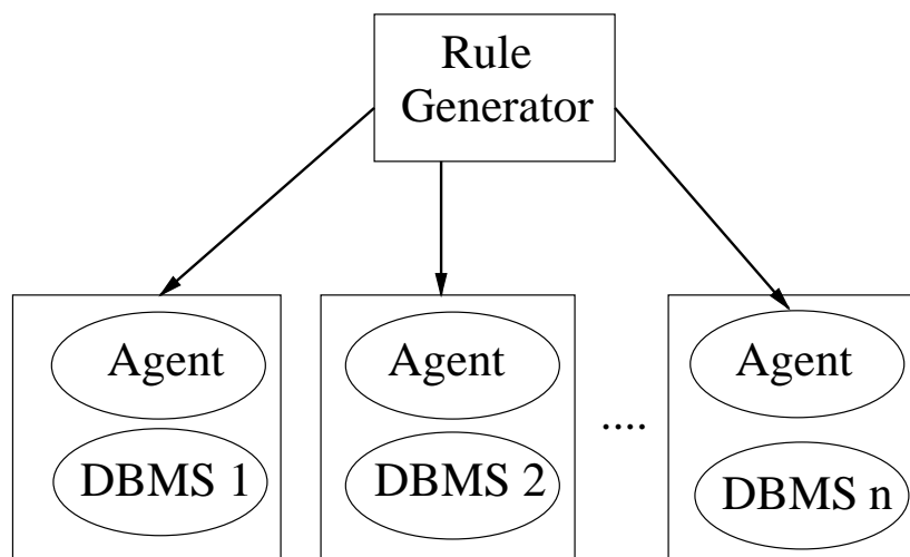
Fig. 3. Architecture of Agent-based Rational Downgrader
