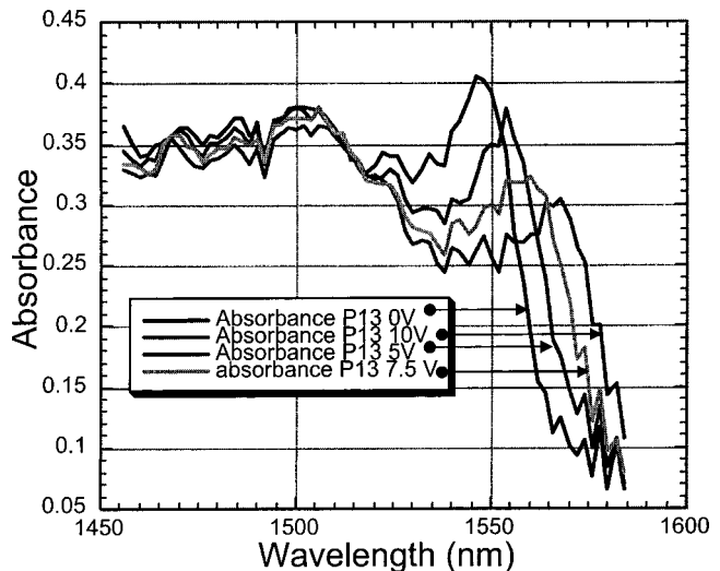
Fig. 10 Absorbance versus wavelength for 1550-nm devices. First efforts are yielding MQW modulators that have 2.3:1 contrast ratios.
