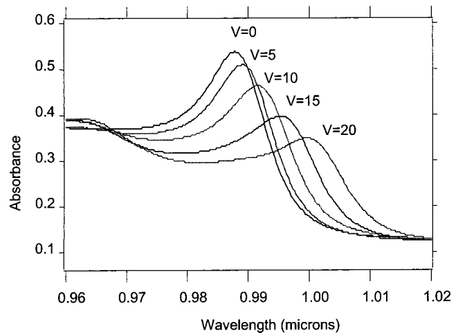
Fig. 2 Switching characteristic of an InGaAs-based MQW modulator.
