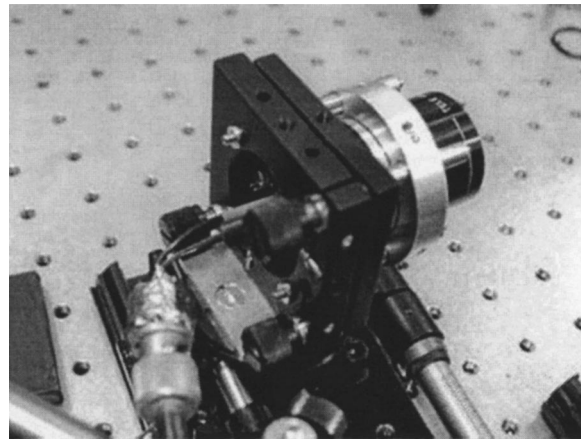
Fig. 13 Photo of a first “cat’s eye” retroreflector. This device supports of the order of 40 Mbps and is about 10 times the diffraction limit.
