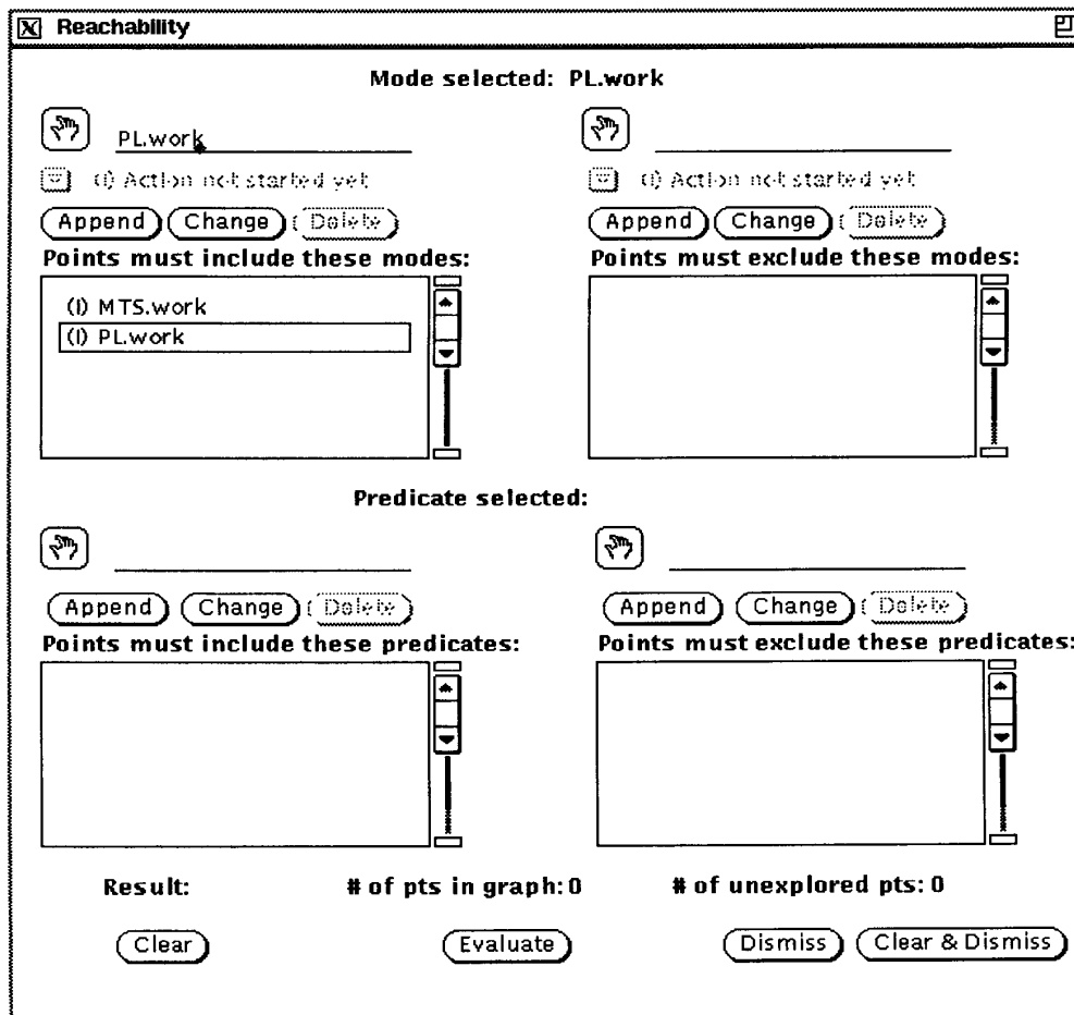
FIGURE 9. The MT verifier's reachability query. The four components are for specifying, respectively, a list of active modes, a list of inactive modes, a list of true predicates, and a list of false predicates. The query returns the number of points in the computation matching the parameters. Objects not mentioned in the lists assume a "don't care" status in the query.
