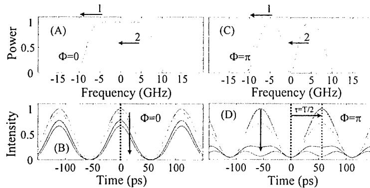
Fig. 4 Fit to Fig. 2 using the frequency-domain model. (A, C) Spectra fit (linear scale) for \delta\epsilon of {0, 7, 14, 21, 28, 35, 42 and 49}%. The arrows indicate the initial line positions and the direction of detuning. Experimental time-domain traces for corresponding frequency offsets are shown for \Phi=0 (B) and \Phi=\pi (D). The arrows indicate intensity peak variations associated with these frequency offsets. Delay positions are marked by dashed lines. (Video file of 0.97 Mb for \Phi=0 and 1.00 Mb for \Phi=\pi .)
