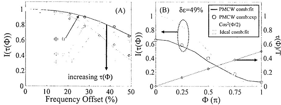
Fig. 6 (A) Experimental (symbols: \Phi = \{0, \pi/4, \pi/2, 3\pi/4 \text{ and } \pi\} ) and calculated (lines: \Phi = 0 to \pi in \pi/4 increments) waveform amplitudes at corresponding \tau(\Phi) for \delta\varepsilon of \{0, 7, 14, 21, 28, 35, 42 \text{ and } 49\}\% . (B) Intensity values for 49% frequency offset at corresponding \tau(\Phi) for different \Phi values using phase-modulated CW comb (blue circle: experimental; blue solid line: calculation). Calculated (dotted line) and experimental (diamonds) \tau(\Phi) is also included. Intensity values assuming ideal comb lines (red square) is plotted with \cos^2(\Phi/2) (red dashed line).
