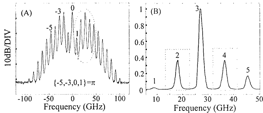
Fig. 8 (A) Spectrum obtained from a low V_{\pi} phase modulator. Circled spectral portion is expanded in (B), in linear scale and normalized to line {3}. Lines {2, 4} are selected by the line-by-line shaper while the others are suppressed.
