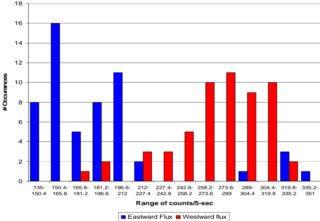
Figure 3.1: Histogram of >25MeV proton counts in the -30° Lat, 315° Long, 1000km Alt bin separated by Eastward and Westward fluxes
