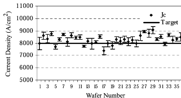
Fig. 3. Trend chart of current density ( J_c ). Mean = 8.3 ± 0.37 kA/cm 2 or ±4.4% ( 1\sigma ). Target specification = 8.0 kA/cm 2 ± 10% ( 1\sigma ).
