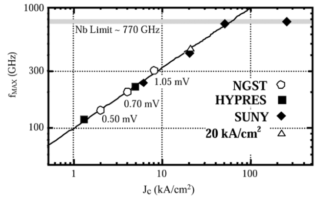
Fig. 14. Maximum reported TFF divider speed f_{MAX} versus J_c for trilayers from HYPRES, NGST, and SUNY. The numbers adjacent to the NGST points indicate the optimum I_c R_N product of the shunted junctions used in the TFF. Also, shown is the projected divider speed of \sim 450 GHz for the next-generation 20-kA/cm 2 process.
