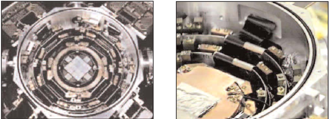
Figure 6. A prototype cryo enclosure for operation at 4 K (Ref: NGST).
