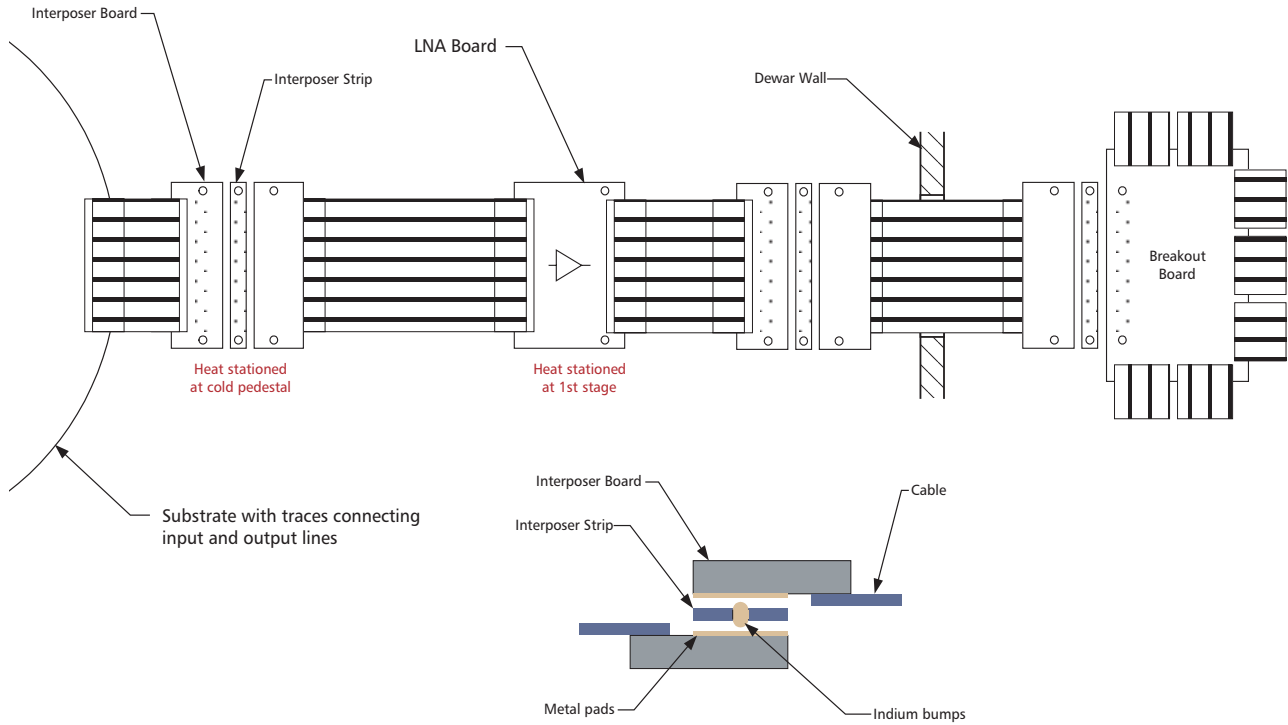
Figure 6-7. A high-speed flexible ribbon cable designed for modular attachment (Ref: NGST).
