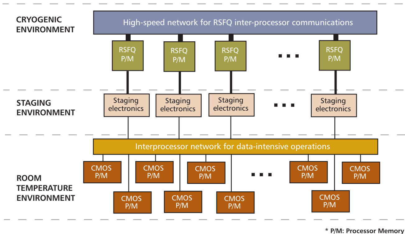
Figure 1-3. Conceptual architecture.
