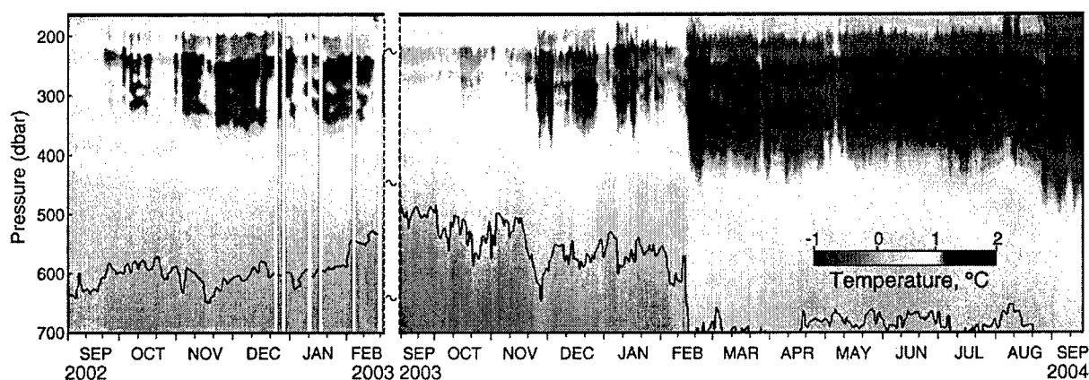
Fig. 3. Water temperature from the MMP profiler. The 0°C isotherm (black line) traces the lower boundary of the AW layer. Blank areas represent missing data. 10-m vertical binning is used.
