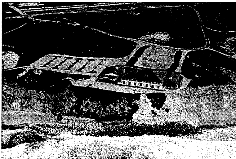
Fig. 2. Aerial oblique photo of Stillwell Hall, Fort Ord, California showing rock-rubble sea wall in front and extensive erosion to each side (from USGS 1998).
