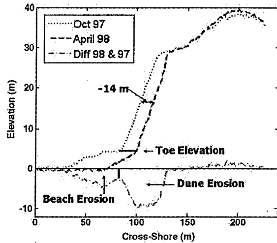
Fig. 5. Cross-shore profiles from LIDAR for 1997 and 1998. The beach and dune erosion are the differences of profile areas and are partitioned at the toe.
