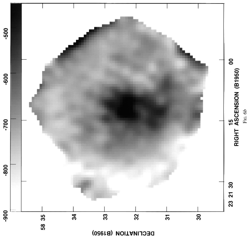
FIG. 6.—Contour (a) and gray-scale (b) spectral index maps of the SNR Cas A between 74 and 333 MHz. The peak value of the map is -1.08 , and for (a) the contours are at (-18, -17, -16, -15, -14, -13, -12, -11, -10, -9, -8) times 0.05 in units of spectral index ( S \propto \nu^{-\alpha} ). This image was made from the images shown in Figs. 2 and 3 above. For (b) the gray-scale range in spectral index is from -900 to -450 in units of spectral index times 10^{-3} , as indicated by the scale at the top of the image.
