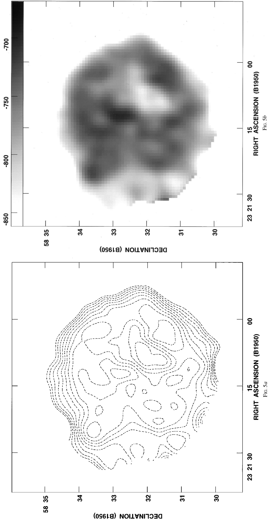
FIG. 5.—Contour (a) and gray-scale (b) spectral index maps of the SNR Cas A between 333 and 1381 MHz. The peak value of the map is -1.146 , and the contours are at (-9, -8.8, -8.6, -8.4, -8.2, -8, -7.8, -7.6, -7.4, -7.2, -7, -6.8, -6.6, -6.4) times 0.1 in units of spectral index ( S \propto \nu^{-\alpha} ). This image was made from the images shown in Figs. 3 and 4 above. For (b) the gray-scale range in spectral index is from -860 to -670 in units of spectral index times 10^{-3} , as indicated by the scale at the top of the image.
