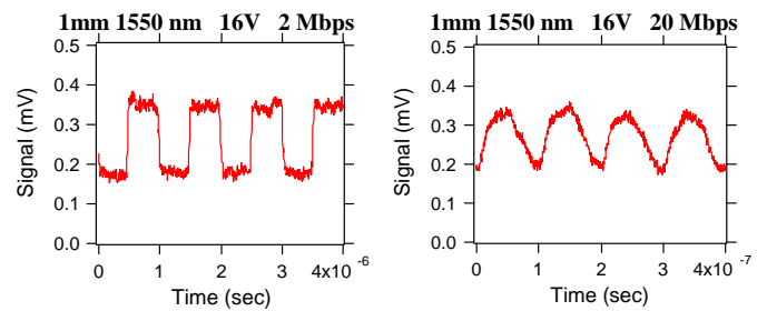
FIGURE 10. Modulation traces are shown for the 1550 MQW devices. The one millimeter diameter devices are shown to support at least 20 Mbps.
