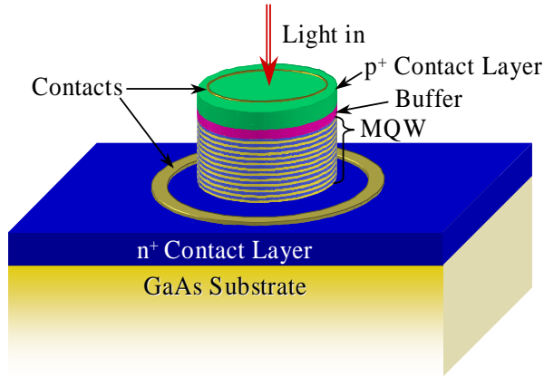
FIGURE 1. Schematic of the MQW modulator geometry showing layer structure and electrical contacts for a surface normal optically transmissive device.[3]
