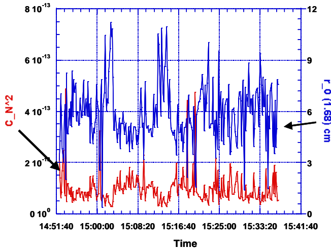
FIGURE 7. Traces of the structure constant, C_n^2 , as a function of time during the data-in-flight measurements. Instantaneous values varied significantly but the average value was on the order of 4E(-14) .
