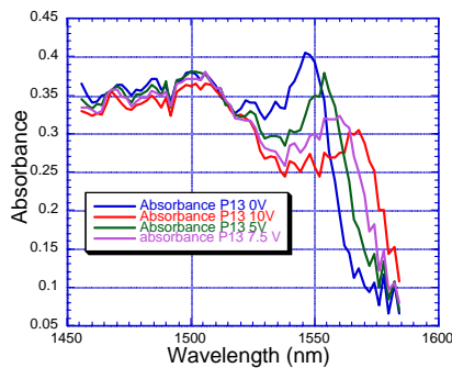
FIGURE 9. Absorbance vs. wavelength for 1550 nm devices. First efforts are yielding MQW modulators that have 2.3:1 contrast ratios.
