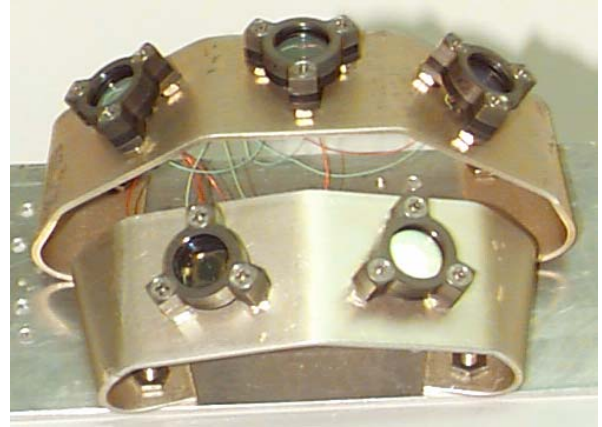
FIGURE 3. Retromodulator Array for UAV Data-in-Flight; MRR units have a 980 nm center frequency; devices populate the array with a 30 degree separation with retros about 5 cm apart which present a 60 degree Field-of-View.
