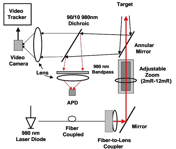
FIGURE 4. Block diagram of Transmit/Receive system for UAV Data-in-Flight; Aperture-sharing is accomplished with an annular mirror; zoom optics enable in-situ changes in divergence; in-line acquisition and tracking is enabled by chromatic aperture-sharing.
