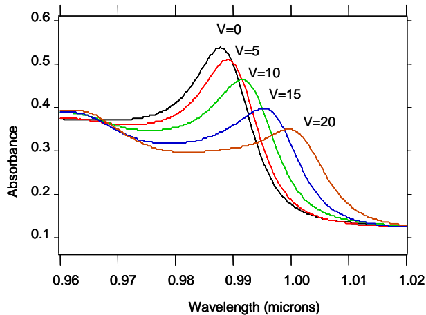
FIGURE 2: Switching characteristic of an InGaAs-Based MQW modulator.
