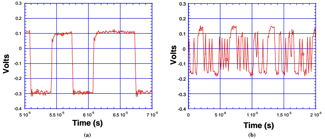
FIGURE 5. Traces of data-in-flight at ranges from about 30m to 50 m. Data streams varied continuously through (a) 300 kbps and (b) 5 Mbps. Data was obtained without bit drop out in daylight outside at ranges up to 100 meters.
