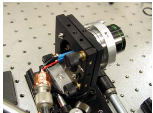
FIGURE 12. A photo of a first "Cat's Eye" retromodulator is shown. This device supports on the order of 40 Mbps and is about 10 times the diffraction limit.
