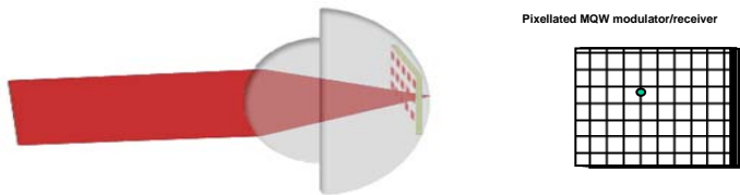
FIGURE 11. The concept of a focal plane "Cat's Eye" retromodulator is shown.
