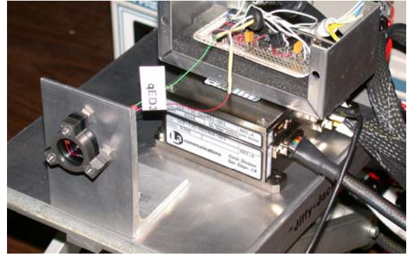
FIGURE 8. A photograph of the communications terminal is shown. The unit was comprised of a 980 nm retromodulator coupled to an L3 wavelet compression unit, impedance-matching drive circuitry and power supply. The link was obtained with 130 mW on the modulator supporting up to 6 Mbps, 30 fps.
