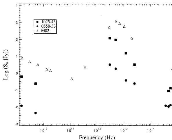
FIG. 3. Spectral energy distributions for two galaxies from the interacting sample plotted along with that of M82, a starbursting galaxy. The downward pointing arrow indicates an upper limit only for the 12 \mu\text{m} passband. Optical data for 0558-33 and 1025-43 and from Smith & Hintzen (1991). Infrared data are from the IRAS Point Source Catalog.
